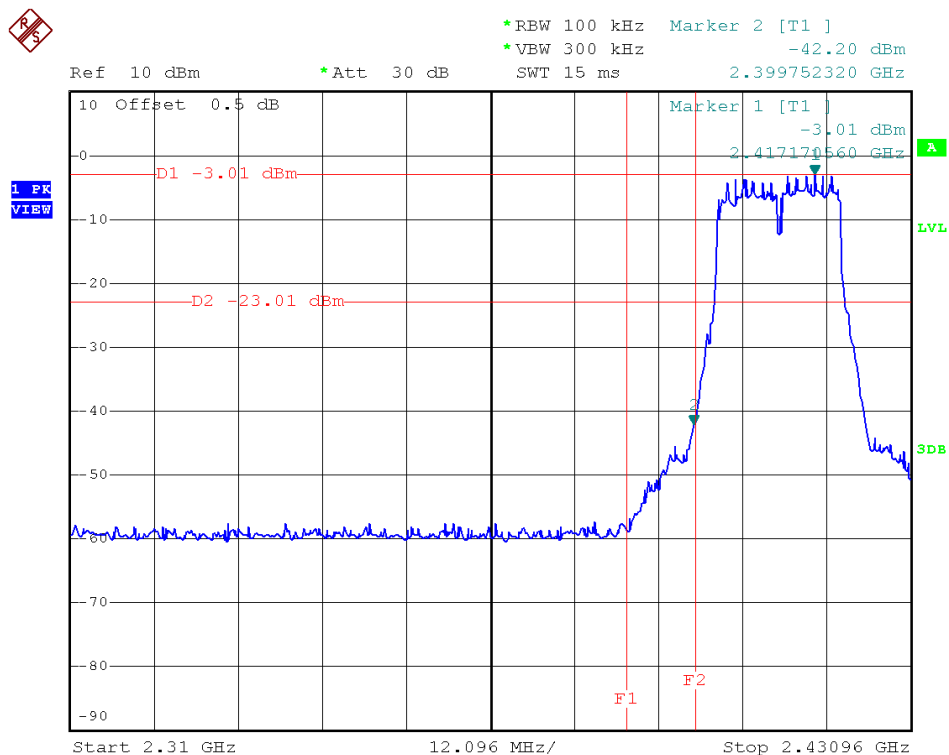
(Plot 2.6 C1: Channel = 1 @ 802.11n-20)
