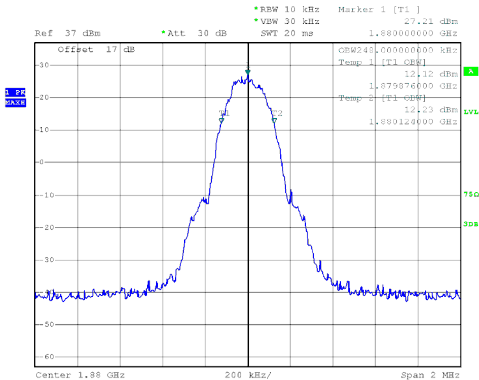
(Plot F4: EDGE 1900MHz Channel = 661)
