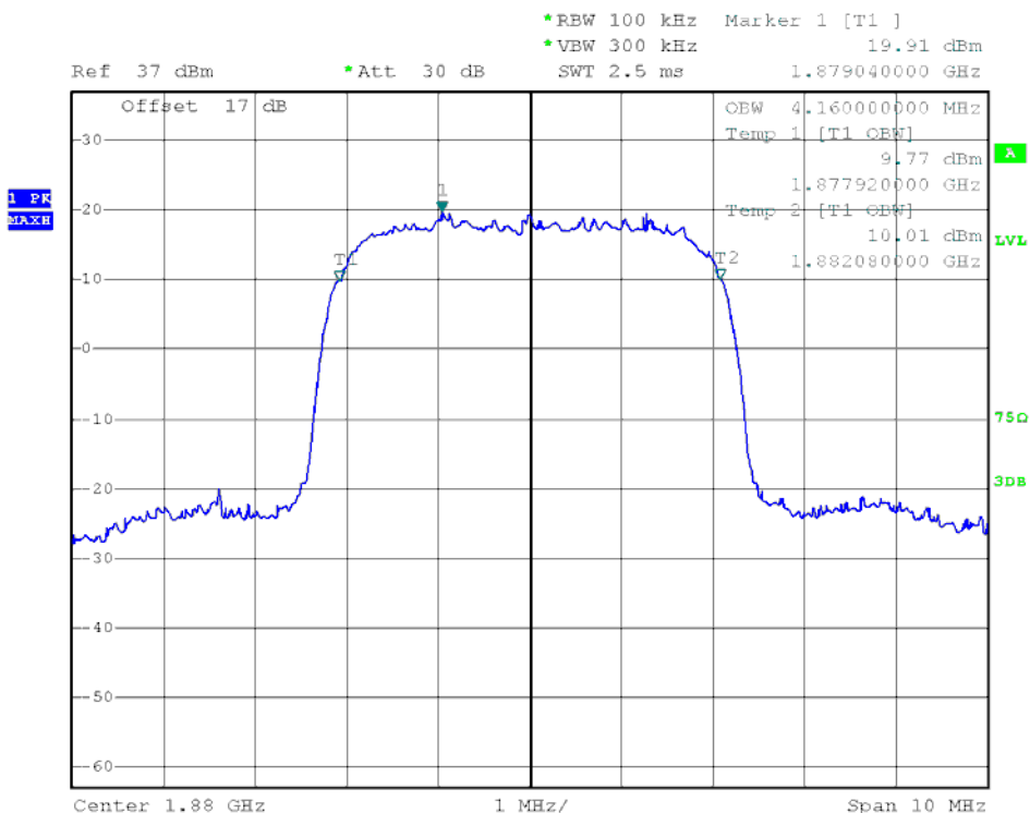
(Plot H4: WCDMA 1900 MHz Channel = 9400)
