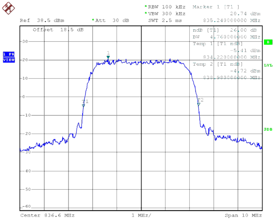
(Plot M3: HSPA+ 850 MHz Channel = 4183)
