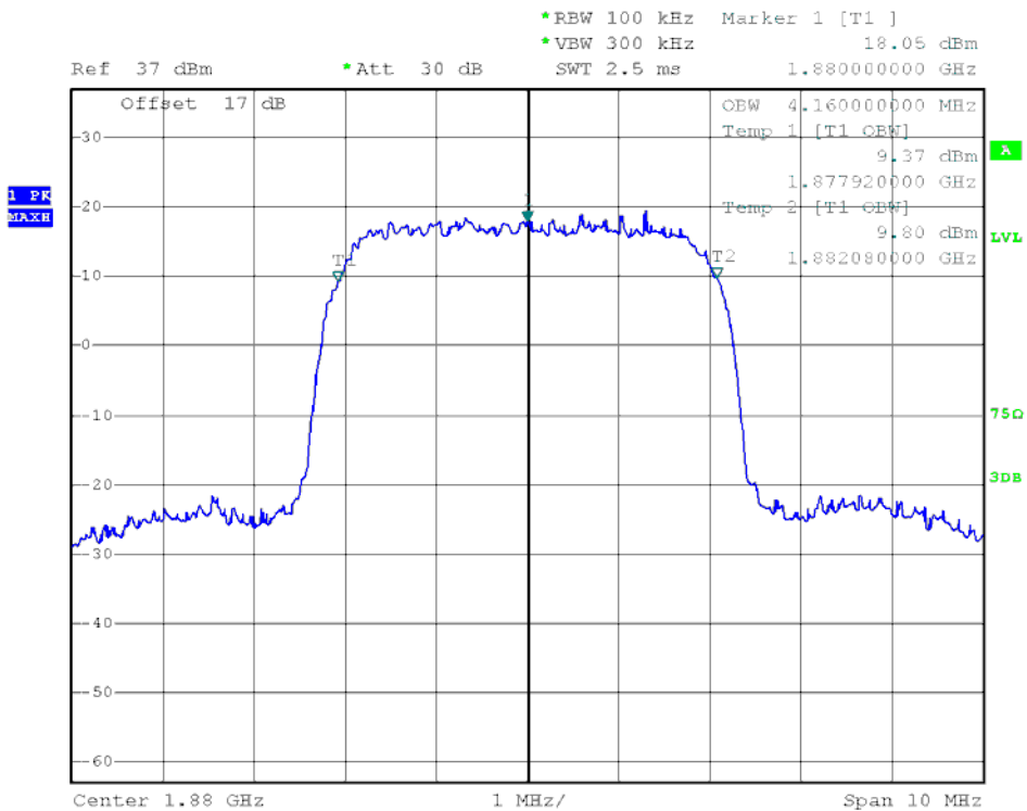
(Plot J4: HSDPA 1900 MHz Channel = 9400)
