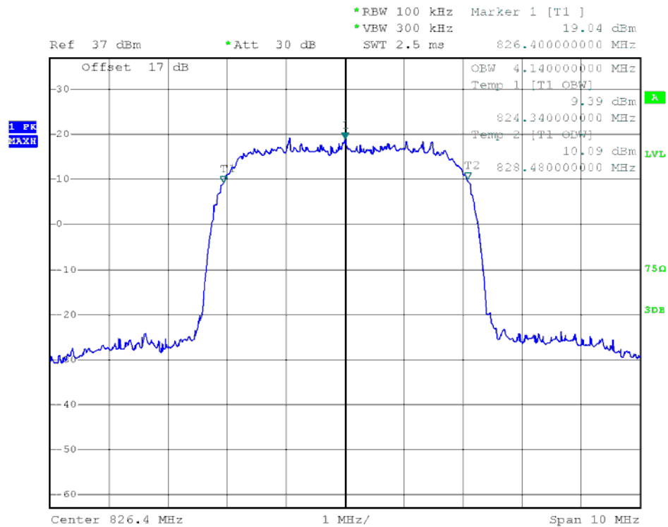
(Plot I2: HSDPA 850MHz Channel = 4132)
