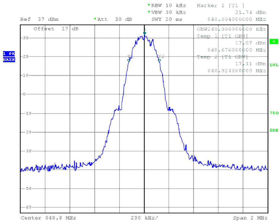
(Plot E6: EDGE 850MHz Channel = 251)
