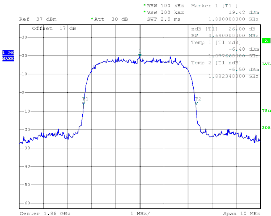
(Plot H3: WCDMA 1900 MHz Channel = 9400)
