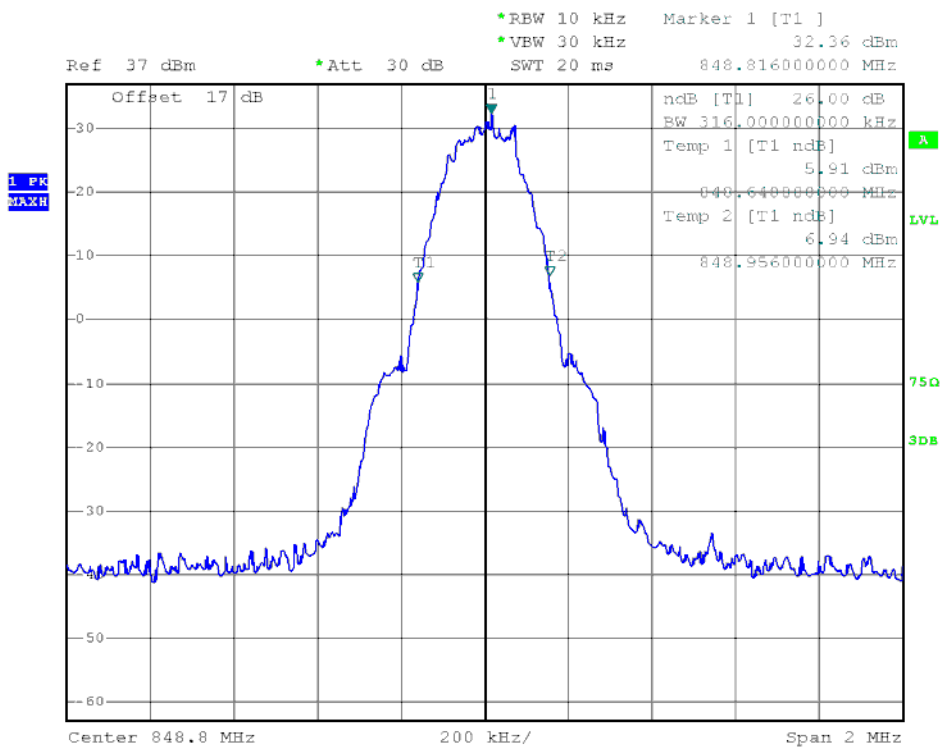
(Plot E5: EDGE 850MHz Channel = 251)
