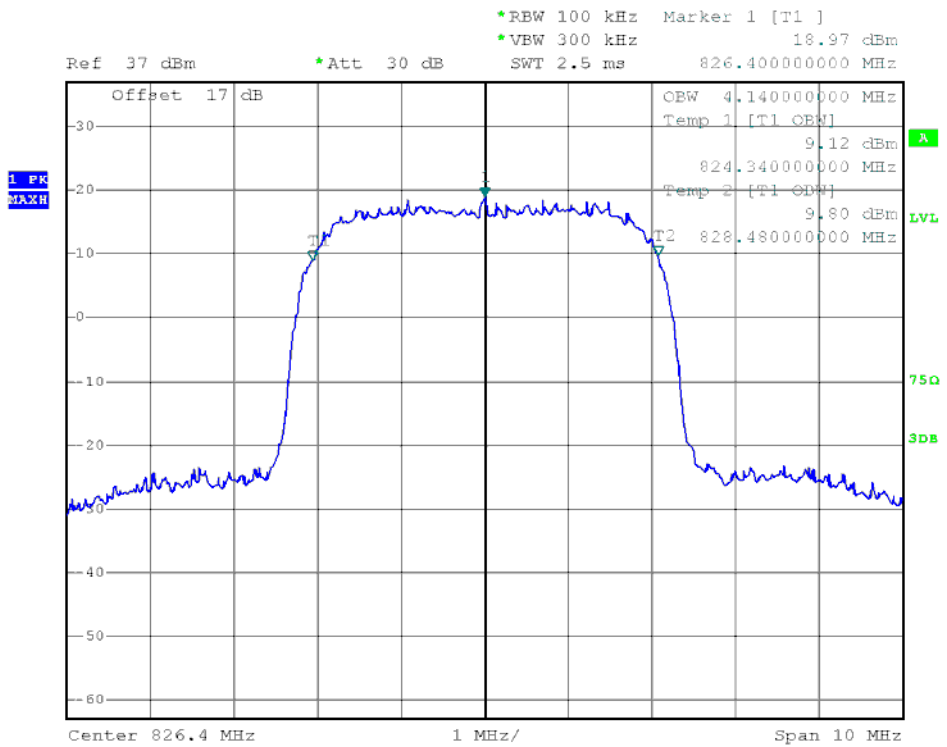
(Plot K2: HSUPA 850MHz Channel = 4132)
