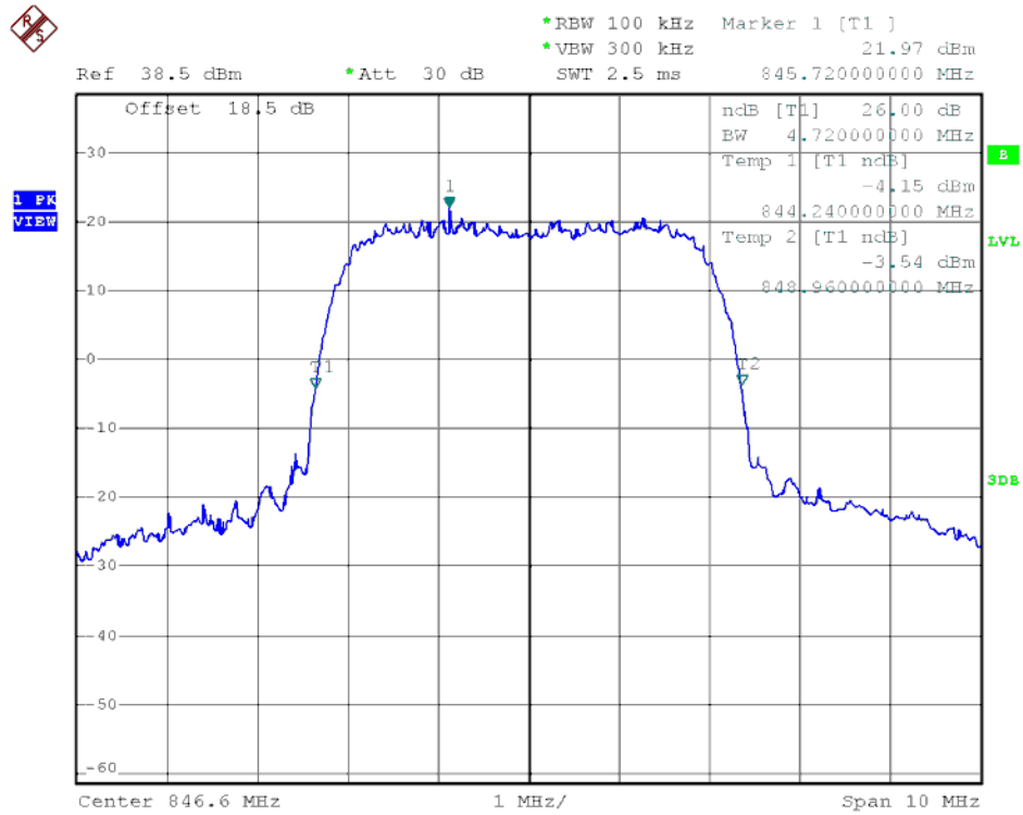
(Plot M5: HSPA+ 850MHz Channel = 4233)
