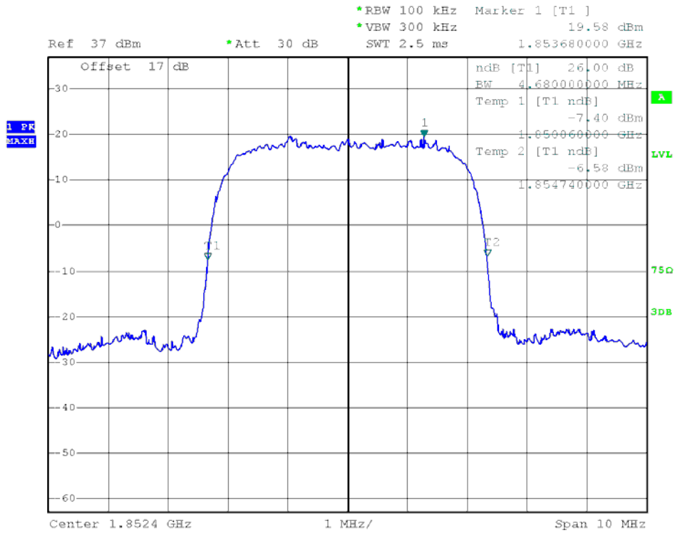
(Plot H1: WCDMA 1900MHz Channel = 9262)
