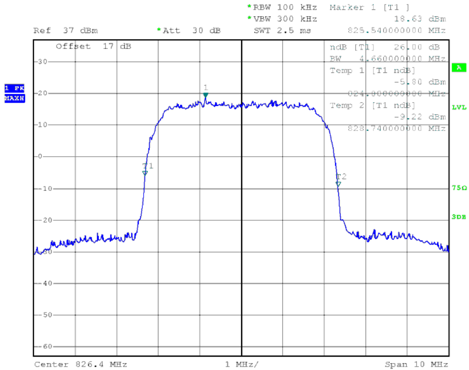
(Plot I1: HSDPA 850MHz Channel = 4132)
