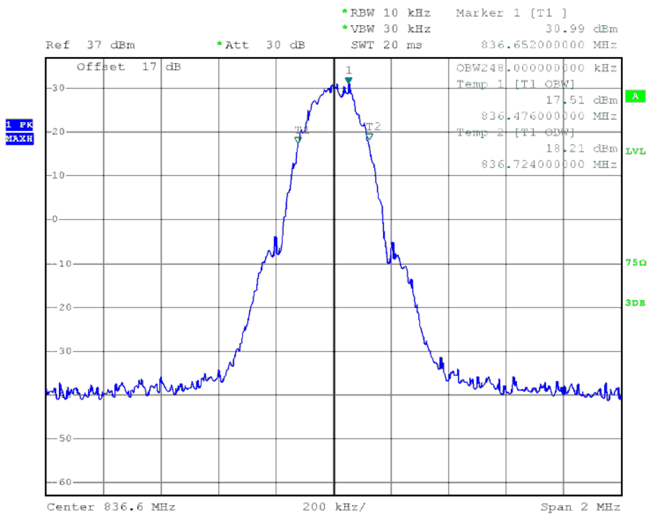
(Plot E4: EDGE 850MHz Channel = 190)
