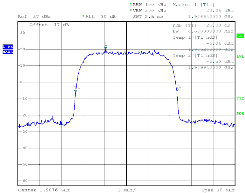
(Plot H5: WCDMA1900MHz Channel = 9538)
