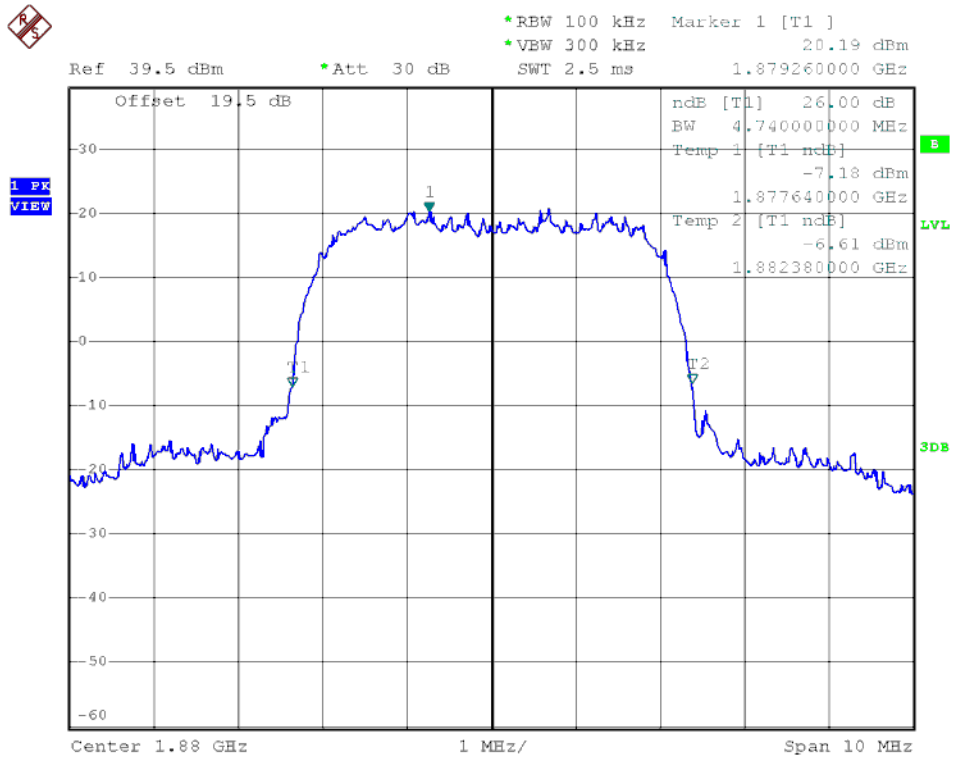
(Plot N3: HSPA+ 1900 MHz Channel = 9400)
