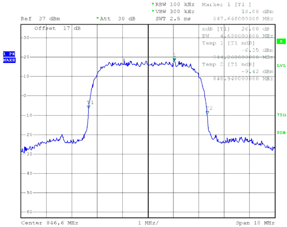
(Plot K5: HSUPA 850MHz Channel = 4233)
