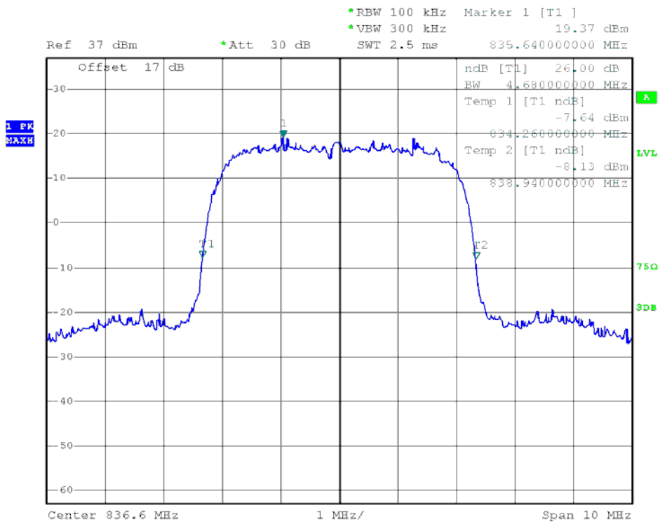
(Plot G3: WCDMA 850 MHz Channel = 4183)
