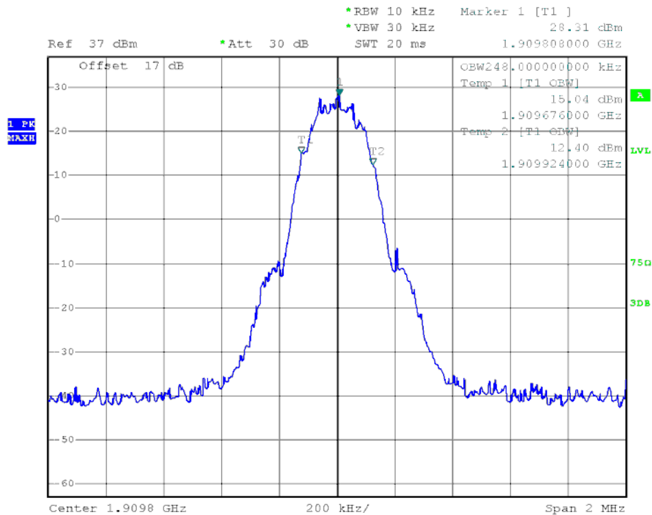
(Plot D6: GPRS 1900MHz Channel = 810)
