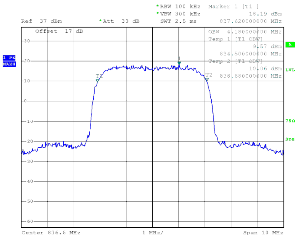
(Plot I4: HSDPA 850 MHz Channel = 4183)
