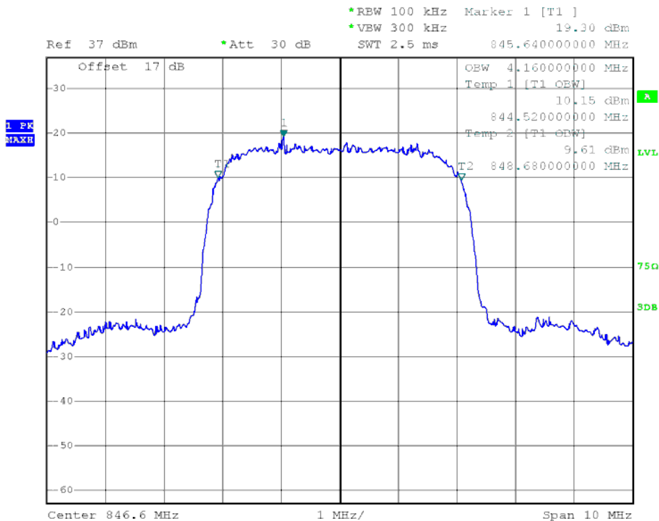
(Plot I6: HSDPA 850MHz Channel = 4233)
