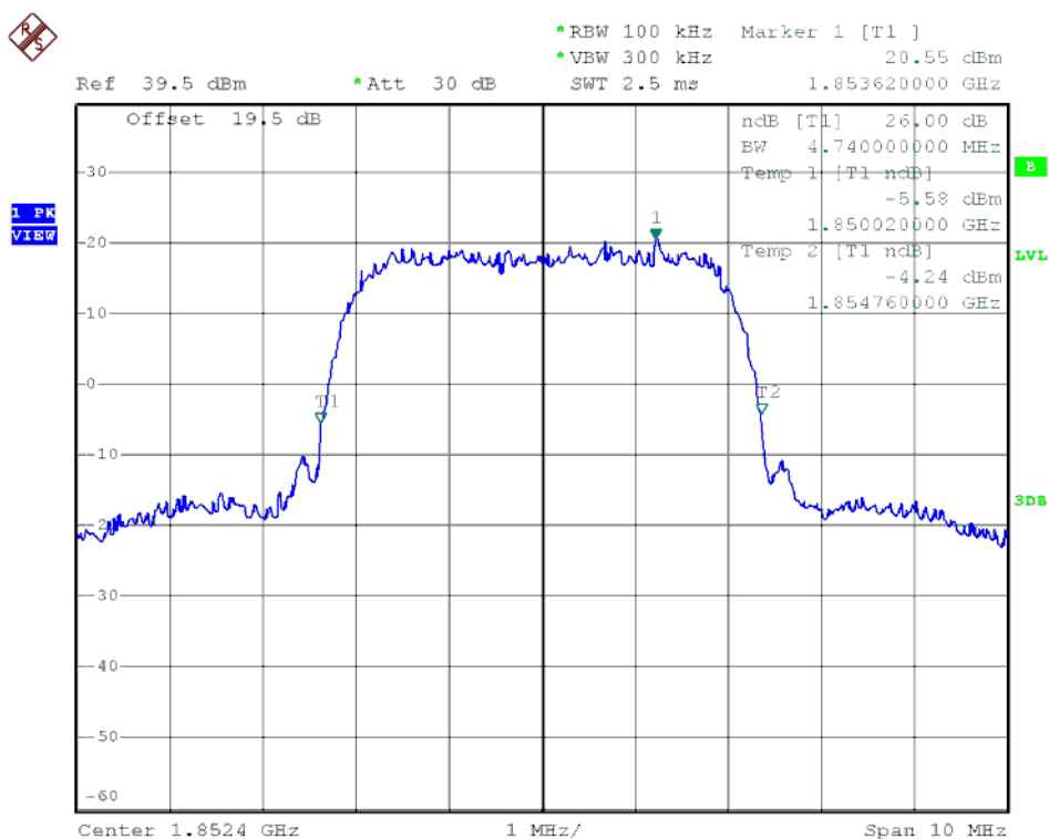
(Plot N1: HSPA+ 1900MHz Channel = 9262)
