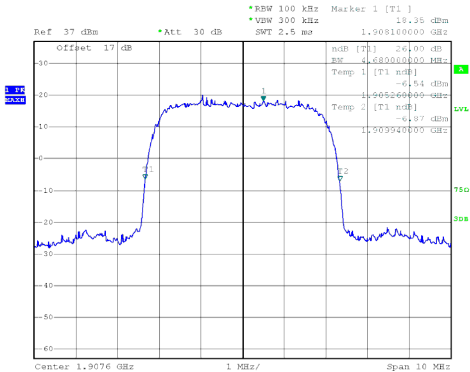
(Plot J5: HSDPA 1900MHz Channel = 9538)
