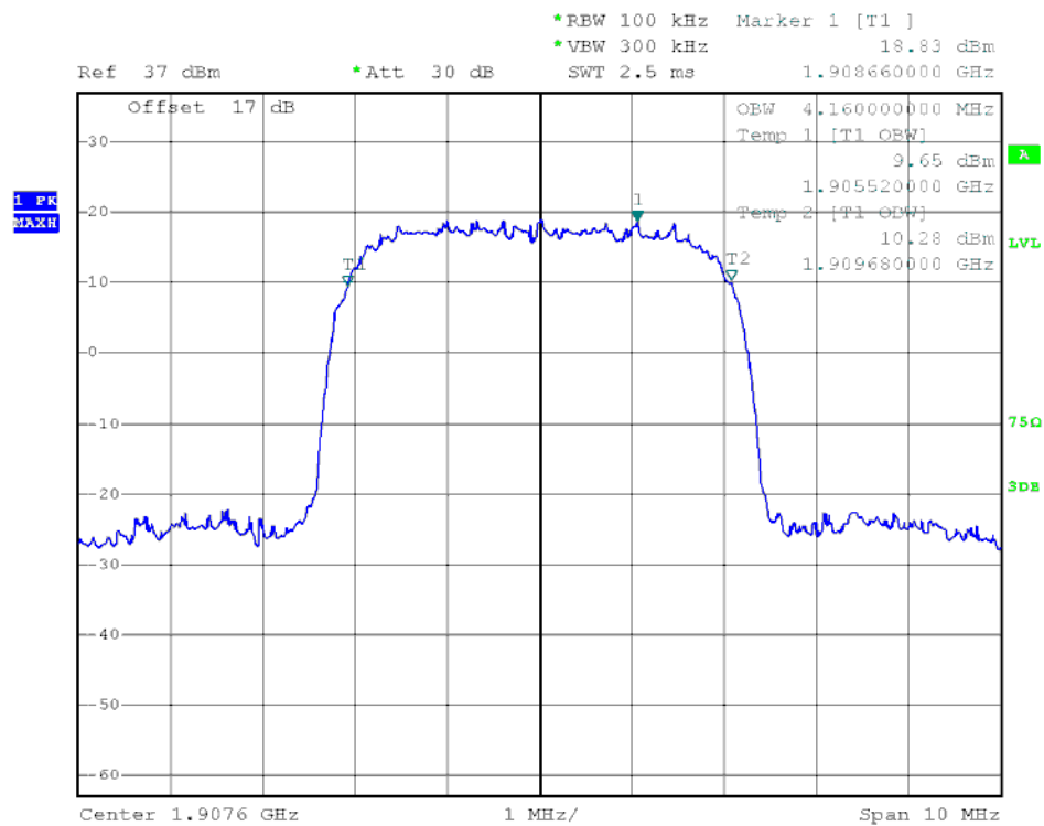
(Plot J6: HSDPA 1900MHz Channel = 9538)
