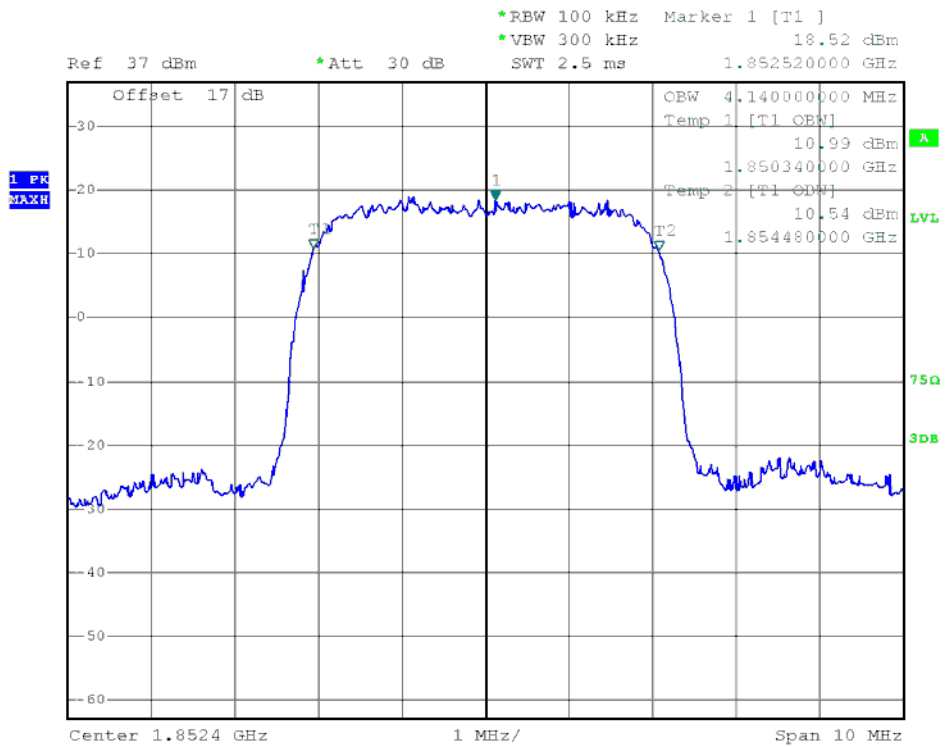
(Plot H2: WCDMA 1900MHz Channel = 9262)
