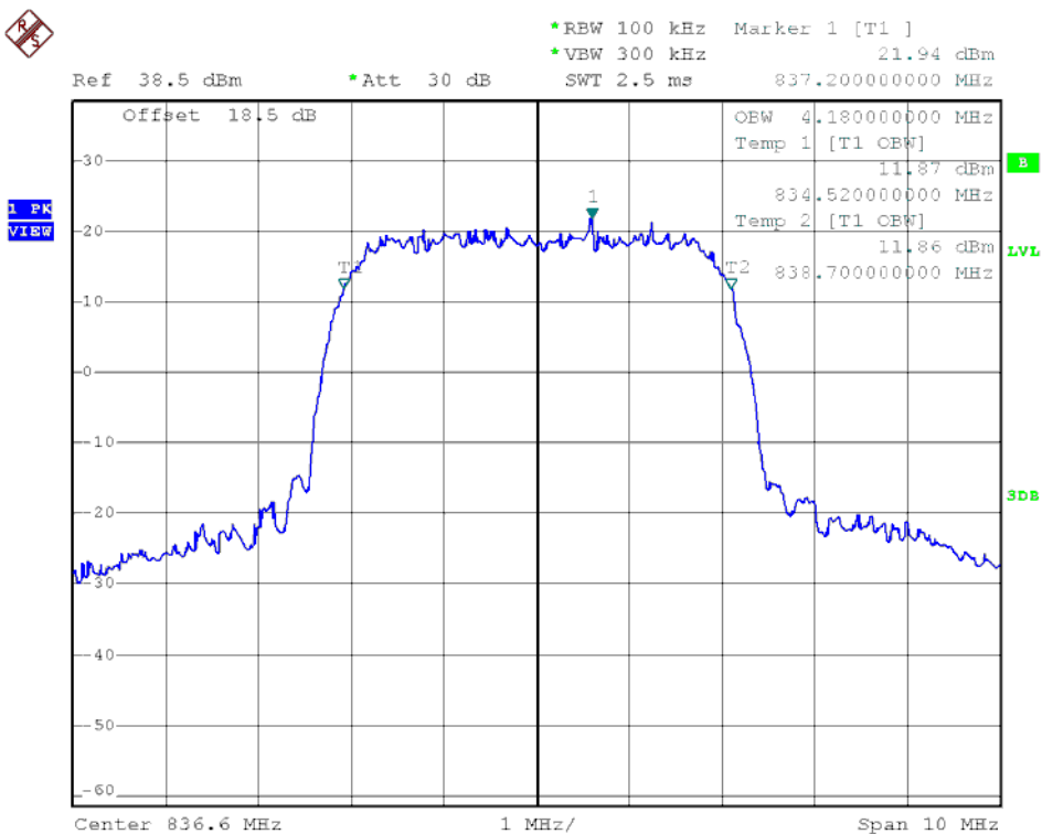
(Plot M4: HSPA+ 850 MHz Channel = 4183)
