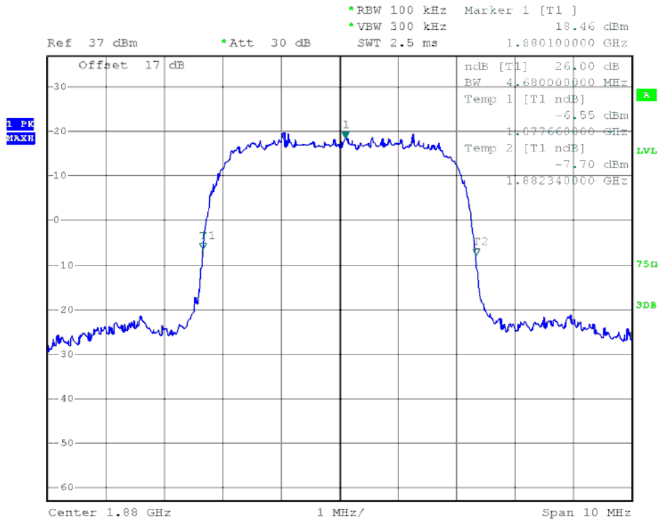
(Plot L3: HSUPA 1900 MHz Channel = 9400)
