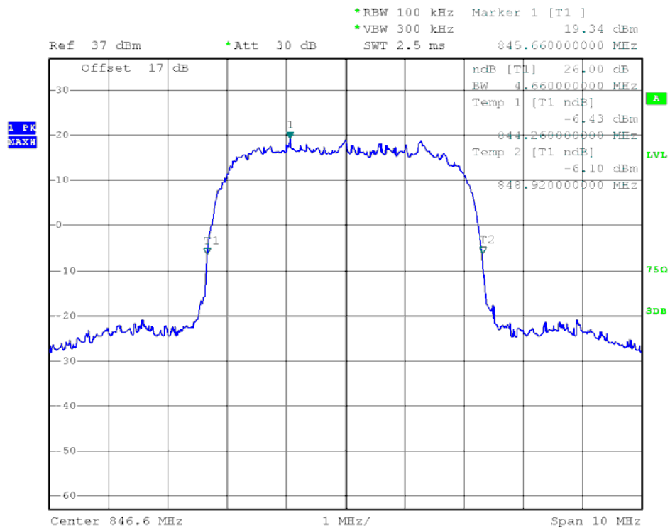
(Plot I5: HSDPA 850MHz Channel = 4233)
