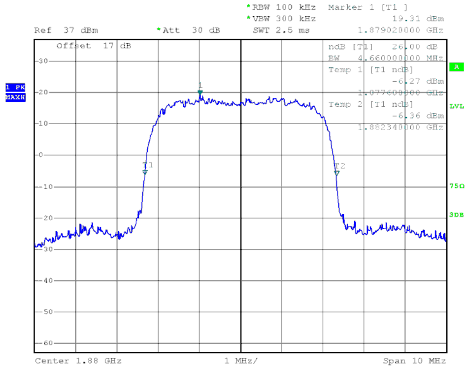
(Plot J3: HSDPA 1900 MHz Channel = 9400)
