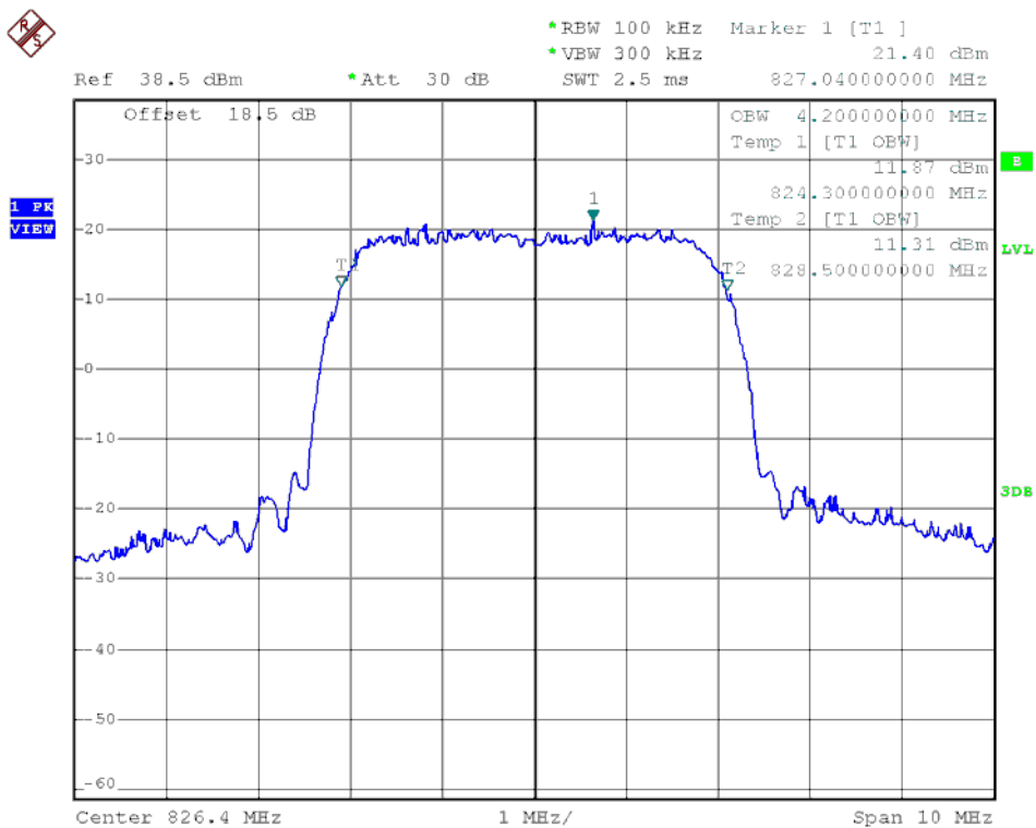
(Plot M2: HSPA+ 850MHz Channel = 4132)
