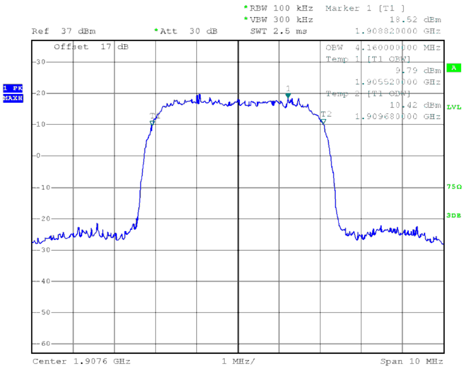
(Plot L6: HSUPA 1900MHz Channel = 9538)
