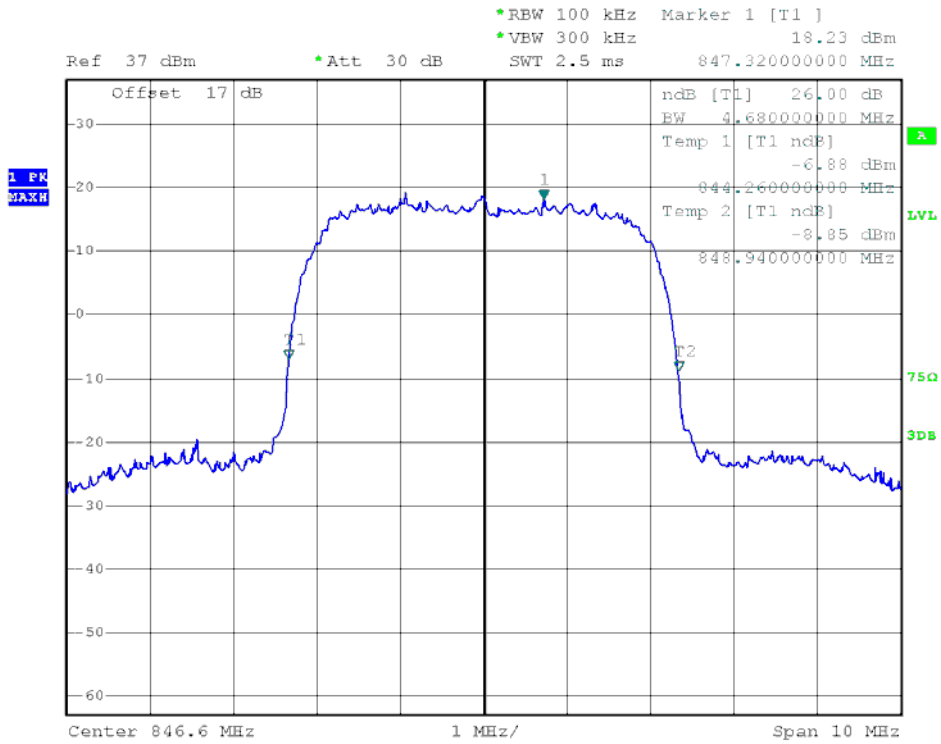
(Plot G5: WCDMA 850MHz Channel = 4233)
