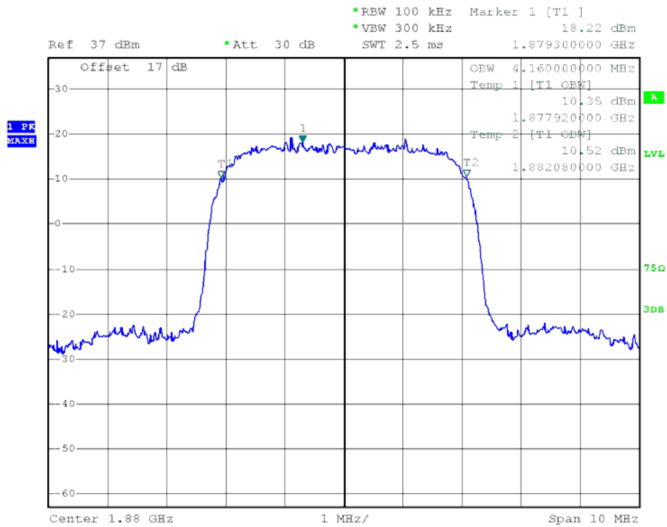
(Plot L4: HSUPA 1900 MHz Channel = 9400)
