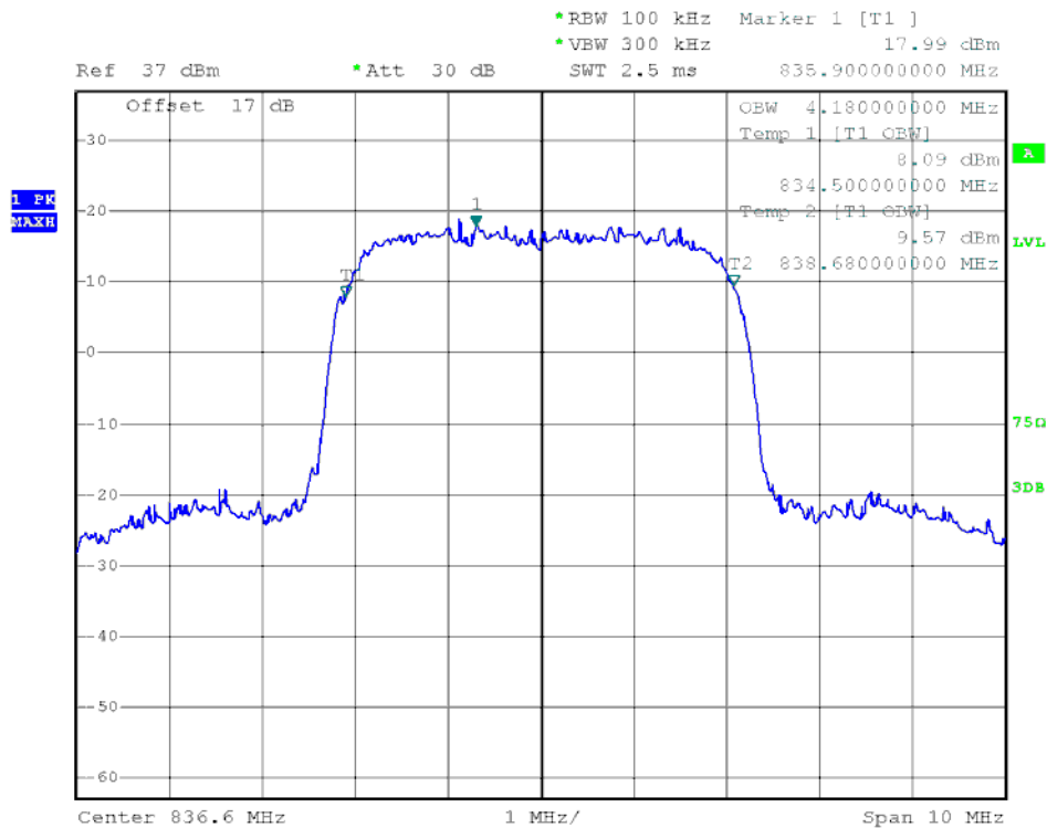
(Plot K4: HSUPA 850 MHz Channel = 4183)
