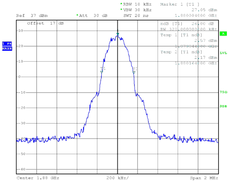
(Plot F3: EDGE 1900MHz Channel = 661)
