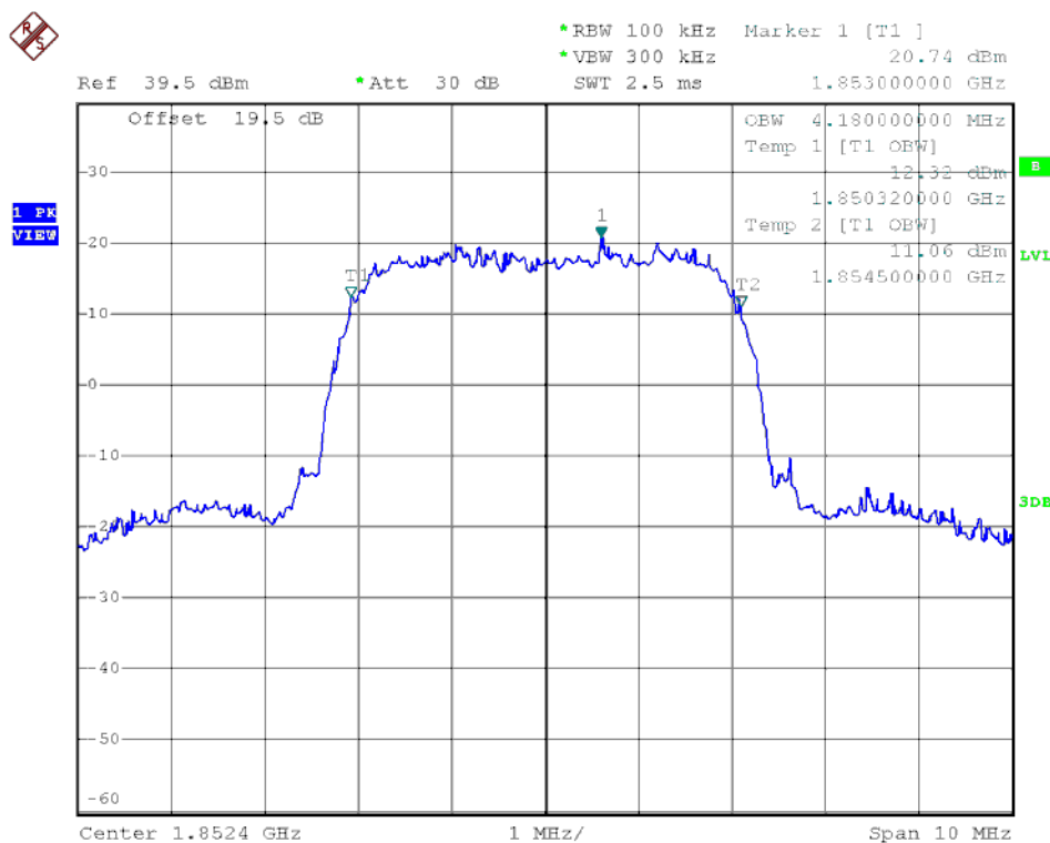
(Plot N2: HSPA+ 1900MHz Channel = 9262)
