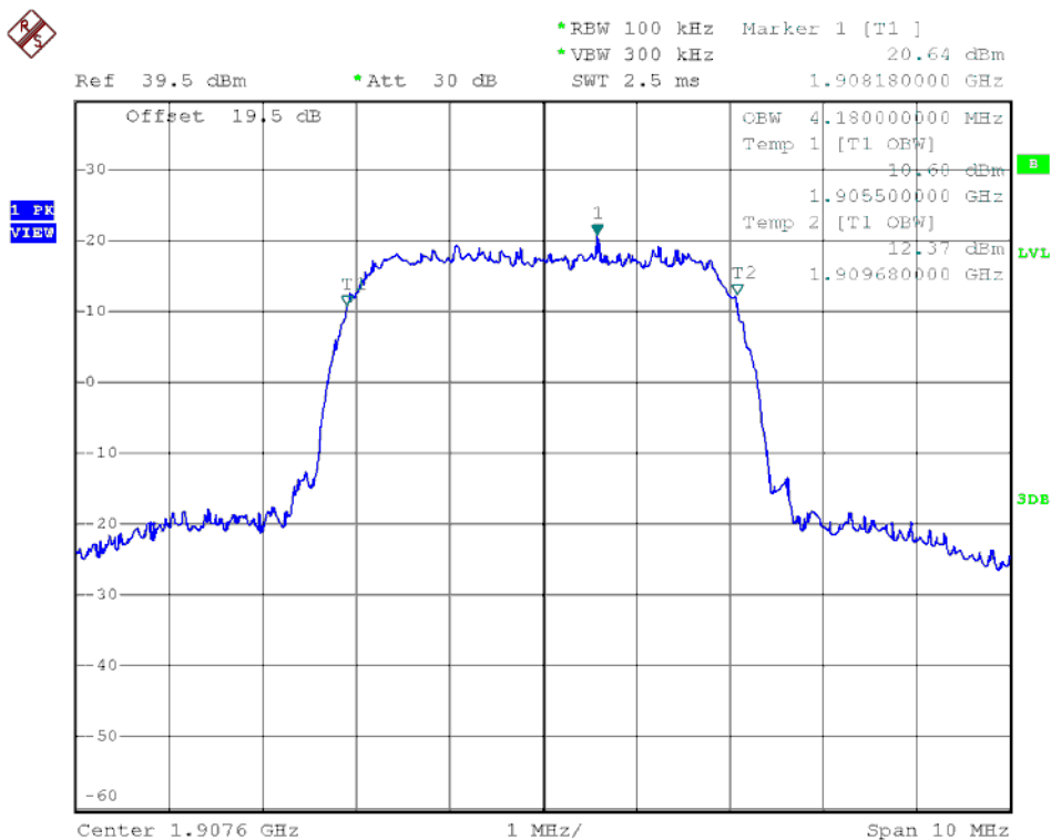
(Plot N6: HSPA+ 1900MHz Channel = 9538)
