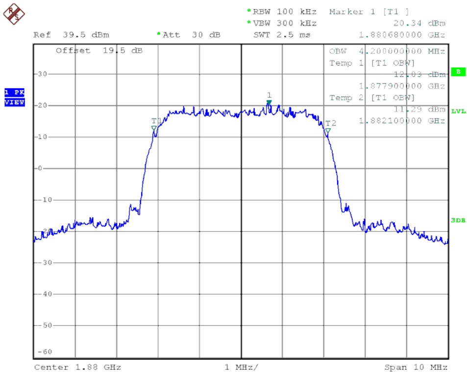
(Plot N4: HSPA+ 1900 MHz Channel = 9400)
