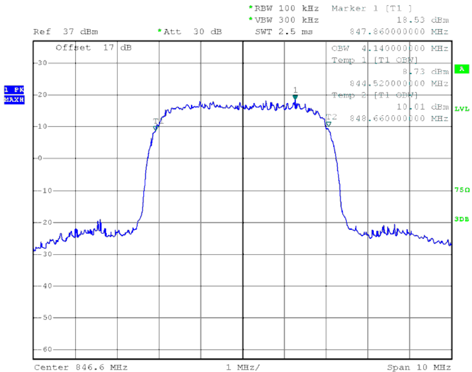
(Plot G6: WCDMA 850MHz Channel = 4233)
