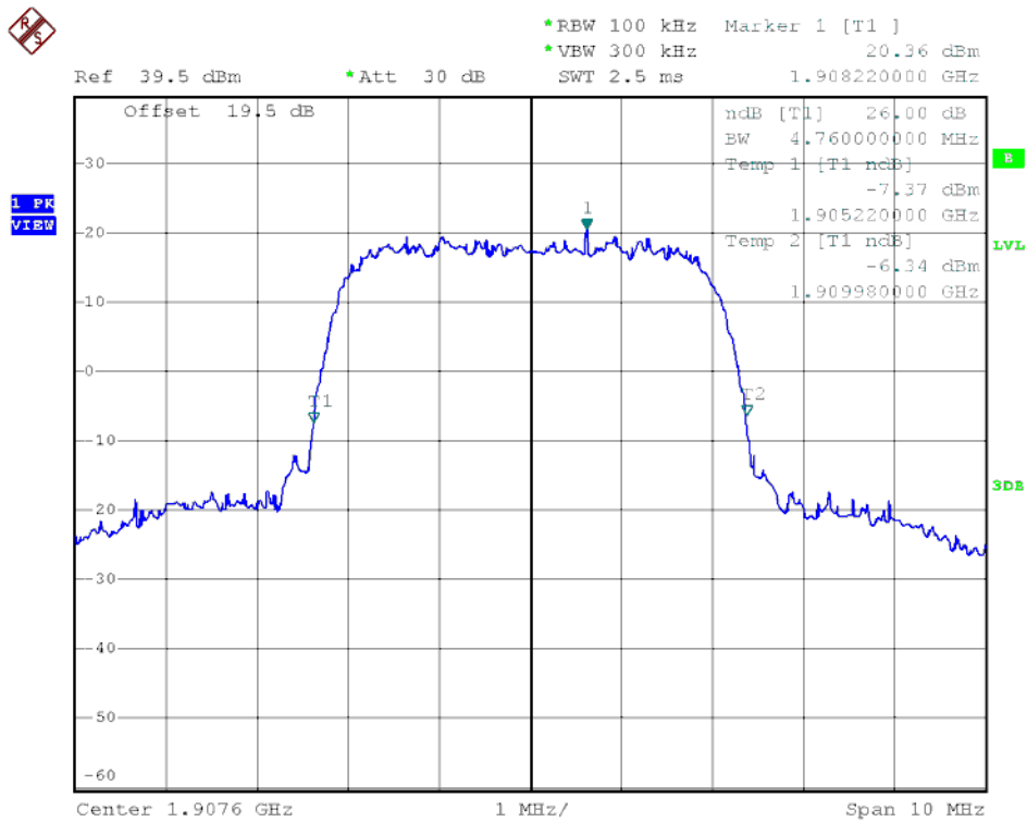
(Plot N5: HSPA+ 1900MHz Channel = 9538)
