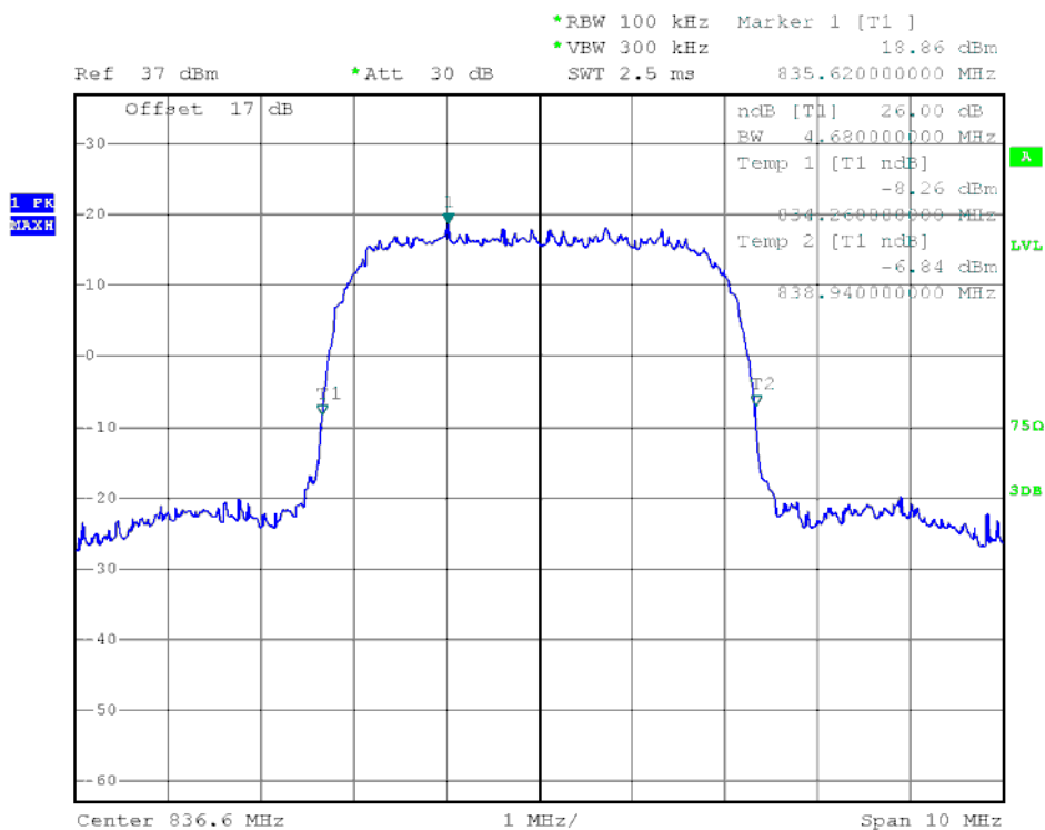
(Plot I3: HSDPA 850 MHz Channel = 4183)
