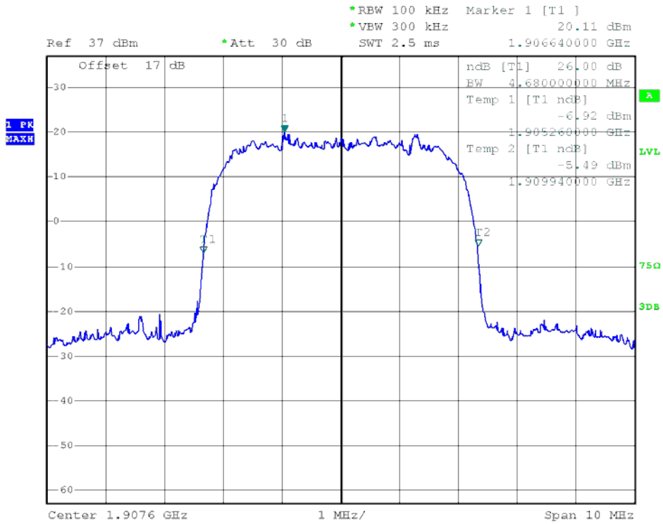
(Plot L5: HSUPA 1900MHz Channel = 9538)
