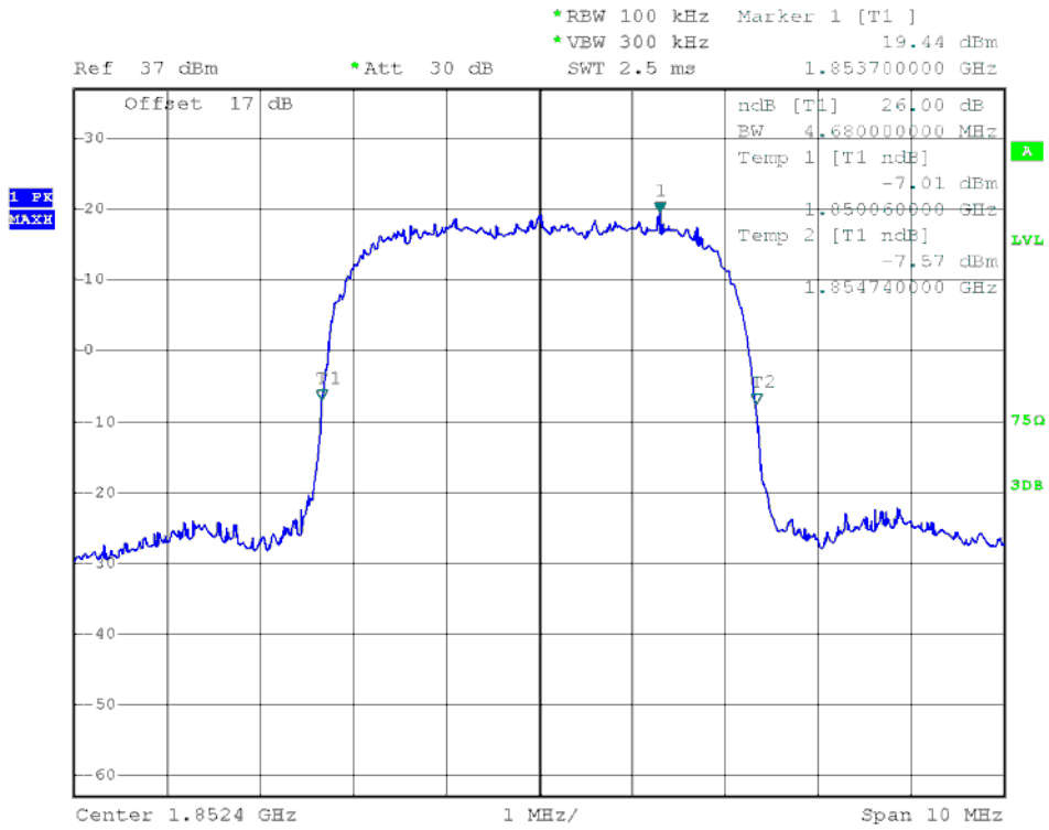
(Plot L1: HSUPA 1900MHz Channel = 9262)
