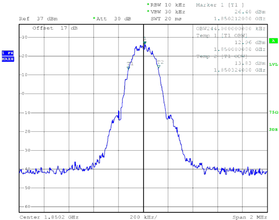
(Plot F2: EDGE 1900MHz Channel = 512)
