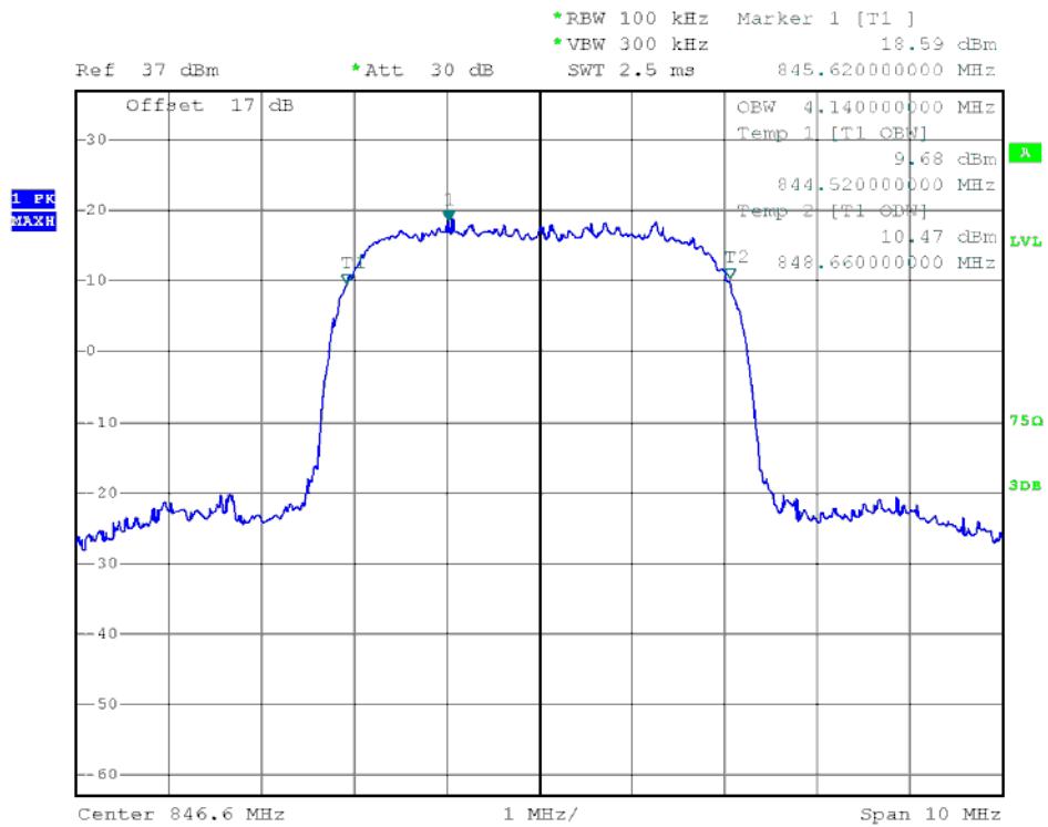
(Plot K6: HSUPA 850MHz Channel = 4233)
