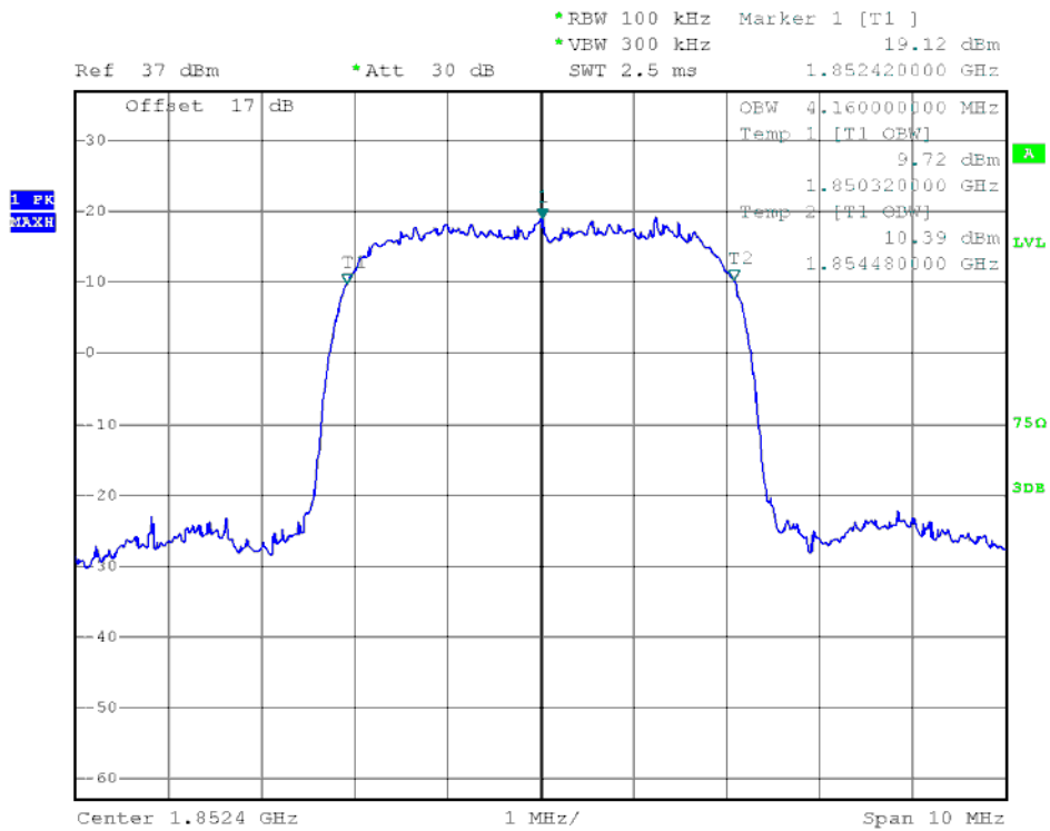
(Plot L2: HSUPA 1900MHz Channel = 9262)
