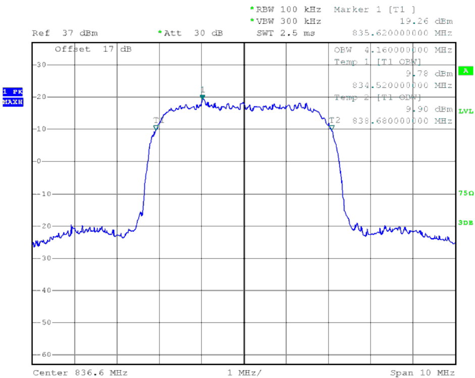
(Plot G4: WCDMA 850 MHz Channel = 4183)
