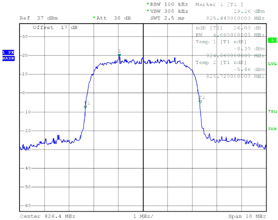
(Plot K1: HSUPA 850MHz Channel = 4132)
