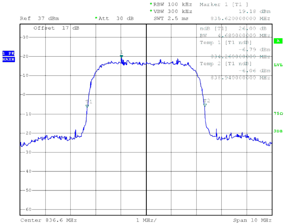
(Plot K3: HSUPA 850 MHz Channel = 4183)
