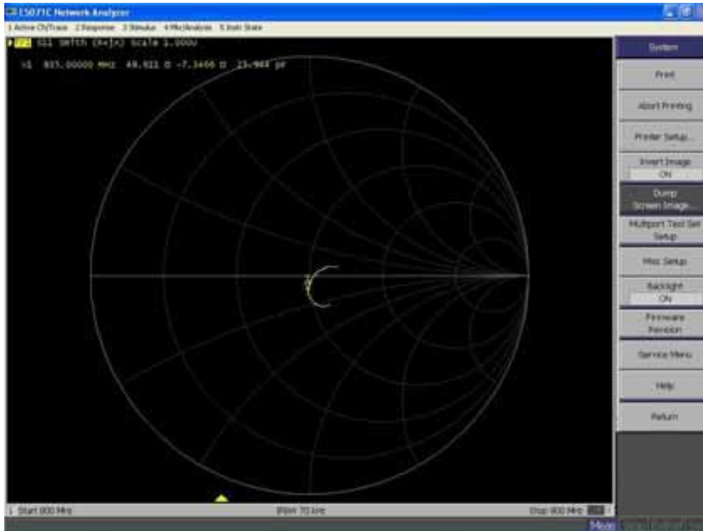
Measured impedance: 48.611\Omega - 7.3j\Omega
