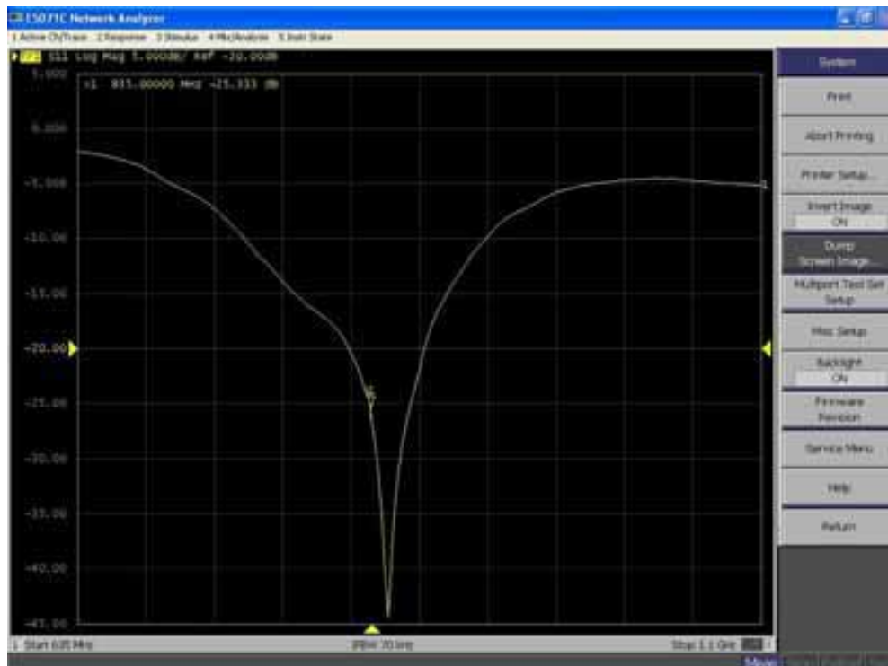
Measured Return loss : -25.333 dB
