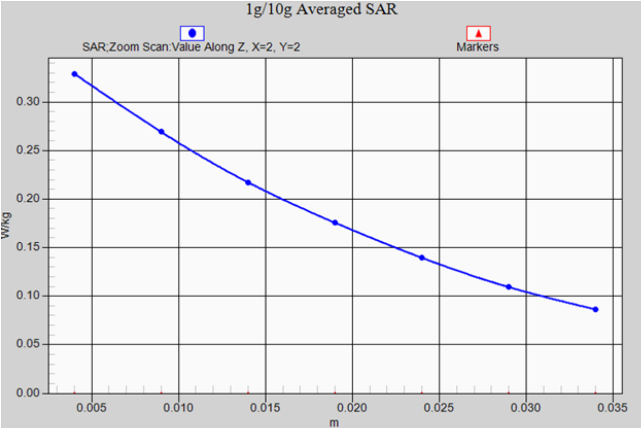
GSM850 LEFT/CHEEK-Low_ axis scan
