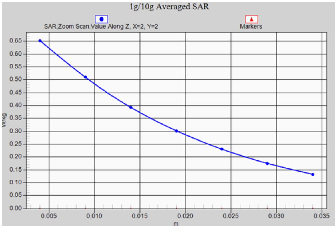
WCDMA Band V(Body)/Back side-High_ axis scan
