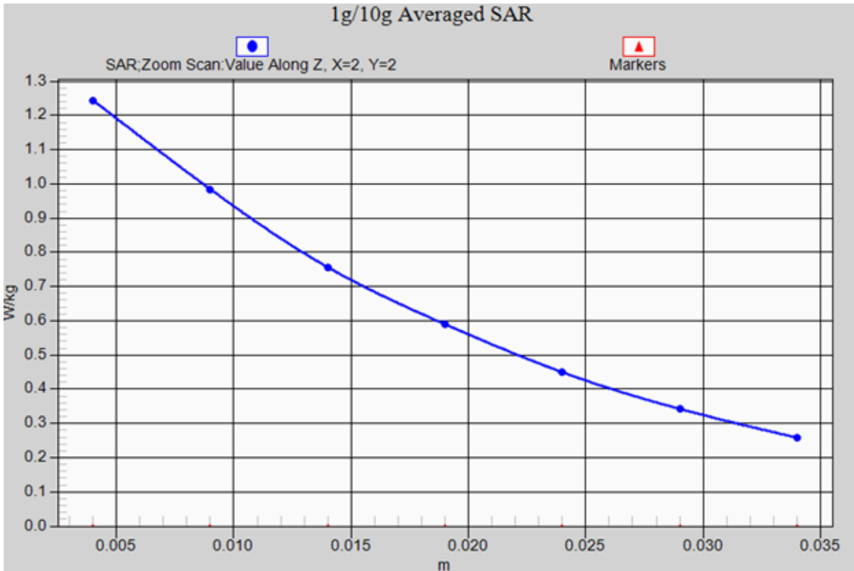
GPRS 850/Back side-Mid_axis scan
