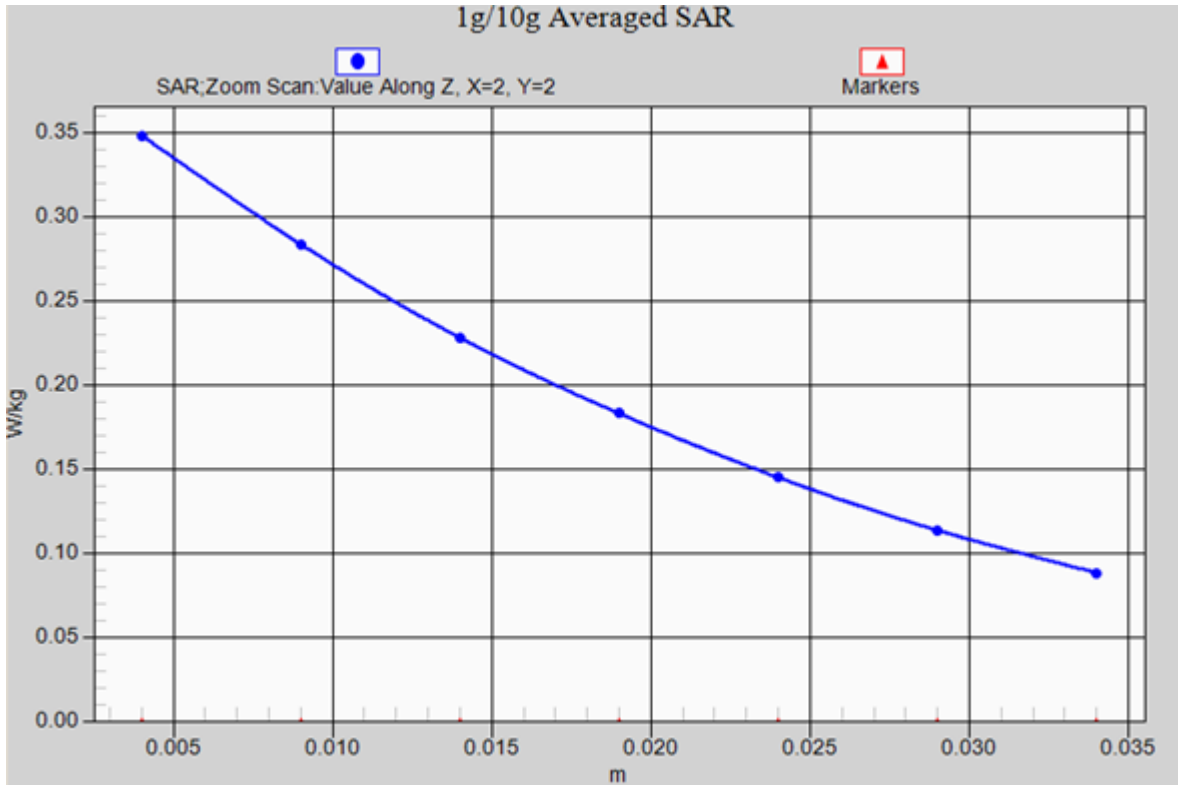
WCDMA Band V- LEFT/CHEEK-High_ axis scan
