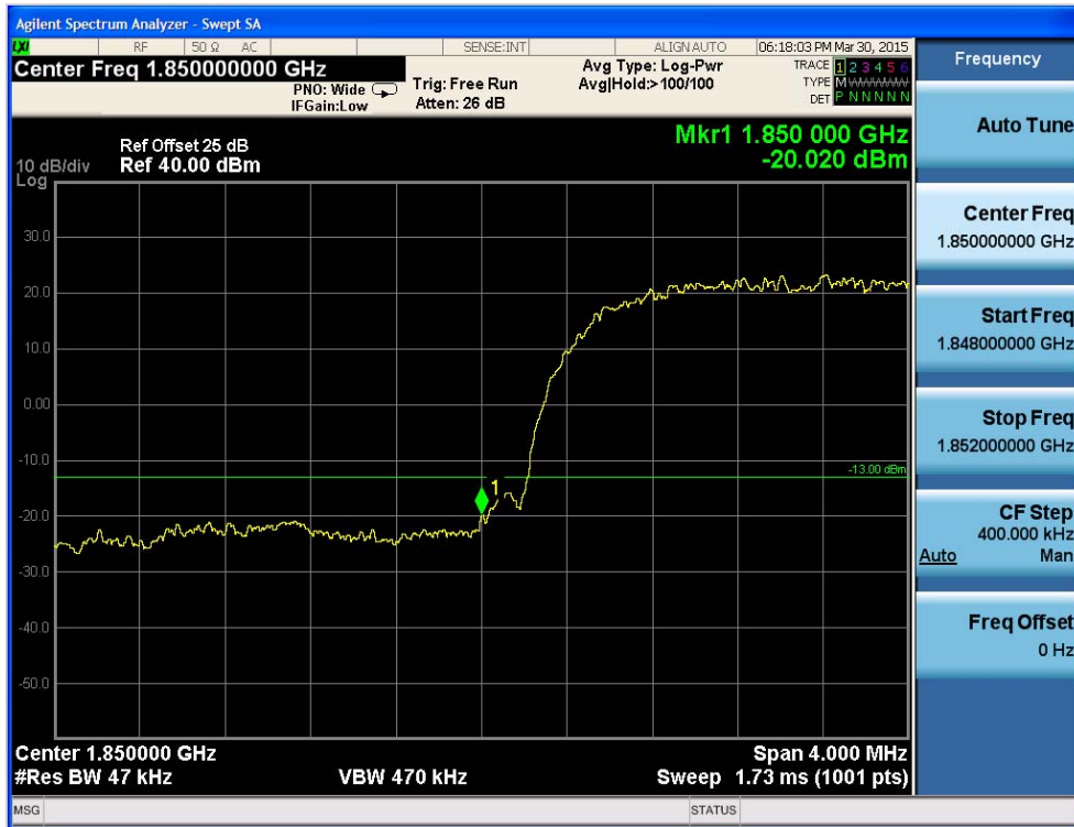
Fig.35 WCDMA Band II-CH9263Band Edge Compliance
