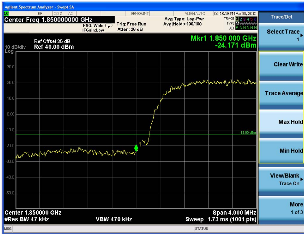
Fig.37 WCDMA Band II-CH9263Band Edge Compliance HSDPA Subtest 1
