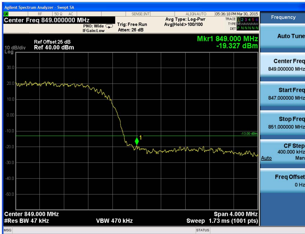
Fig.32 WCDMA Band V-CH4232 Band Edge Compliance HSDPA Subtest 1
