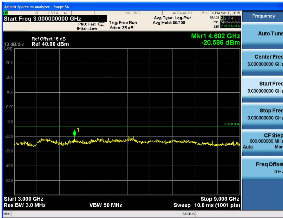
Fig.46 WCDMA Band V on Channel 4175 3GHz~9GHz
