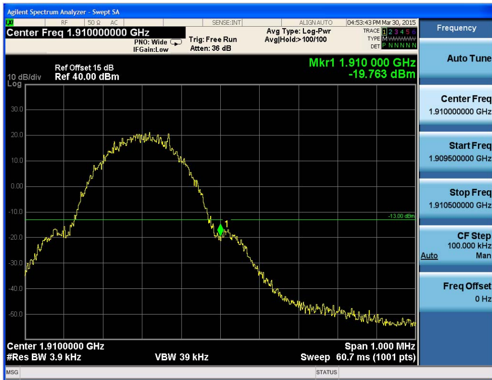
Fig.28 GSM1900-CH810 Band Edge Compliance
