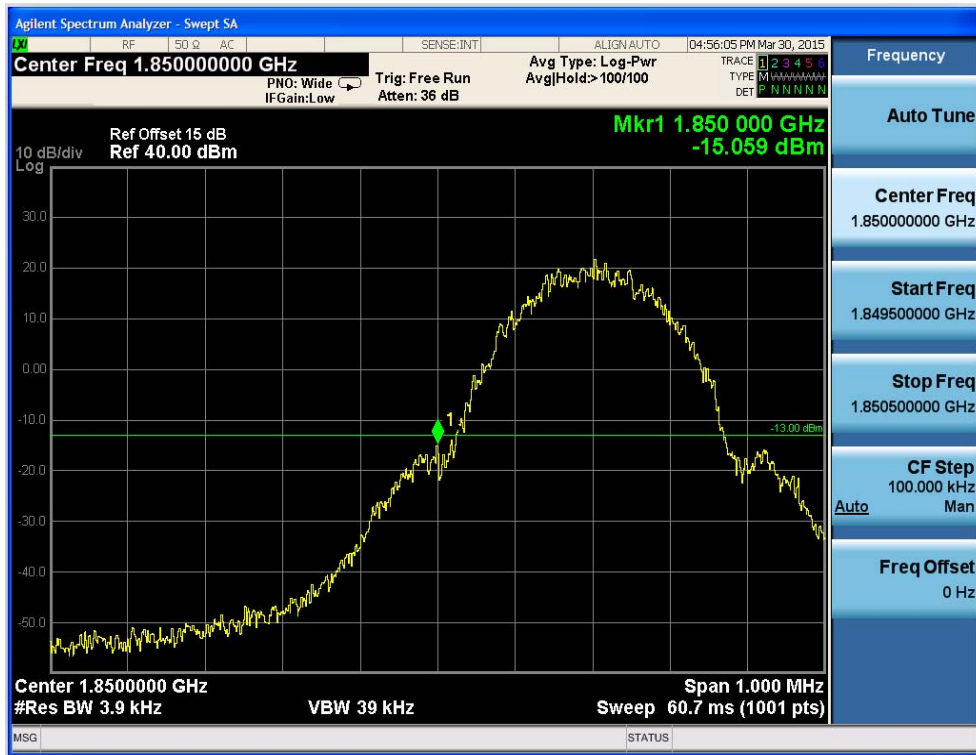
Fig.27 GSM1900-CH512 Band Edge Compliance
