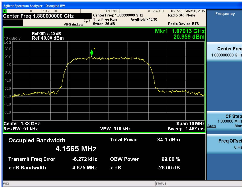
Fig.20 WCDMA Band II-CH9400 Occupied Bandwidth (HSDPA Subtest 1)
