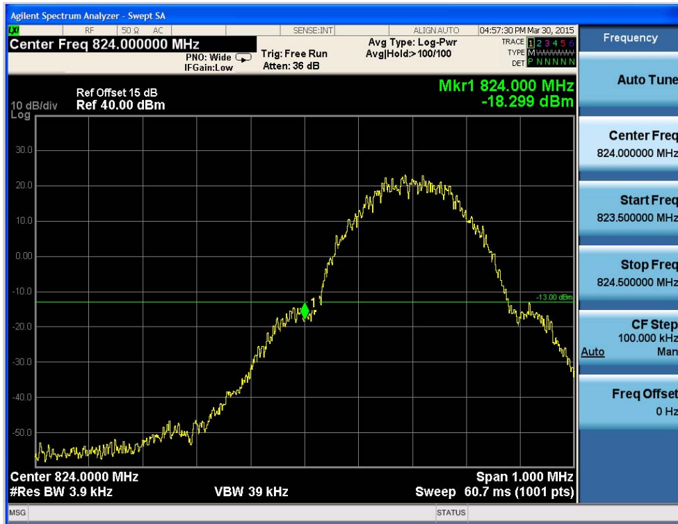
Fig.25 GSM850-CH128 Band Edge Compliance
