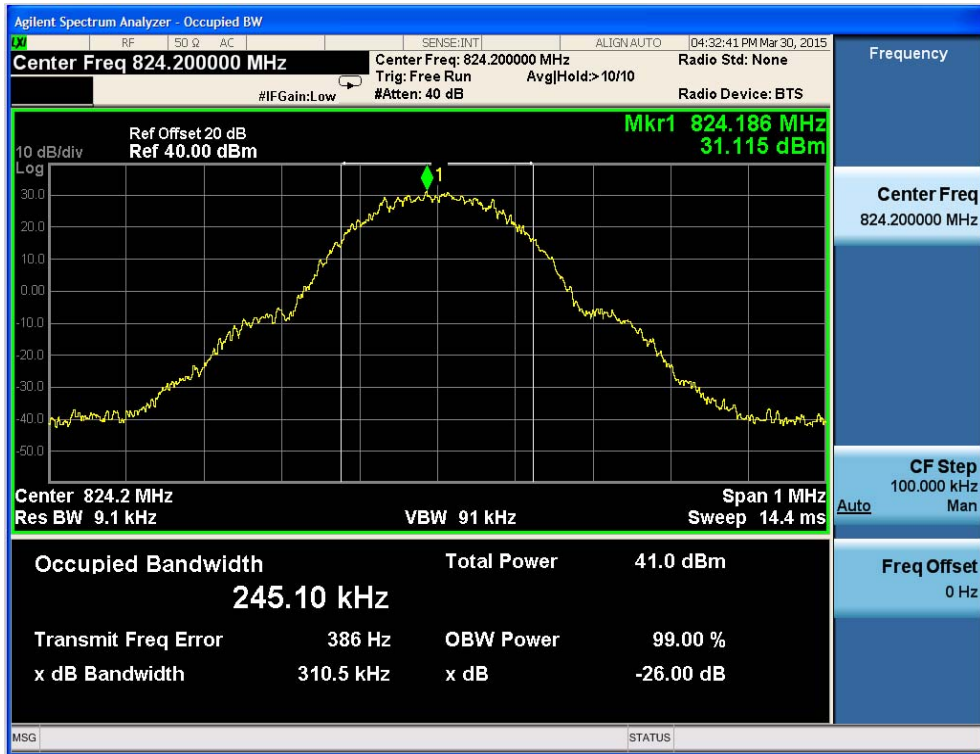
Fig.1 GSM850-CH128 Occupied Bandwidth
