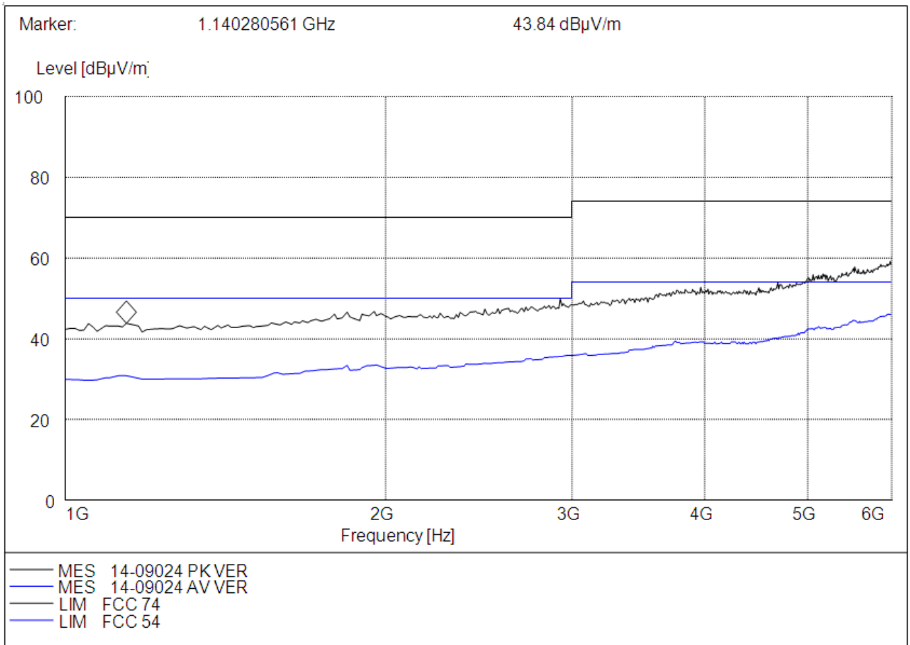
(Plot F: Test Antenna Vertical 1G – 6G)
