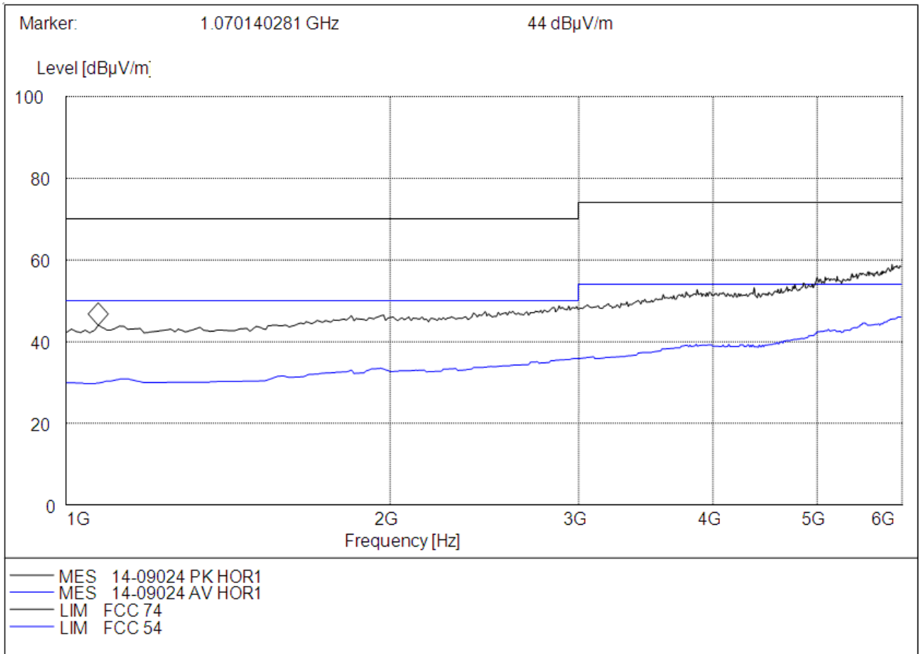
(Plot E: Test Antenna Horizontal 1G – 6G)
