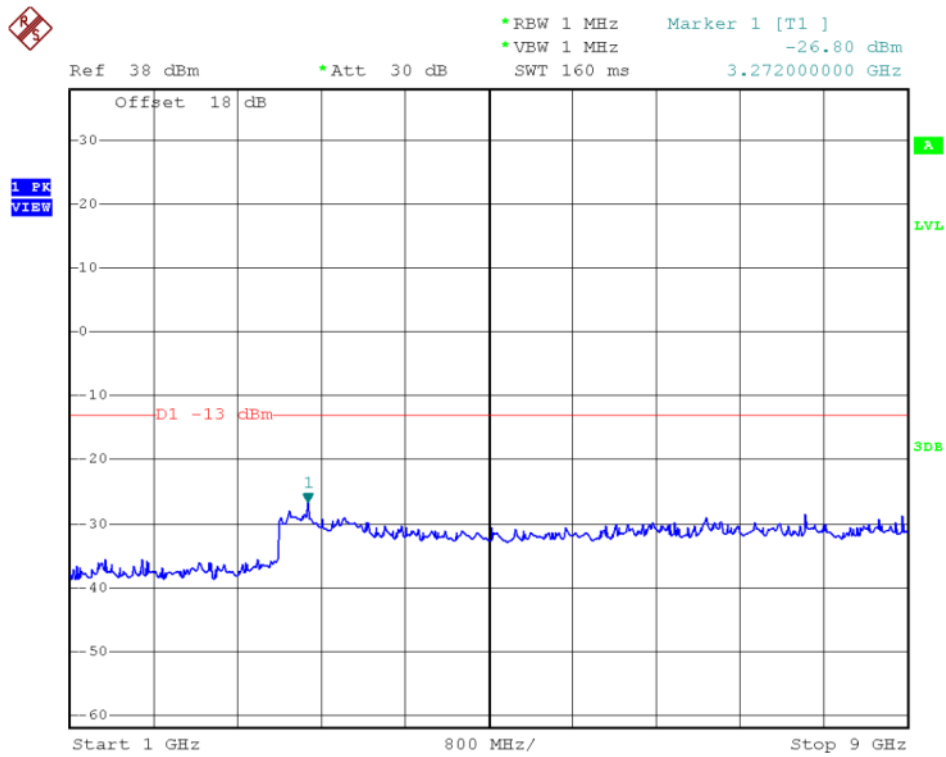
(Plot E2.1: HSDPA 850MHz Channel = 4183, 1GHz to 9GHz)
