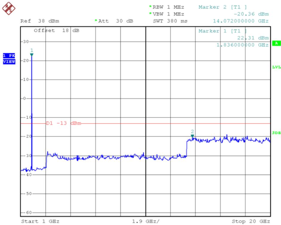
(Plot F1.1: HSDPA1900MHz Channel = 9262, 1GHz to 20GHz)
