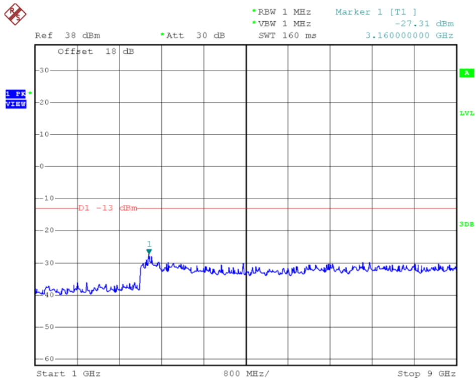
(Plot E1.1: HSDPA 850MHz Channel = 4132, 1GHz to 9GHz)
