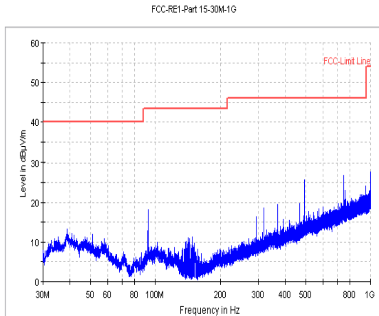
Fig.180 Radiated Spurious Emission (802.11n-40M, Ch6, 30MHz-1 GHz)
