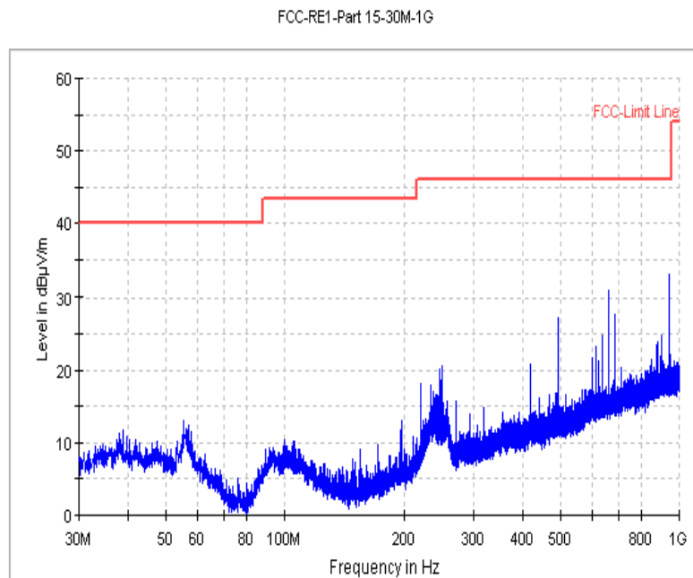
Fig.162 Radiated Spurious Emission (802.11g, Ch1,30MHz-1 GHz)
