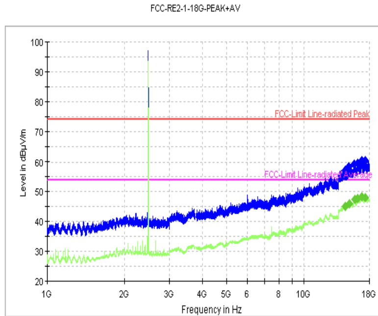
Fig. 71 Radiated Spurious Emission (8DPSK, Ch78, 1 GHz ~18 GHz)
