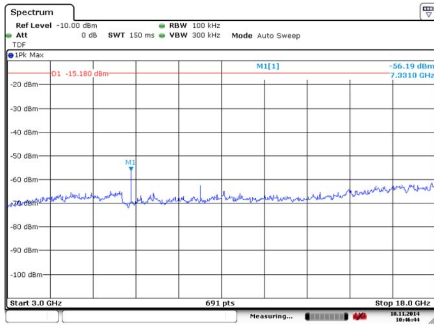
Fig. 27 Conducted Spurious Emission (GFSK, Ch39, 3GHz-18 GHz)
