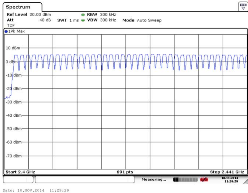
Fig. 90 Hopping channel ch0~39 (GFSK, Ch39)
