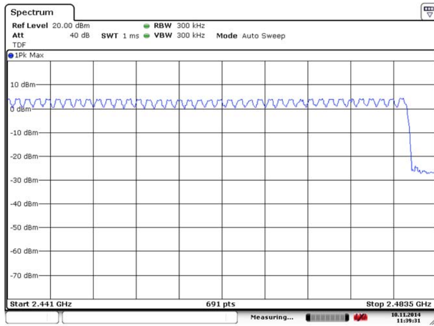
Fig. 95 Hopping channel ch39~78 (8DPSK, Ch39)
