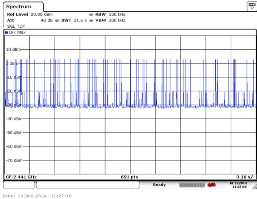
Fig. 89 Number of Transmissions (8DPSK, Ch39)
