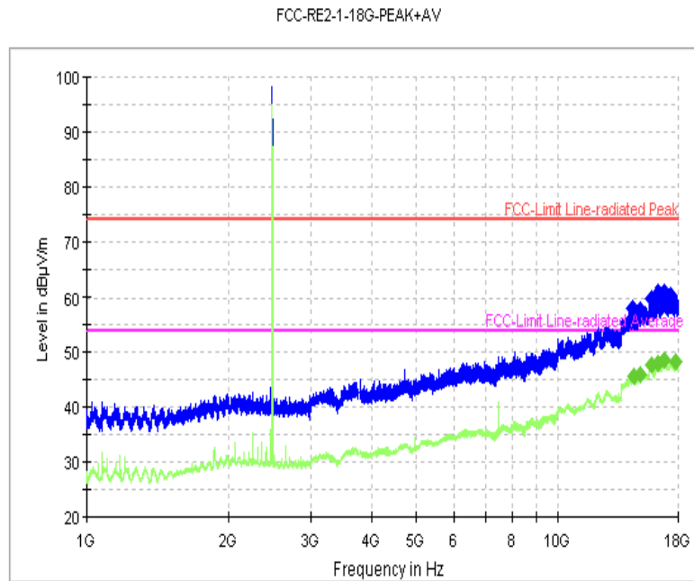
Fig. 55 Radiated Spurious Emission (GFSK, Ch78, 1 GHz ~18 GHz)
