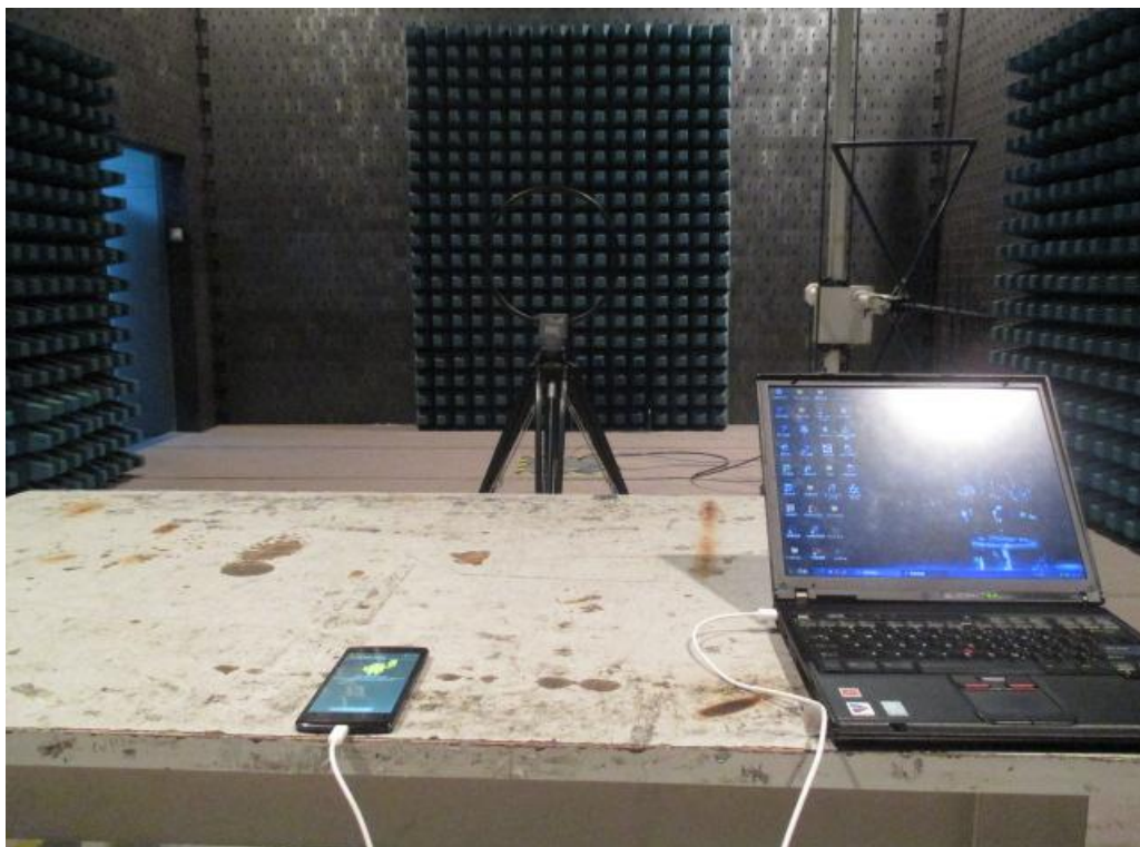
Radiated Emission Test setup photos
