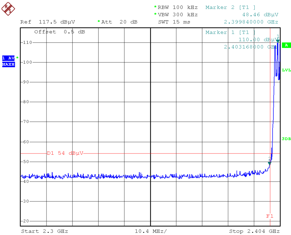
(Plot A2-1: Channel = 0 AVERAGE)
