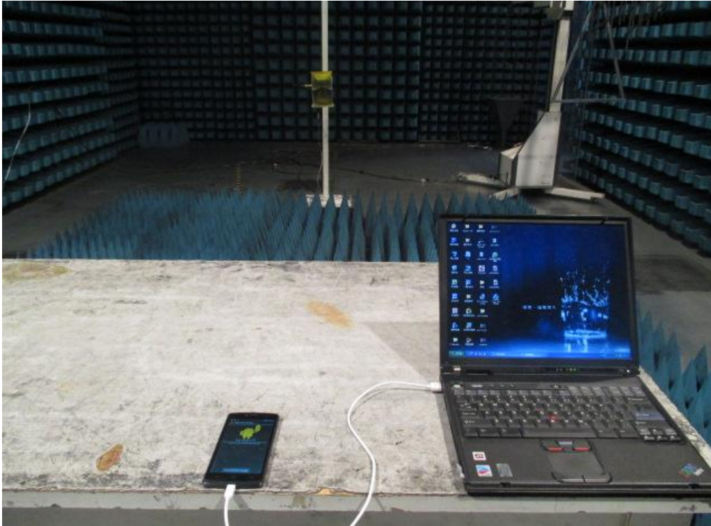
Radiated Emission of 1-18G
