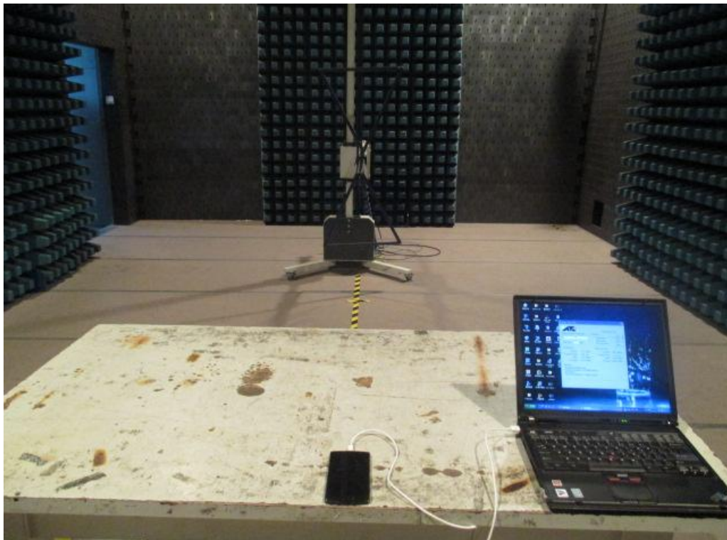
Radiated Emission of 30M-1G
