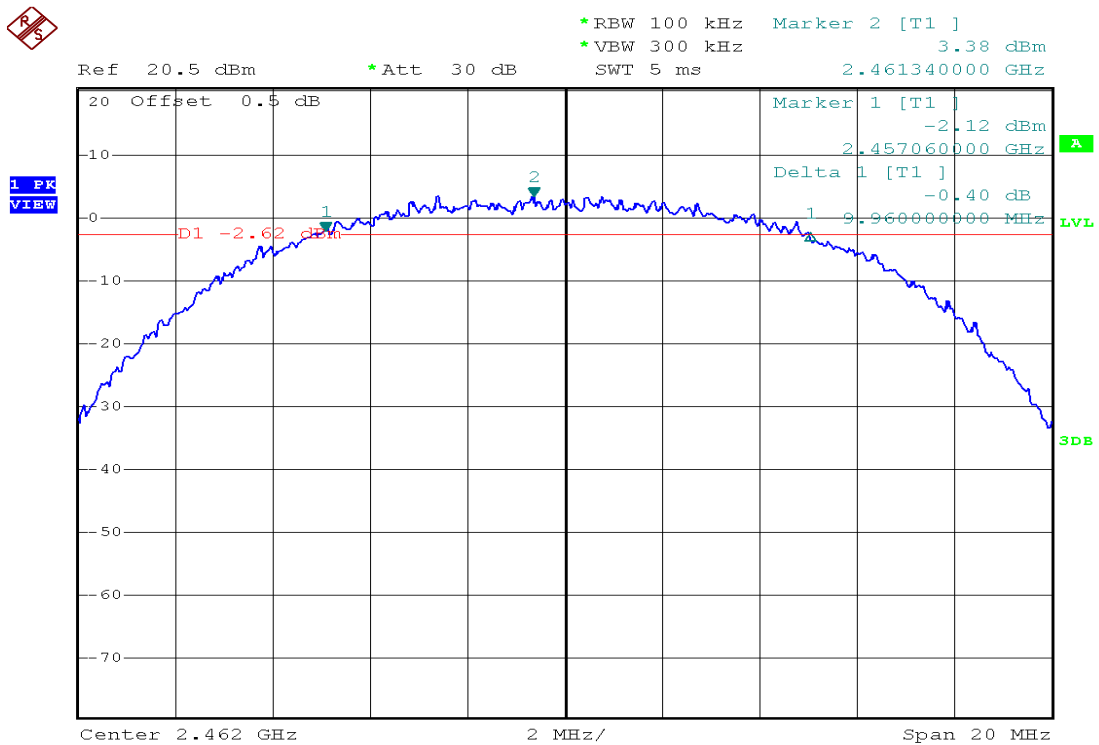
(Plot 2.3 C: Channel 11: 2462MHz @ 802.11b)
