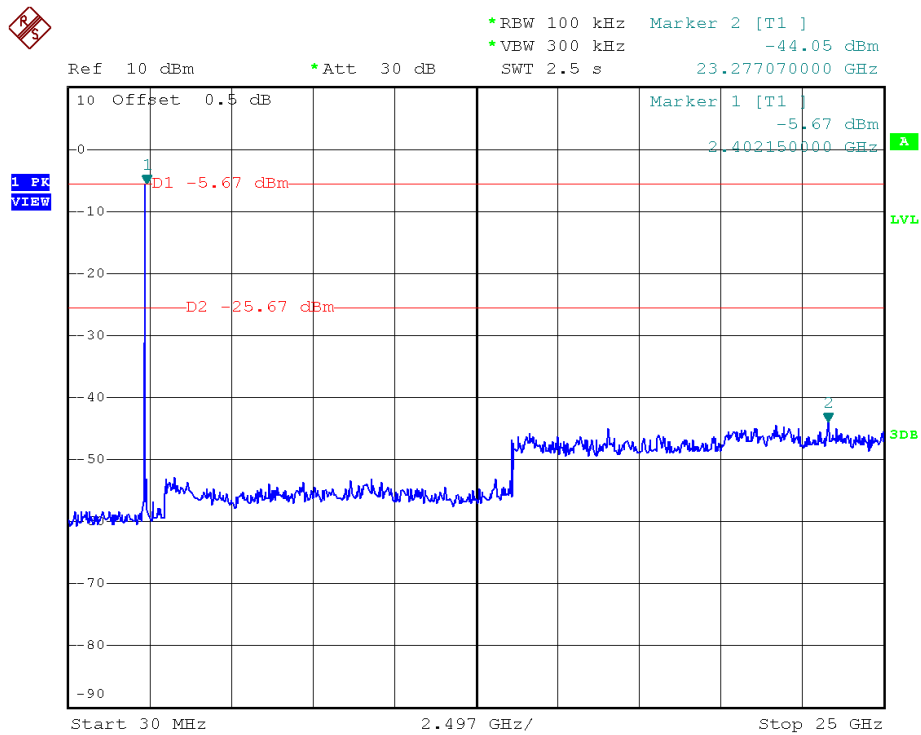
(Plot 2.4 G: Channel = 1, 30MHz to 25GHz@ 802.11n-20)
