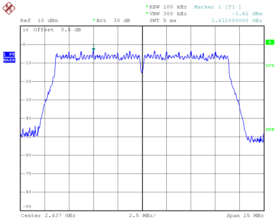
(Plot 2.5 H: Channel = 6 @ 802.11n-20)
