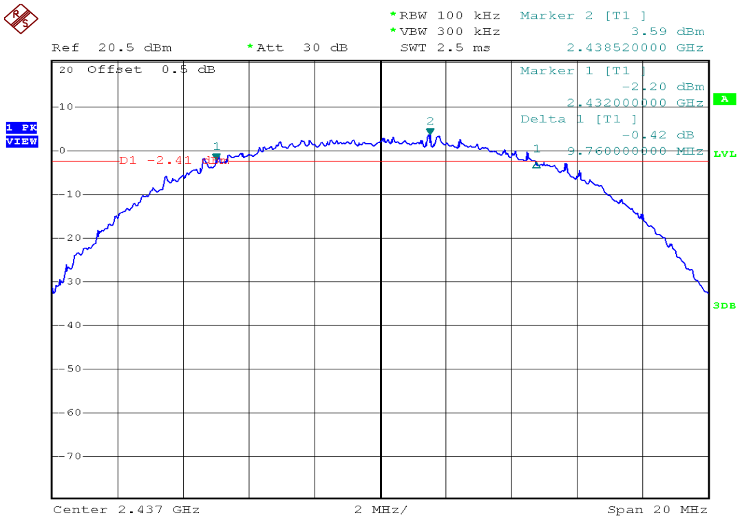
(Plot 2.3 B: Channel 6: 2437 MHz @ 802.11b)
