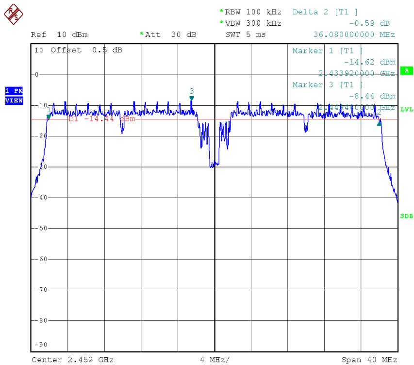
(Plot 2.3 L: Channel 9: 2452MHz @ 802.11n-40)
