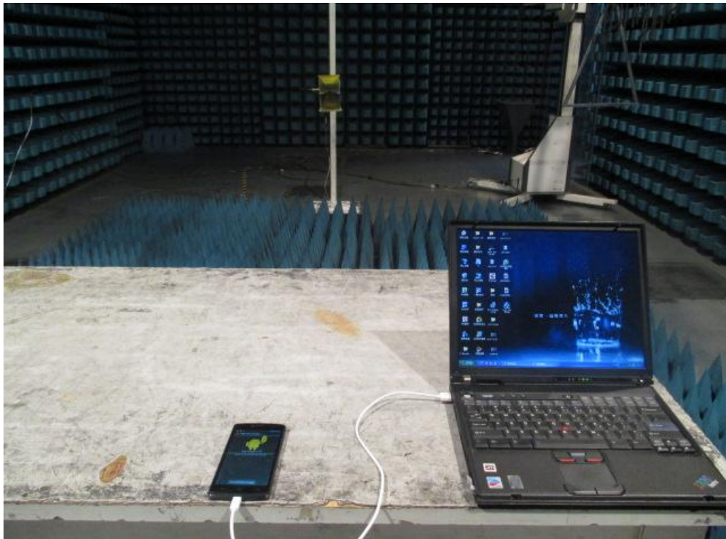
Radiated Emission of 1-18G
