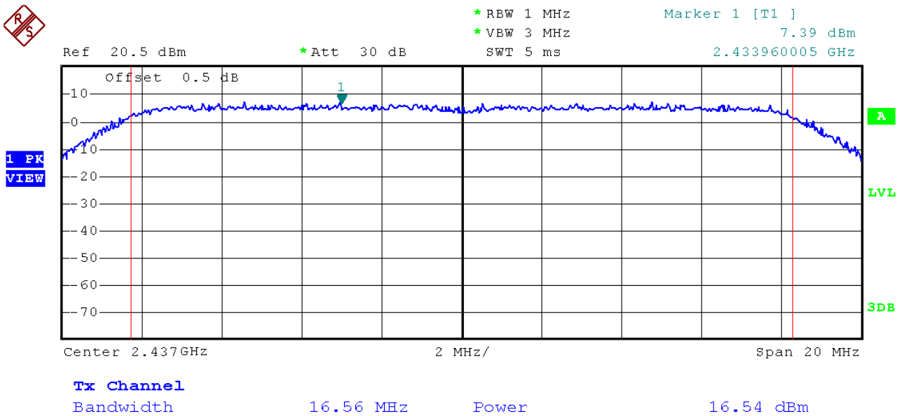
(Plot 2.2 E: Channel 6: 2437MHz @ 802.11g)
