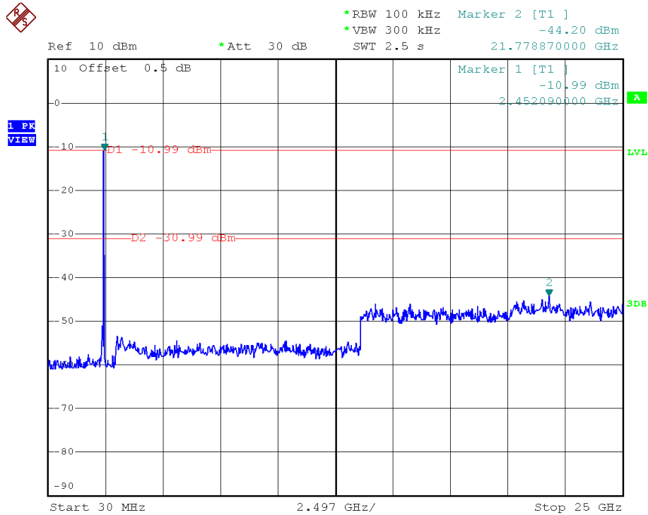
(Plot 2.4 L: Channel = 9, 30MHz to 25GHz@ 802.11n-40)
