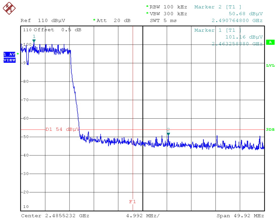
(Plot 2.6 C4: Channel = 11 AVG @ 802.11n-20)
