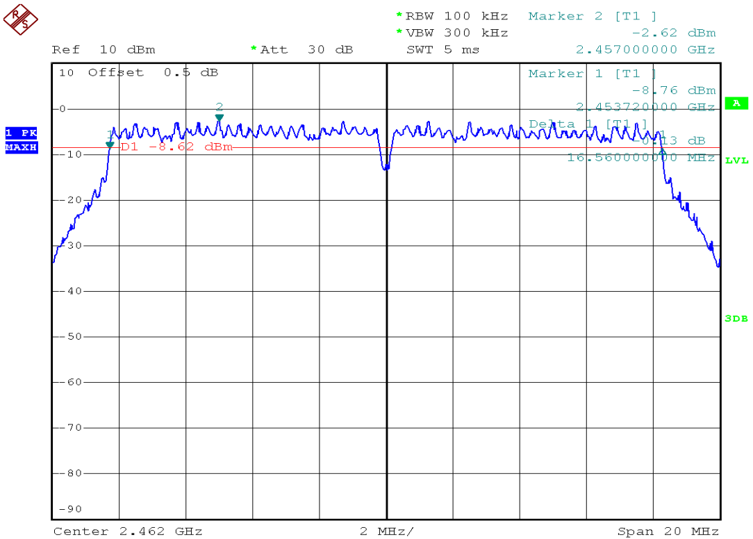
(Plot 2.3 F: Channel 11: 2462MHz @ 802.11g)
