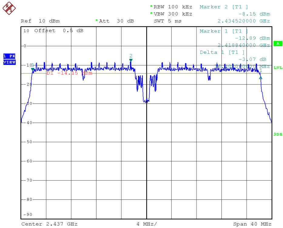
(Plot 2.3 K: Channel 6: 2437MHz @ 802.11n-40)
