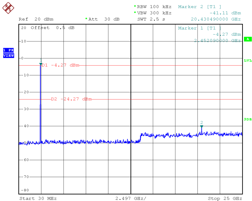
(Plot 2.4 H: Channel = 6, 30MHz to 25GHz@ 802.11n-20)
