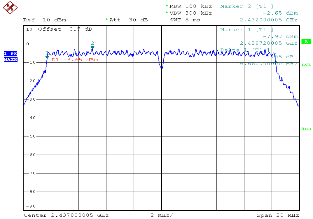
(Plot 2.3 E: Channel 6: 2437MHz @ 802.11g)
