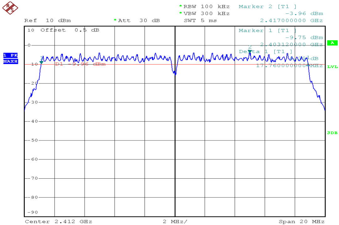
(Plot 2.3 G: Channel 1: 2412MHz @ 802.11n-20)
