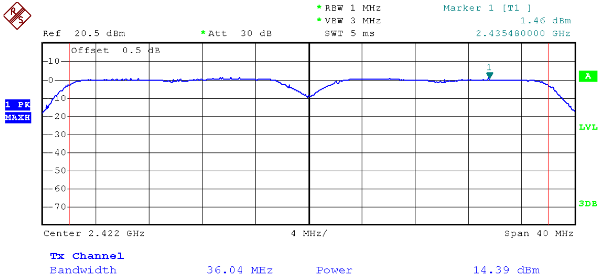
(Plot 2.2 J: Channel 3: 2422MHz @ 802.11n40)
