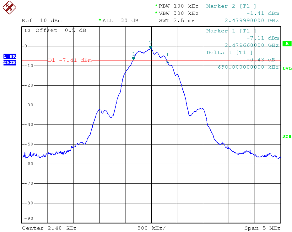
(Plot C1: Channel 39: 2480MHz)
