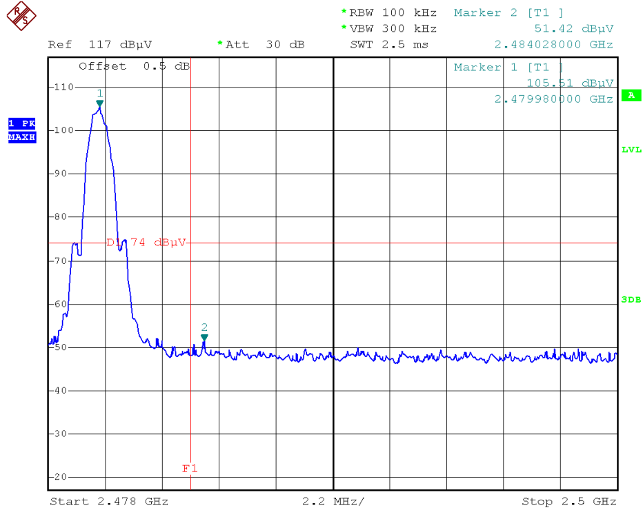
(Plot B1: Channel = 39 PEAK)
