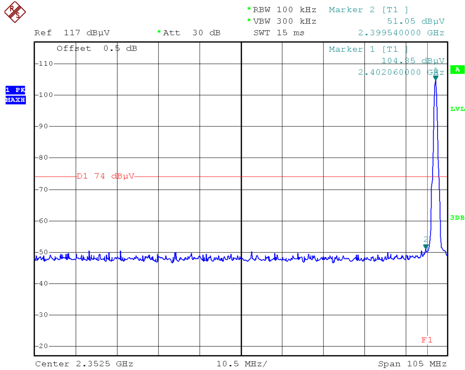
(Plot A1: Channel = 0 PEAK)
