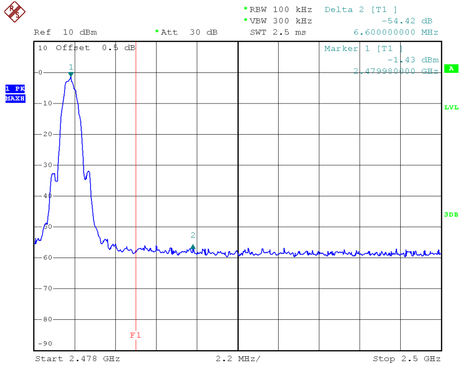
(Plot B: Channel = 39)
