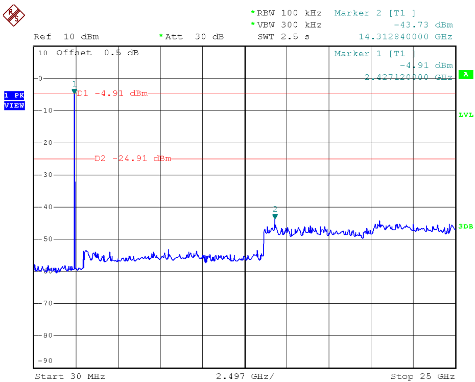
(Plot B.1: Channel = 20, 30MHz to 25GHz)
