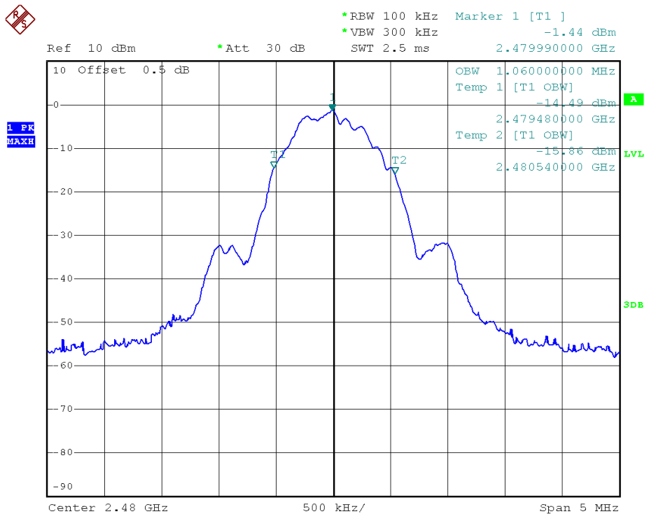
(Plot C2: Channel 39: 2480MHz)
