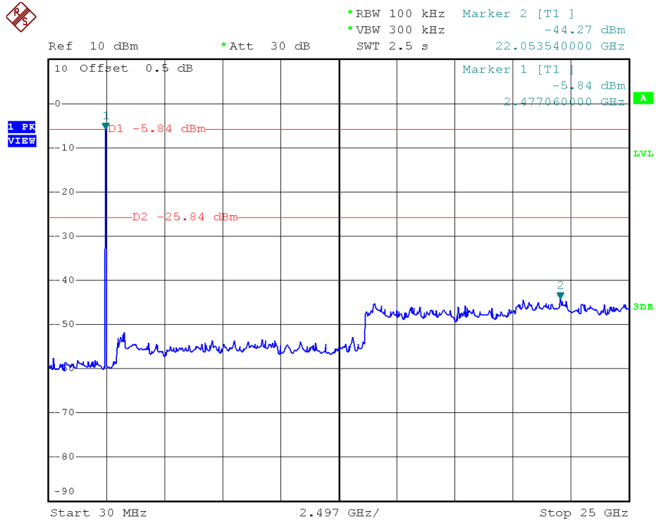
(Plot C.1: Channel = 39, 30MHz to 25GHz)
