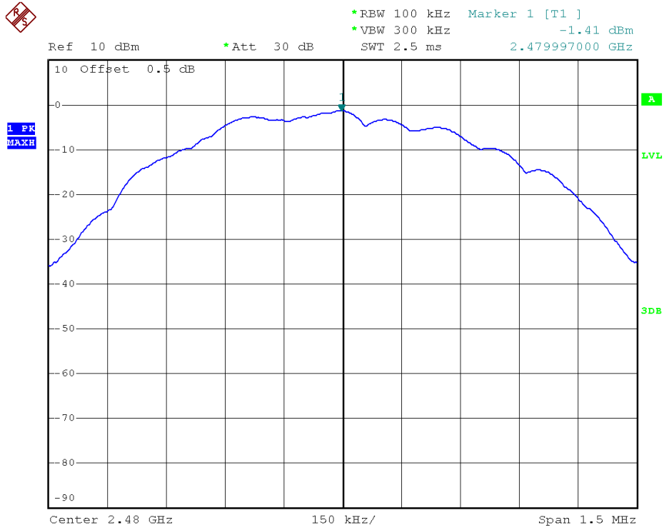
(Plot C: Channel = 39)
