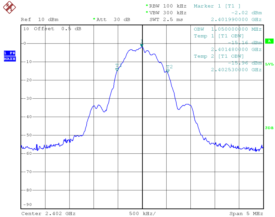
(Plot A2:Channel 0: 2402MHz)
