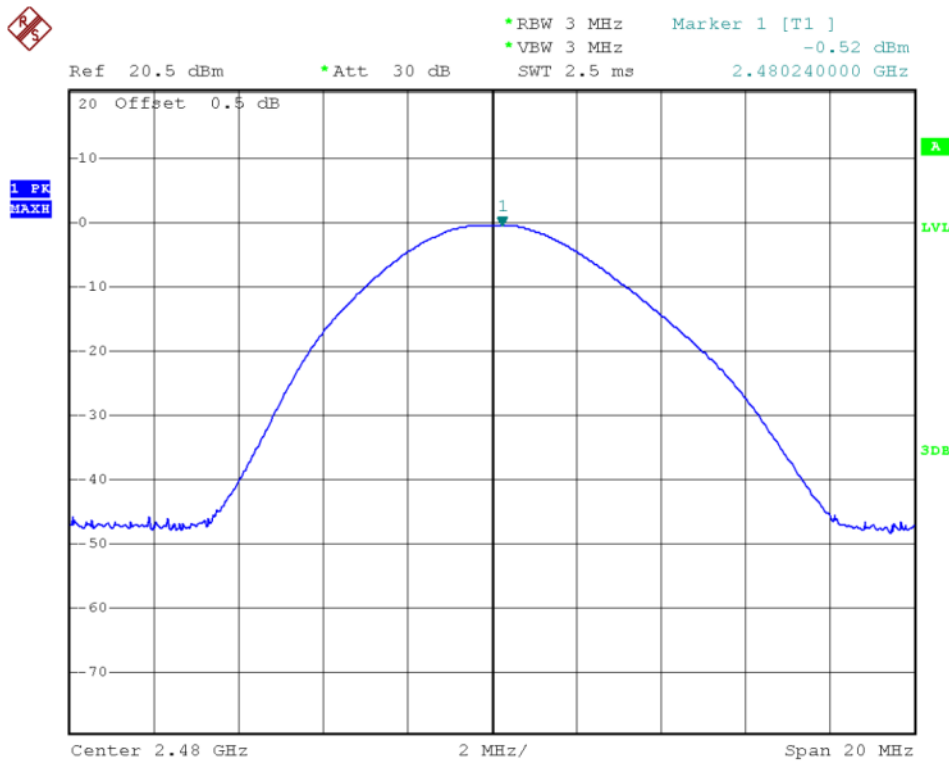
(Plot C: Channel 39: 2480MHz)
