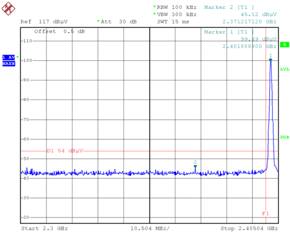
(Plot A2: Channel = 0 AVG)
