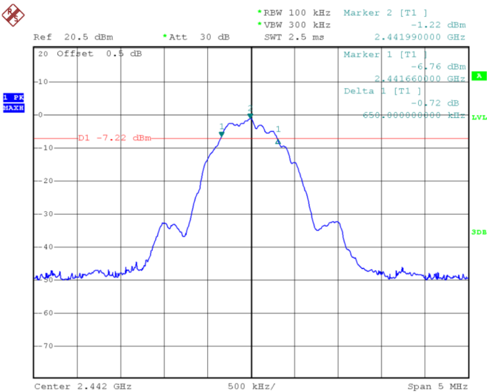
(Plot B1: Channel 20: 2442 MHz)
