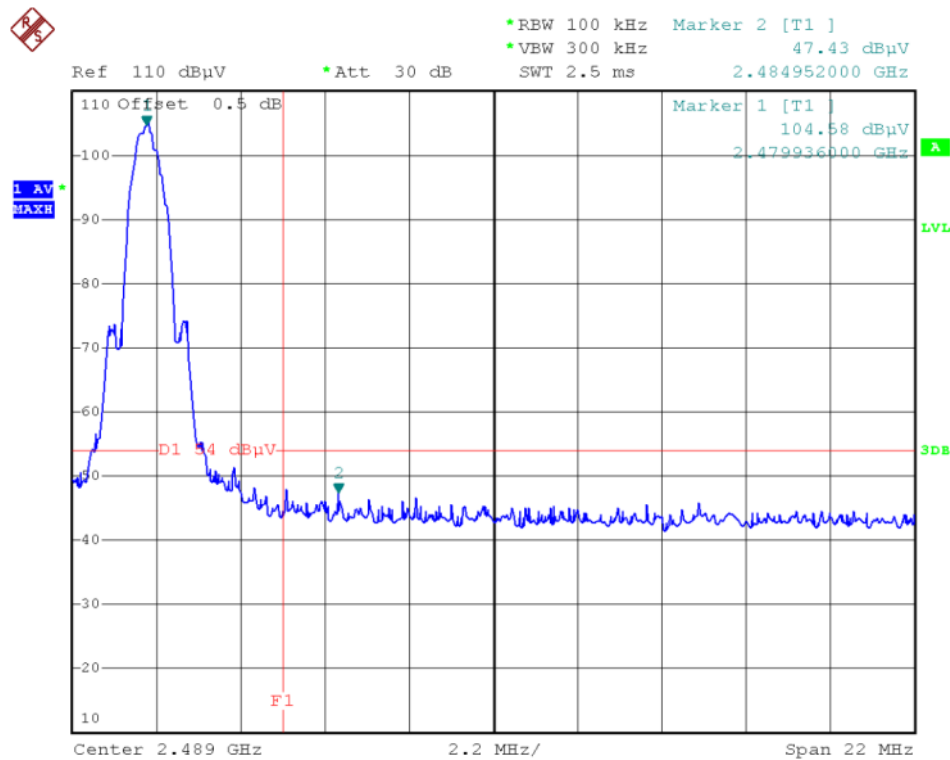
(Plot B2: Channel = 39 AVG )
