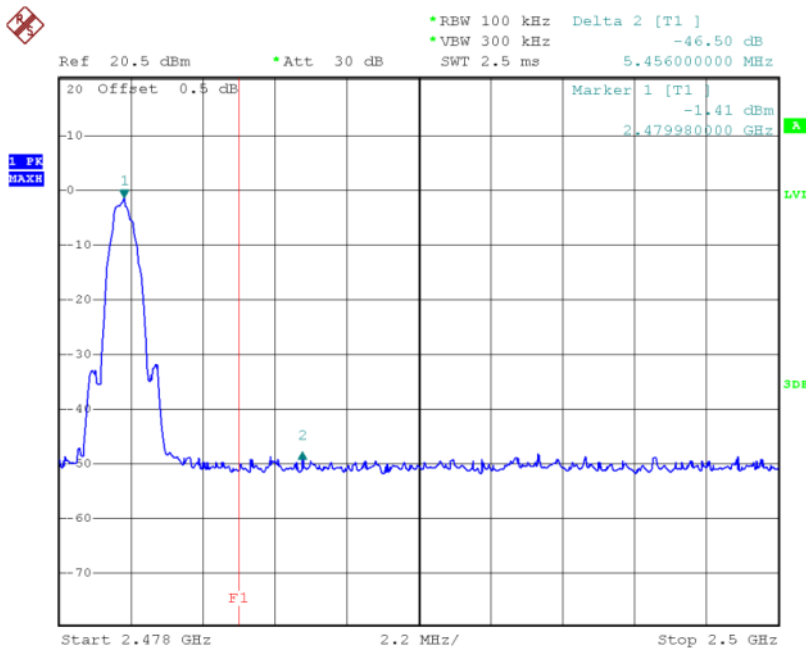
(Plot B: Channel = 39)
