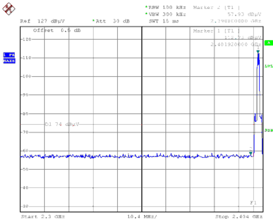
(Plot C1: Channel = 0 PEAK @ \pi/4 -DQPSK)
