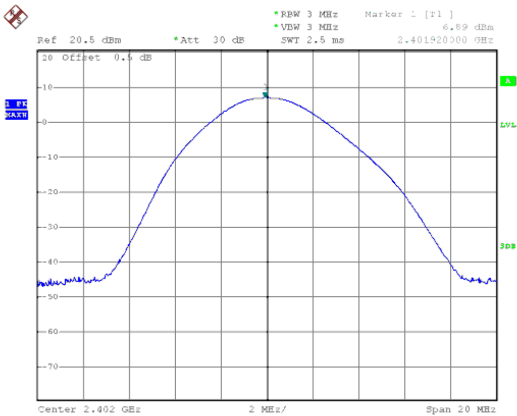
Plot A1: GFSK
