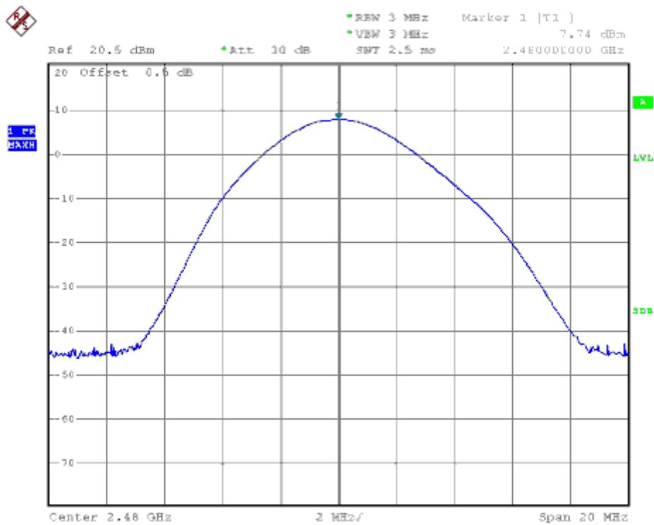
Plot A3: GFSK
