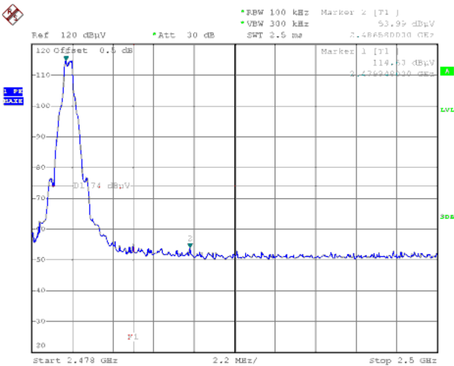
(Plot B1: Channel = 78 PEAK @ GFSK)
