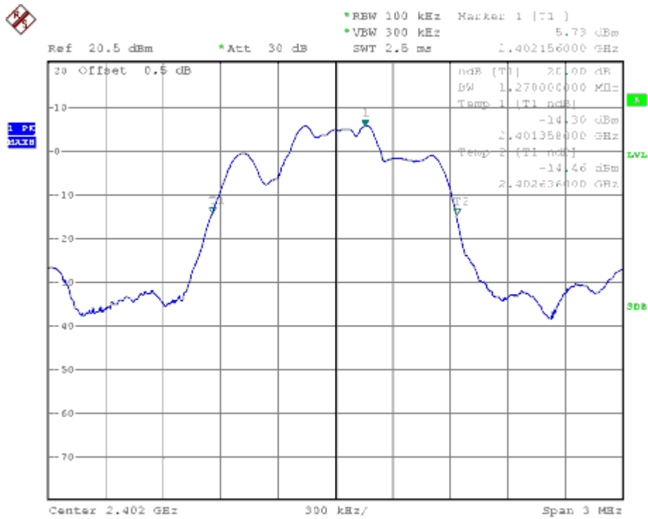
(Plot G: Channel = 2402 @ 8-DPSK)
