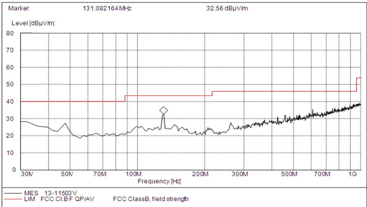
(Plot B: 30MHz to 1GHz, Antenna Vertical)
