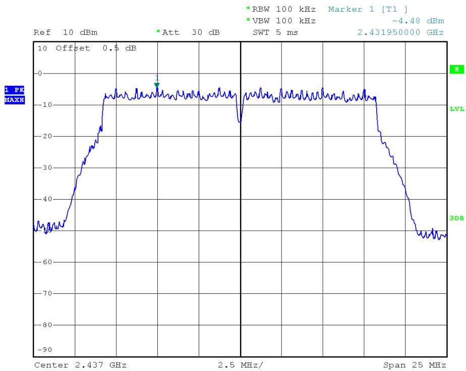
(Plot 2.5 E: Channel = 6 @ 802.11g)
