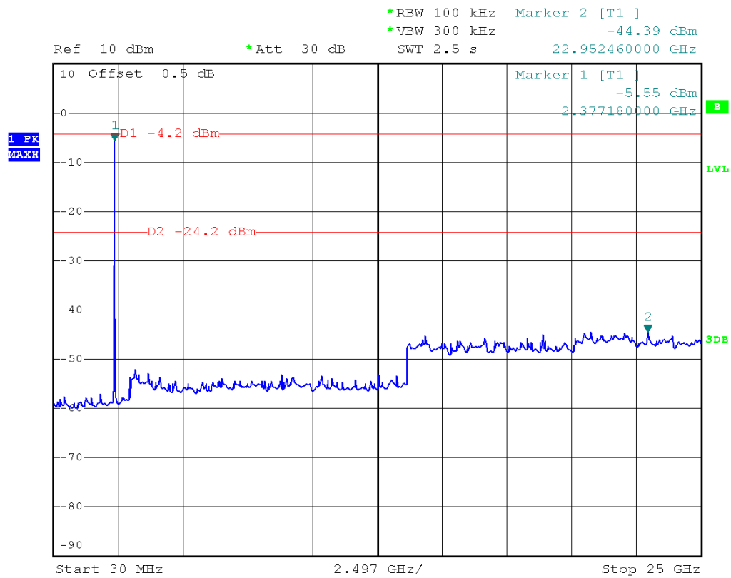
(Plot 2.4 D: Channel = 1, 30MHz to 25GHz@ 802.11g)
