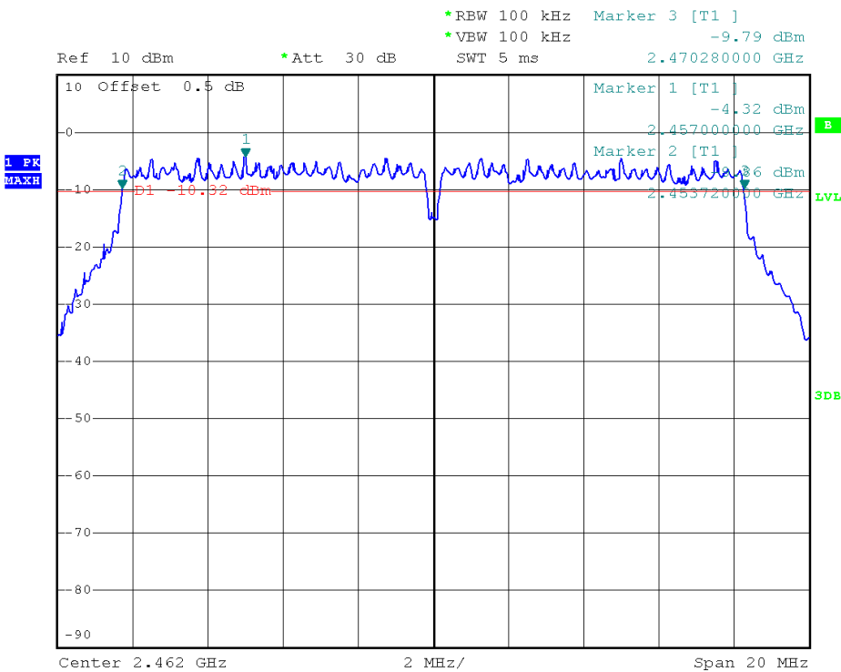
(Plot 2.3 F: Channel 11: 2462MHz @ 802.11g)
