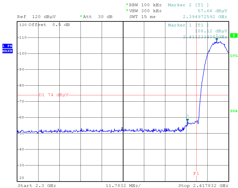
(Plot 2.6 A1: Channel = 1 Peak @ 802.11b)
