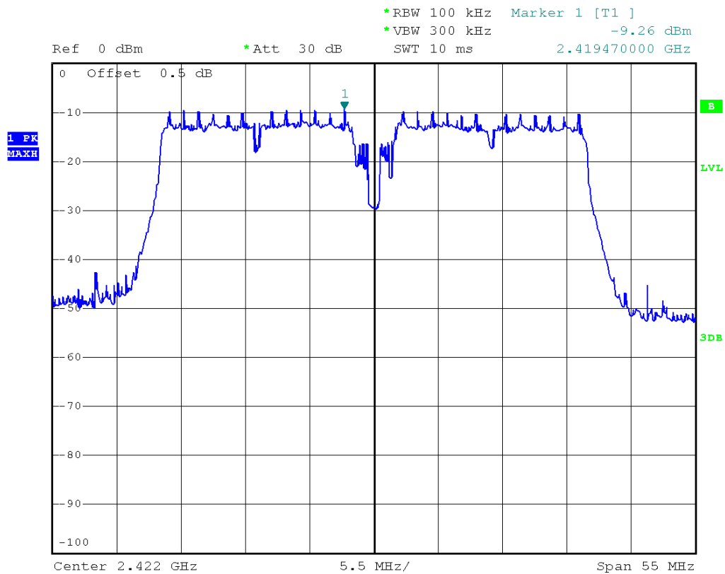
(Plot 2.5 J: Channel = 3 @ 802.11n-40)
