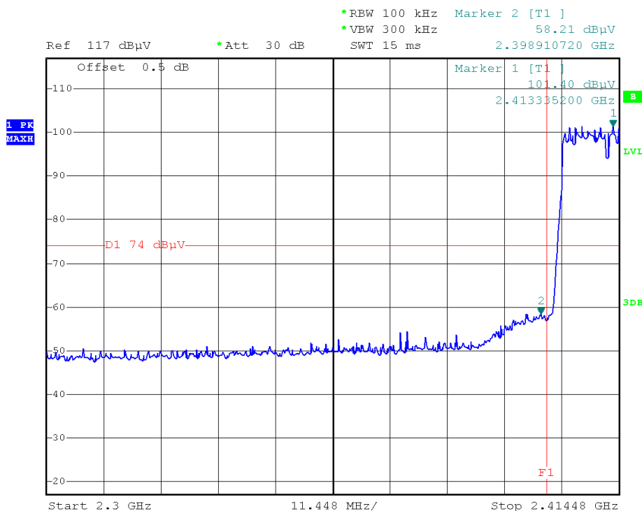
(Plot 2.6 C1: Channel = 1 Peak @ 802.11n-20)
