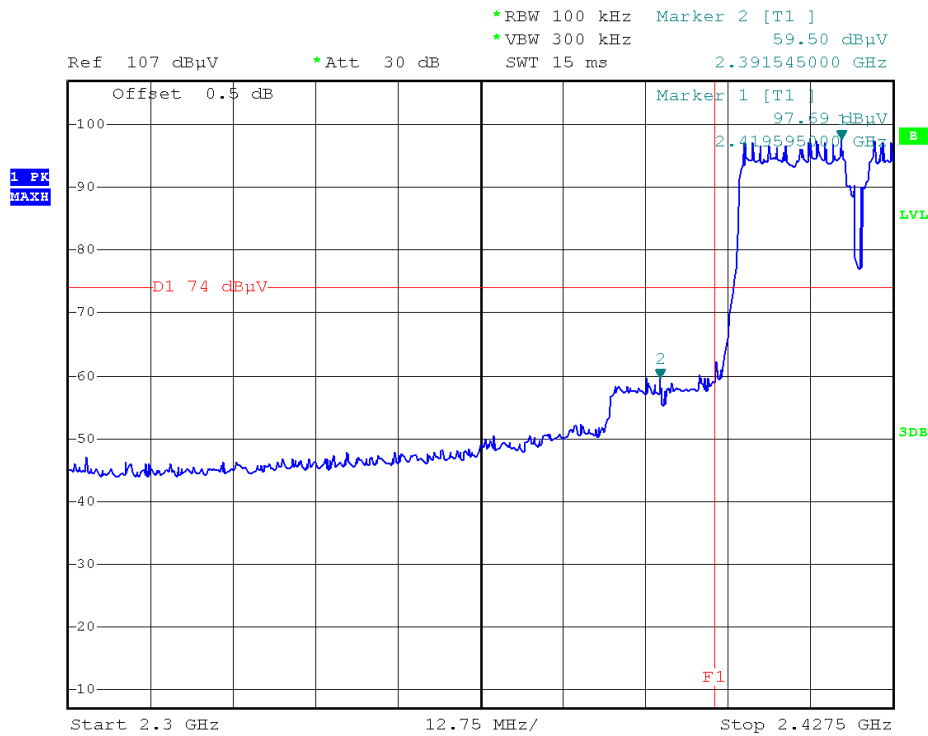
(Plot 2.6 D1: Channel = 3 Peak @ 802.11n-40)
