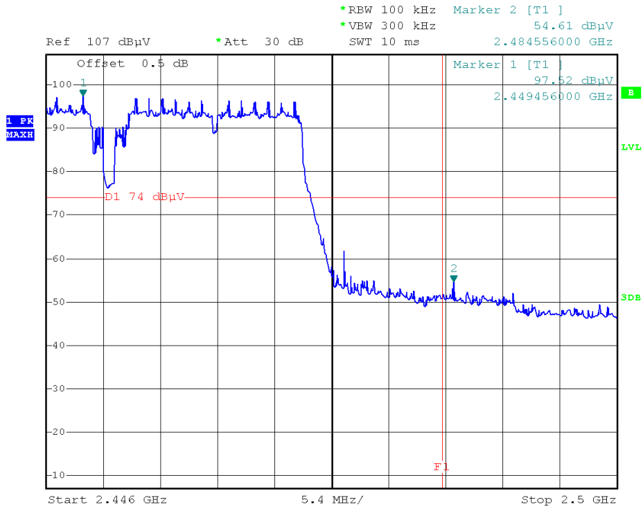
(Plot 2.6 D3: Channel = 9 Peak @ 802.11n-40)
