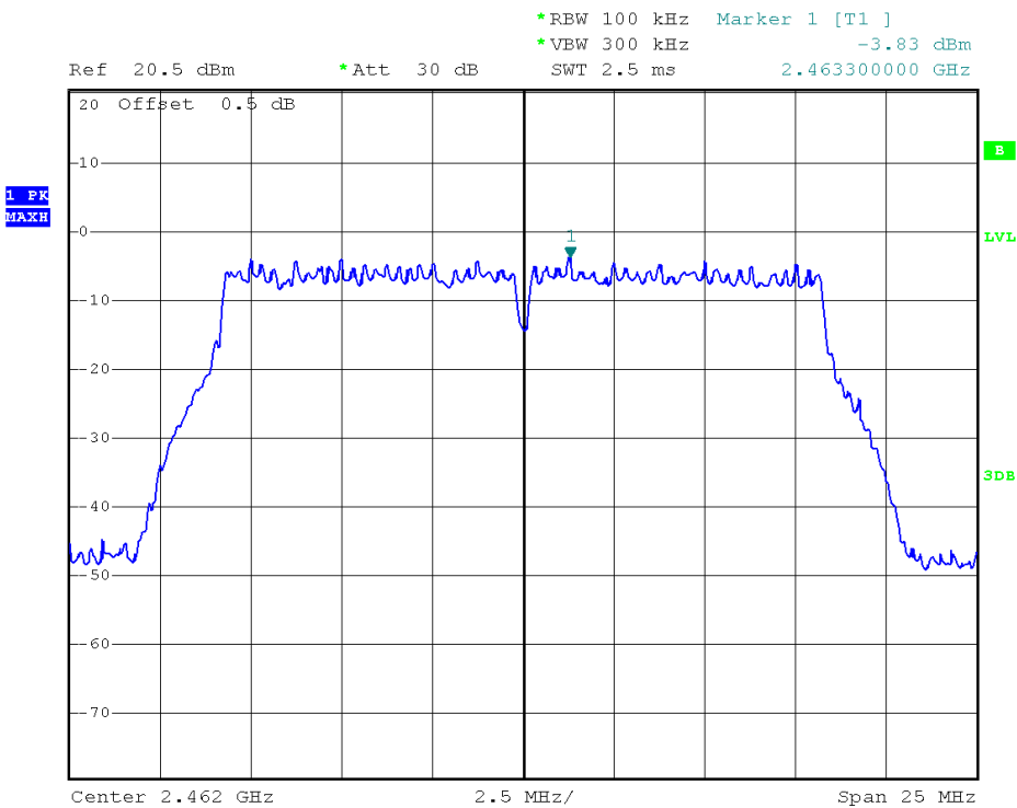
(Plot 2.5 F: Channel = 11 @ 802.11g)
