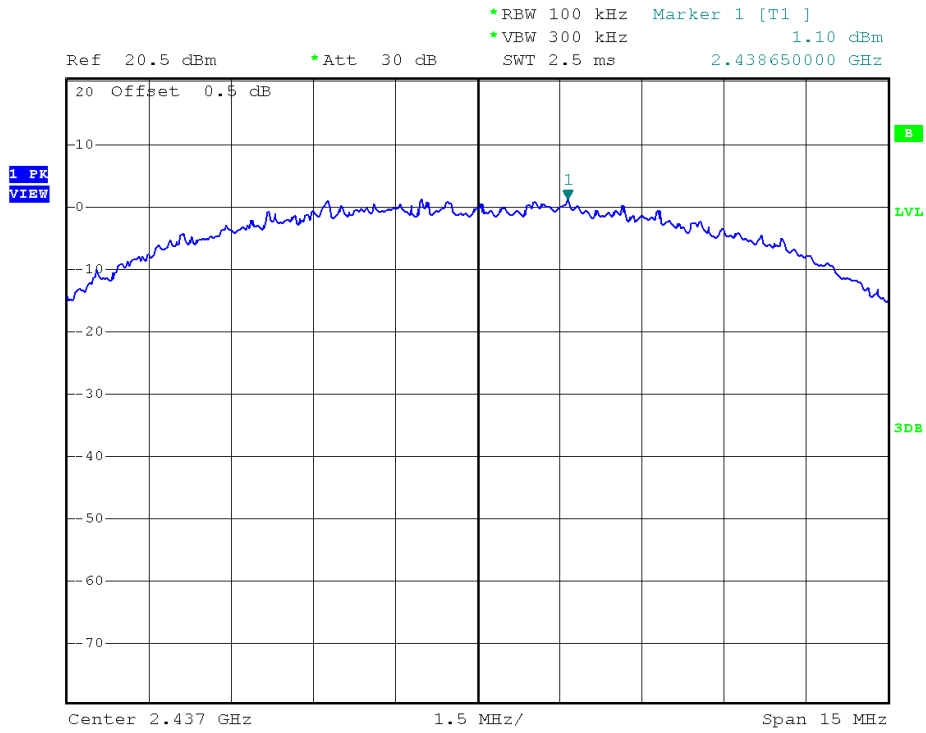
(Plot 2.5 B: Channel = 6 @ 802.11b)
