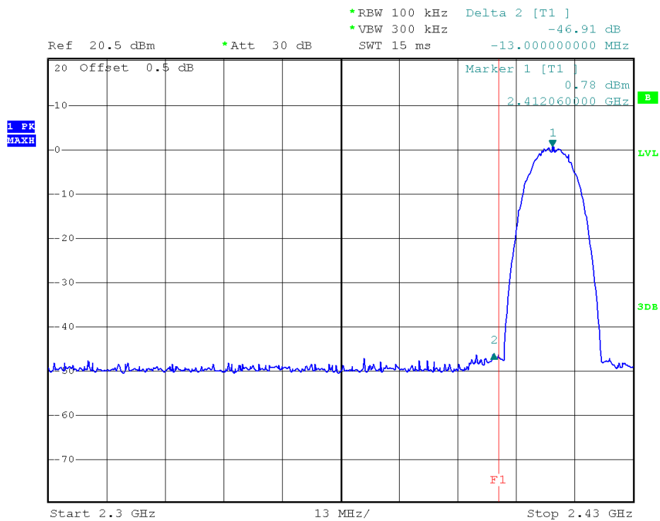
(Plot 2.6 E1: Channel =1 2412MHz @ 802.11b)
