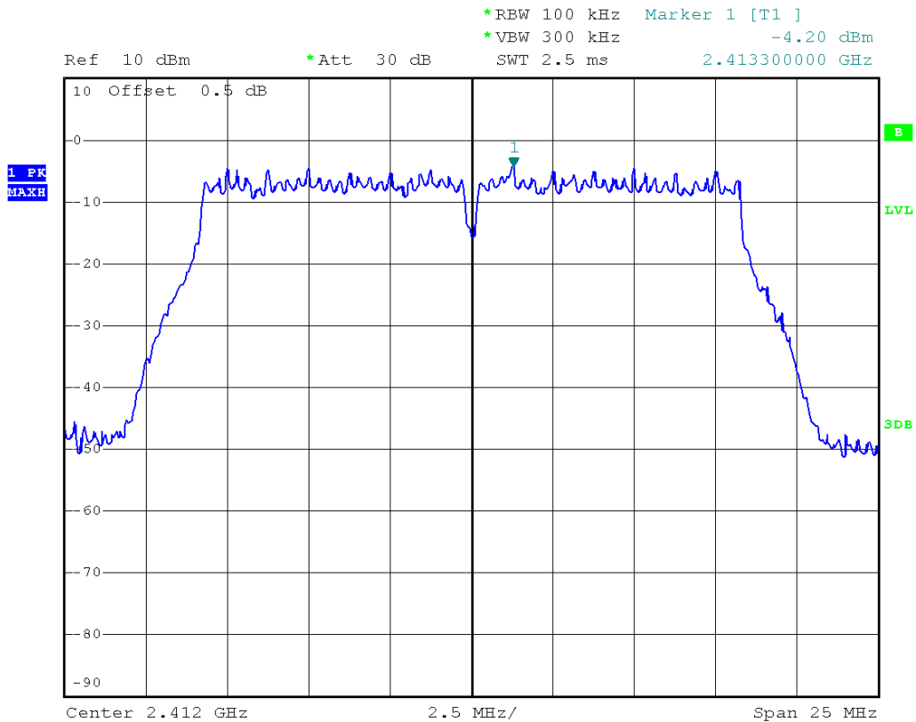
(Plot 2.5 D: Channel = 1 @ 802.11g)
