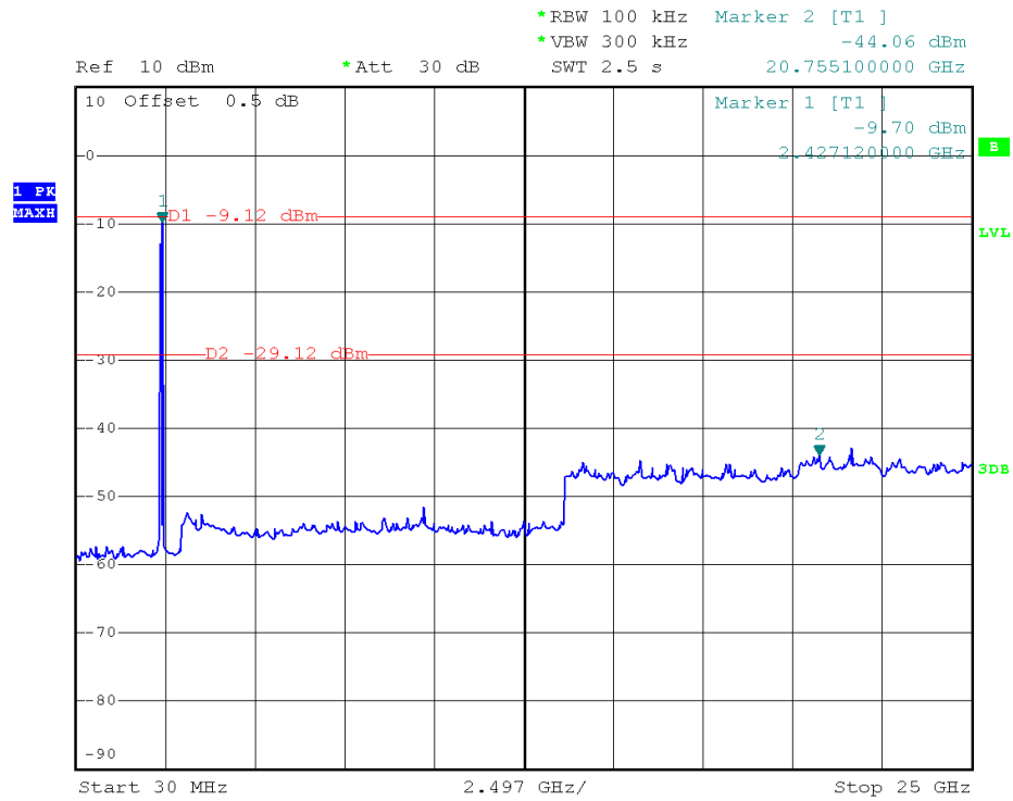
(Plot 2.4 K: Channel = 6, 30MHz to 25GHz@ 802.11n-40)
