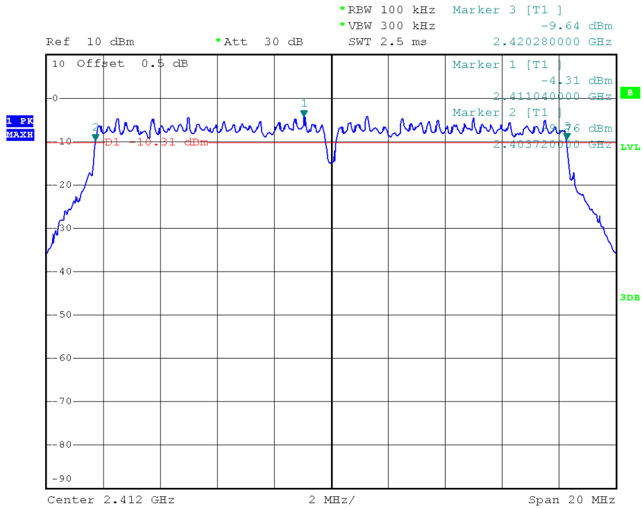
(Plot 2.3 D: Channel 1: 2412MHz @ 802.11g)
