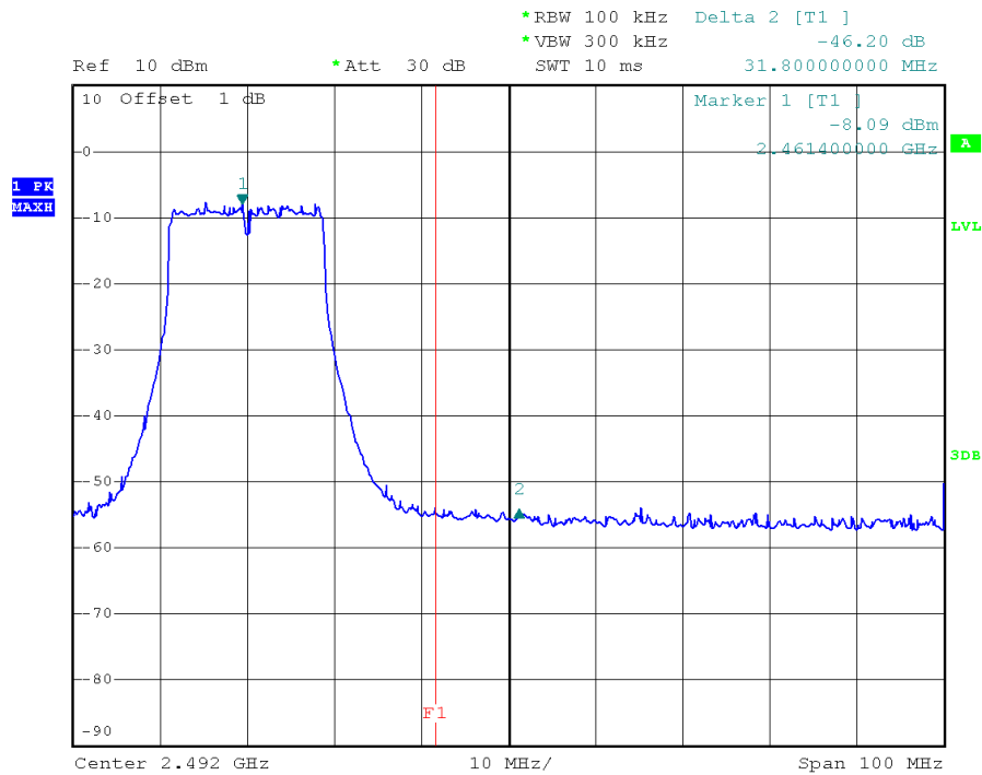
(Plot 2.6 G2: Channel =11 2462MHz @ 802.11n-20)
