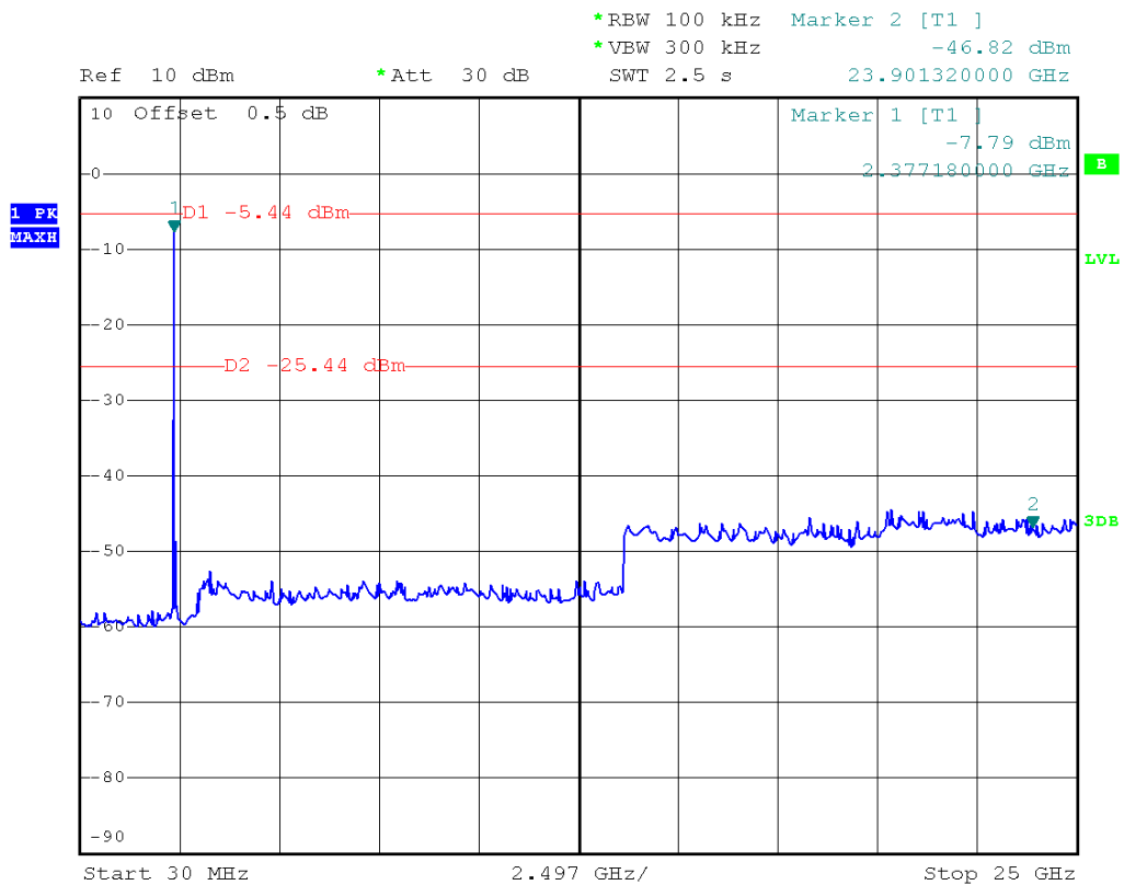
(Plot 2.4 G: Channel = 1, 30MHz to 25GHz@ 802.11n-20)
