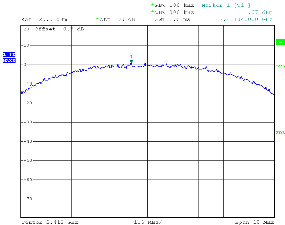
(Plot 2.5 A: Channel = 1 @ 802.11b)
