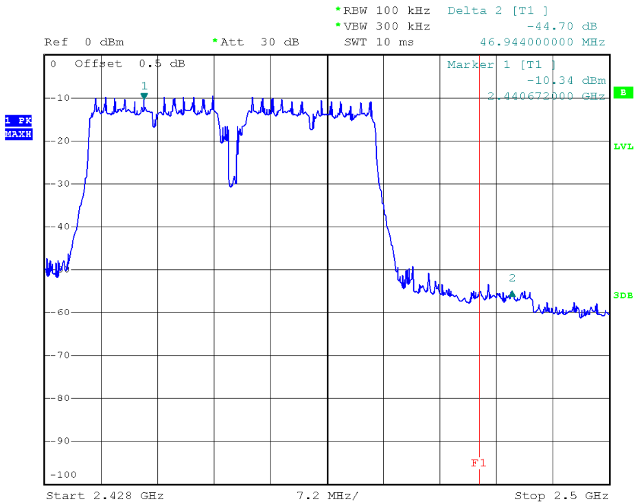
(Plot 2.6 H2: Channel =9 2452MHz @ 802.11n-40)
