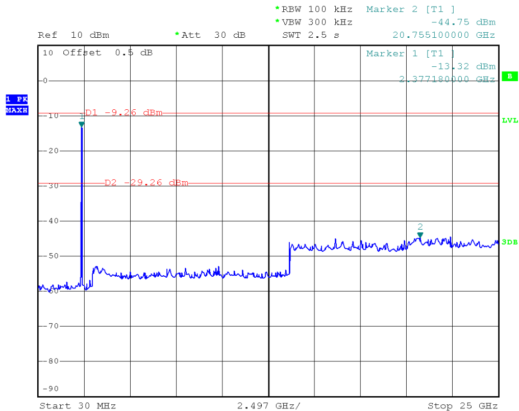
(Plot 2.4 J: Channel = 3, 30MHz to 25GHz@ 802.11n-40)
