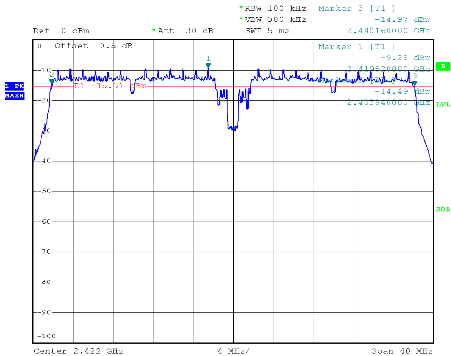
(Plot 2.3 J: Channel 3: 2422MHz @ 802.11n-40)
