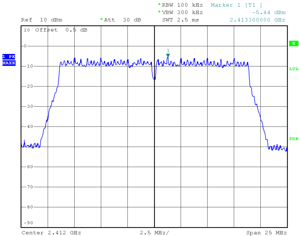
(Plot 2.5 G: Channel = 1 @ 802.11n-20)
