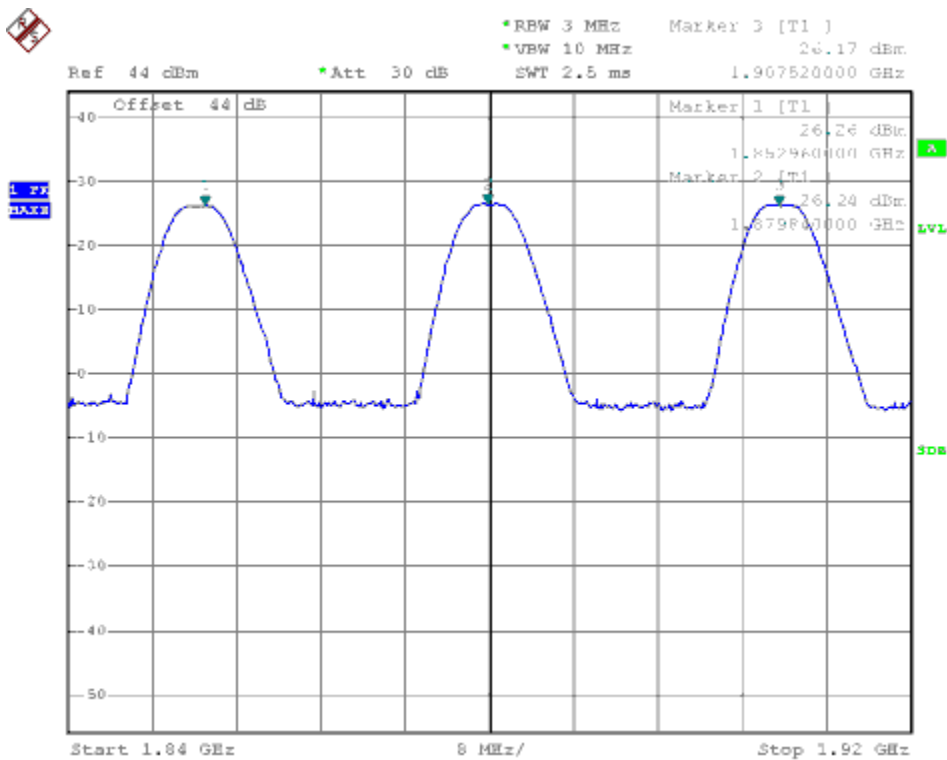
(Plot I: HSDPA 1900 MHz Channel = 9262, 9400, 9538)
