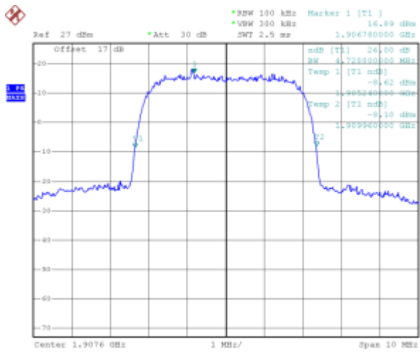
(Plot L: HSDPA 1900 MHz Channel = 9538)
