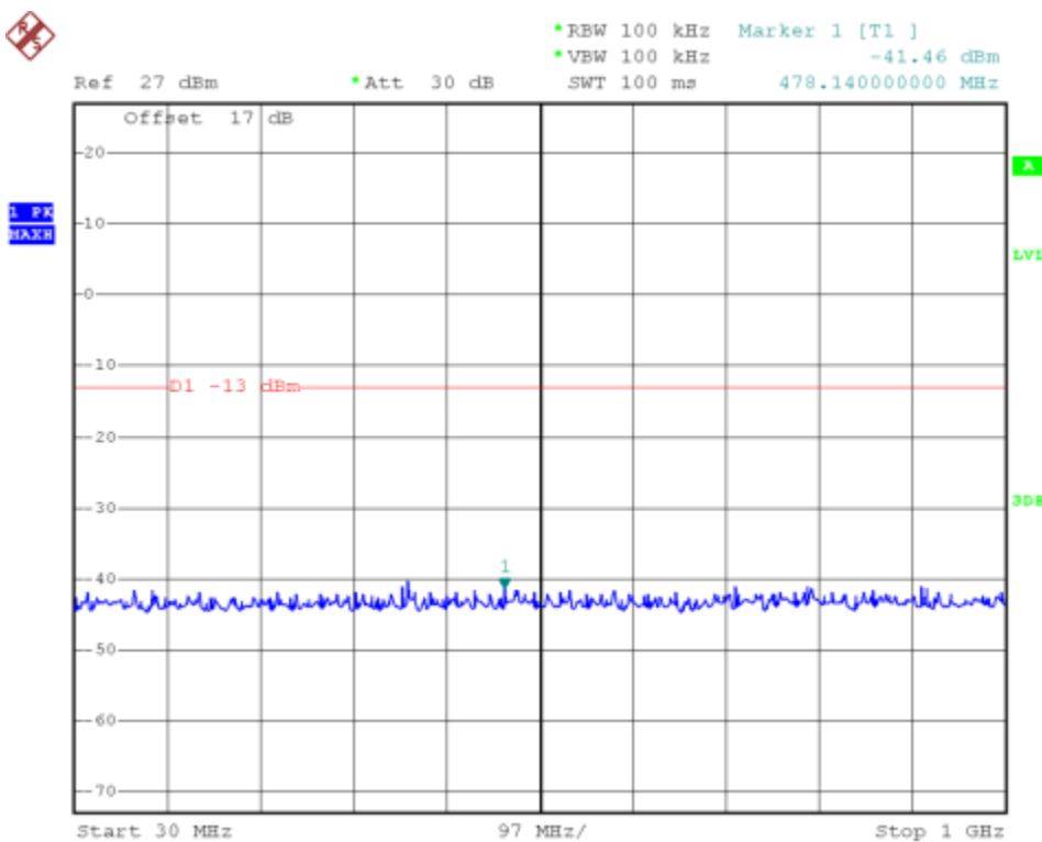
(Plot H3: HSUPA1900MHz Channel = 9538, 30MHz to 1GHz)
