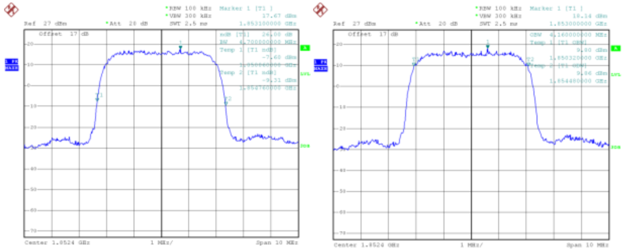
(Plot P: HSUPA1900 MHz Channel = 9262)
