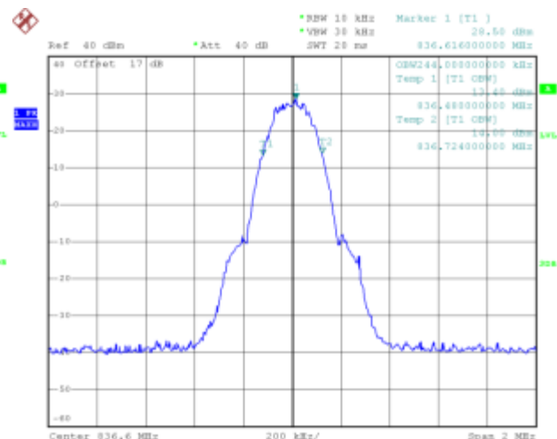
(Plot Z: GPRS 850MHz Channel = 190)
