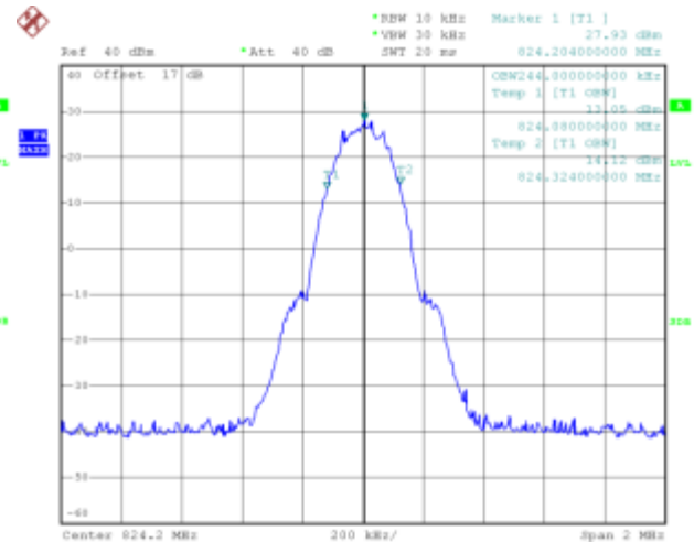
(Plot Y: GPRS 850MHz Channel = 128)
