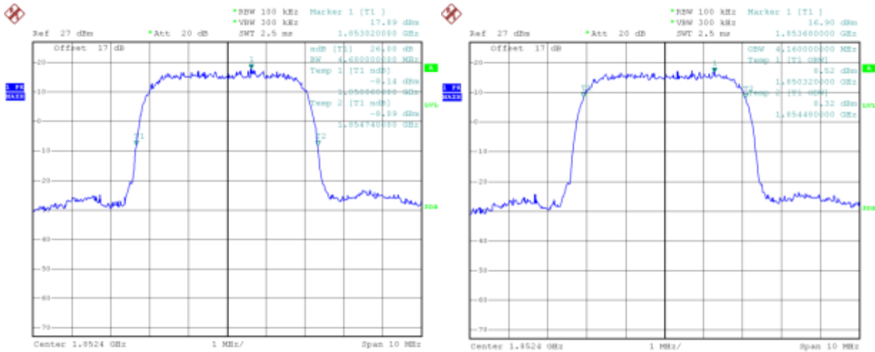
(Plot D: WCDMA 1900MHz Channel = 9262)
