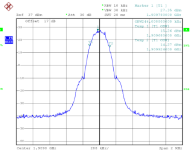
(Plot X: GSM 1900MHz Channel = 810)
