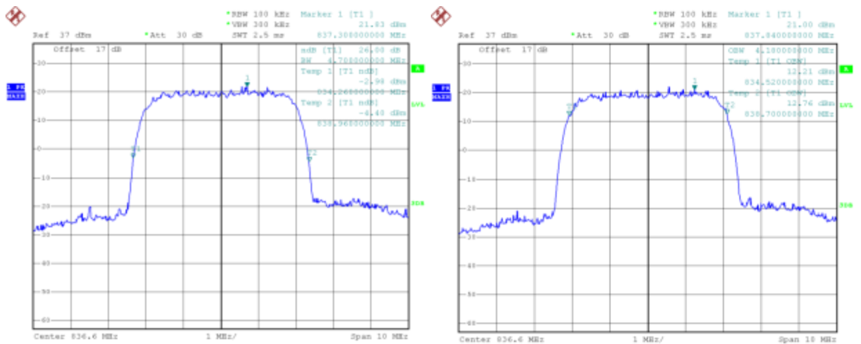
(Plot H: HSDPA 850 MHz Channel = 4183)
