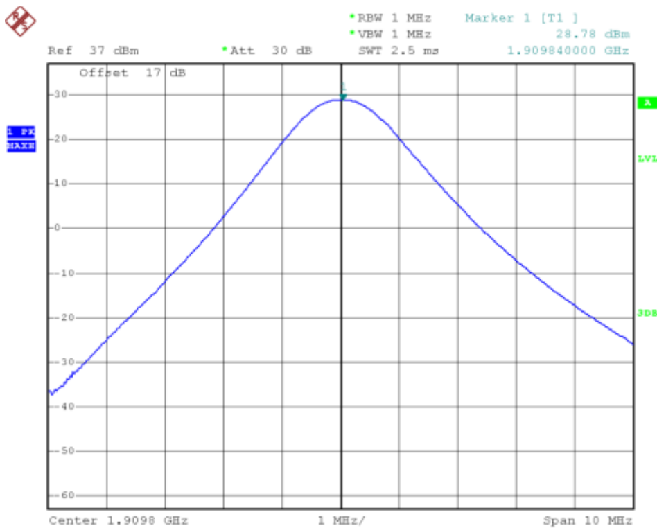
(Plot D3: GPRS 1900MHz Channel = 810)
