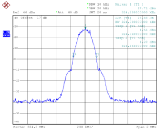
(Plot Y: GPRS 850MHz Channel = 128)
