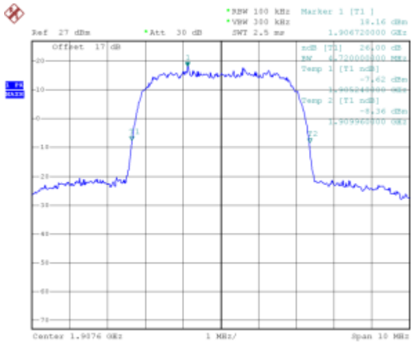
(Plot R: HSUPA1900 MHz Channel = 9538)
