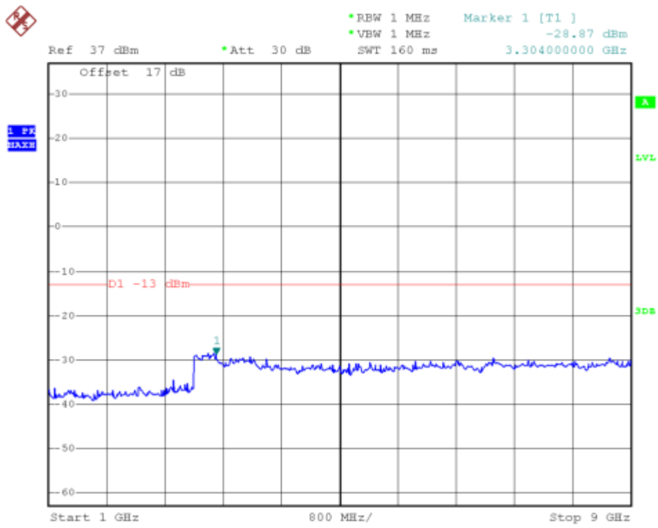
(Plot G2.1: HSUPA 850MHz Channel = 4183, 1GHz to 9GHz)
