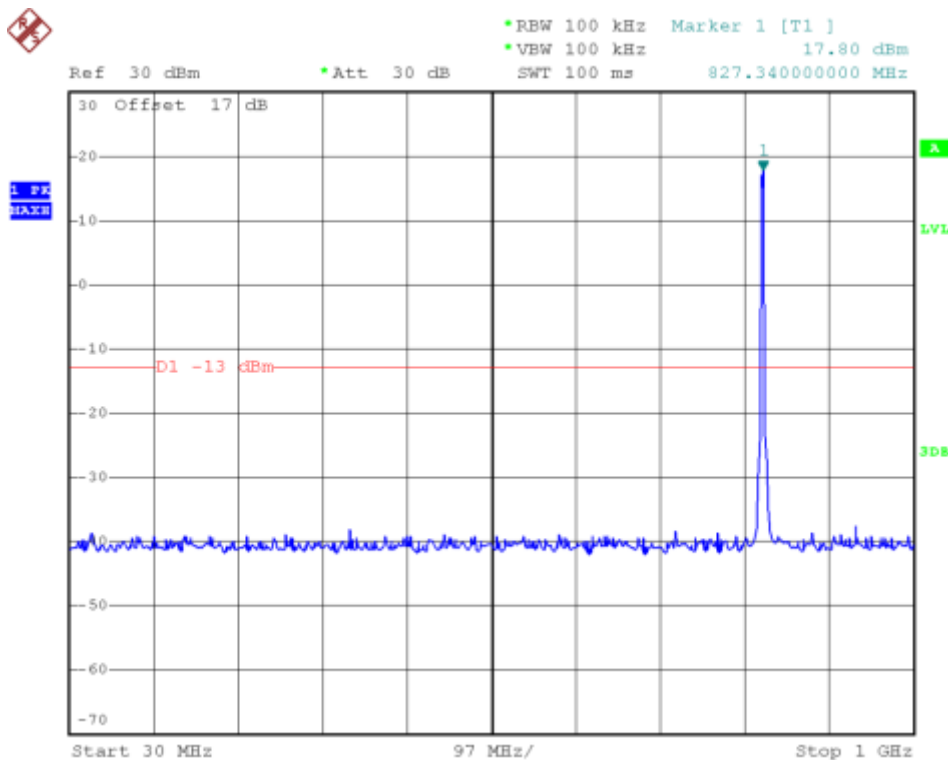
(Plot G 1: HSUPA 850MHz Channel = 4132, 30MHz to 1GHz)
