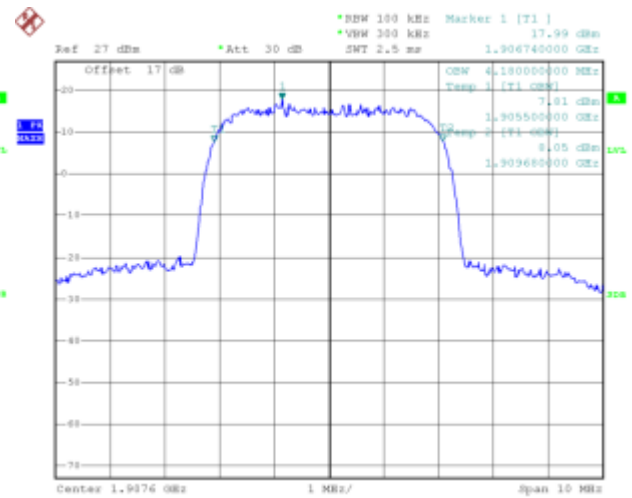
(Plot L: HSDPA 1900 MHz Channel = 9538)
