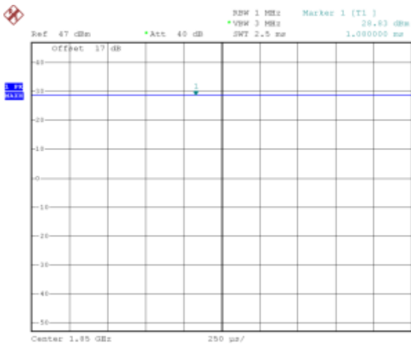
(Plot A1: GSM 1900 MHz Channel = 512)
