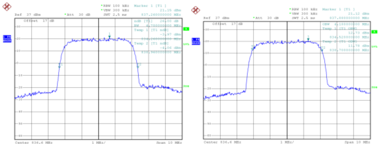
(Plot B: WCDMA 850 MHz Channel = 4183)
