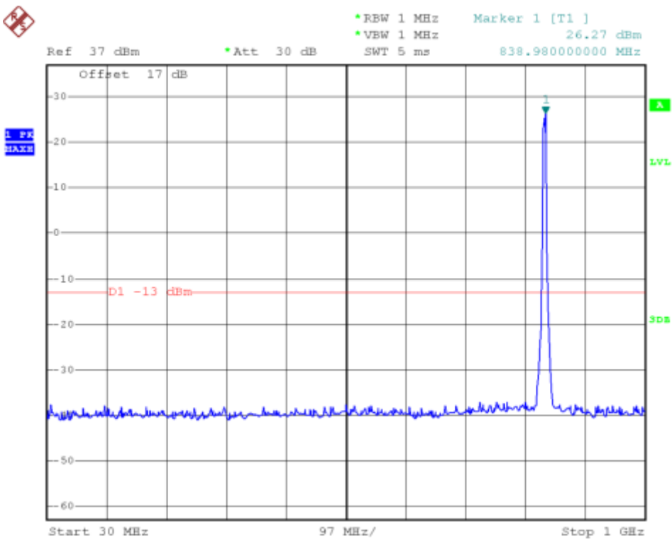
(Plot E2: HSDPA 850MHz Channel = 4183, 30MHz to 1GHz)
