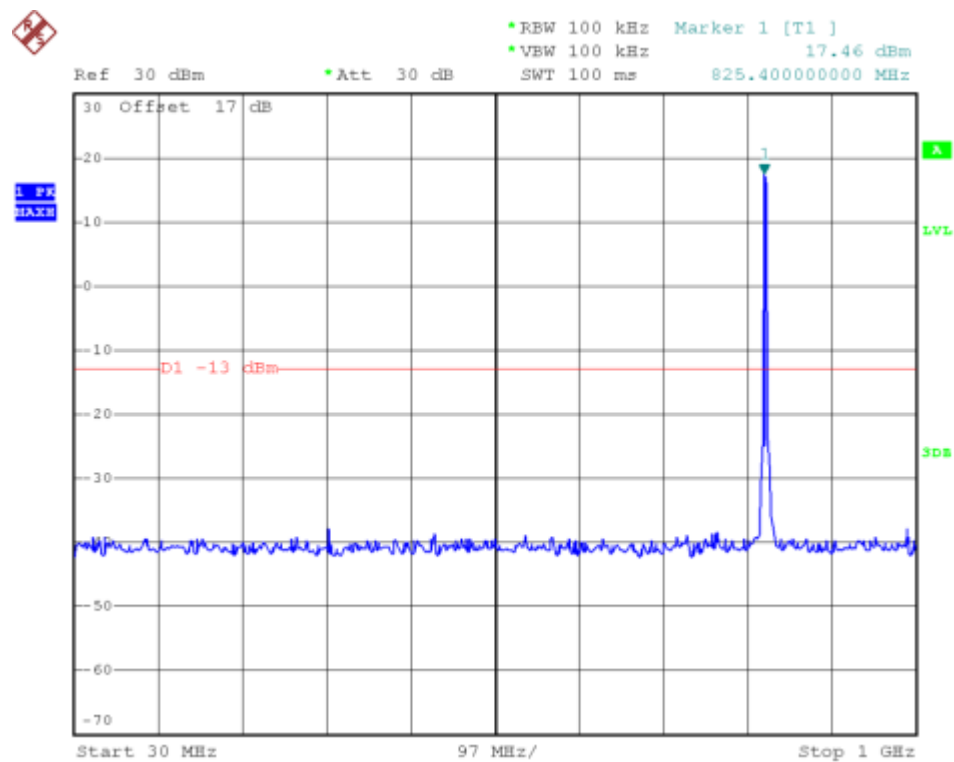
(Plot E1: HSDPA 850MHz Channel = 4132, 30MHz to 1GHz)
