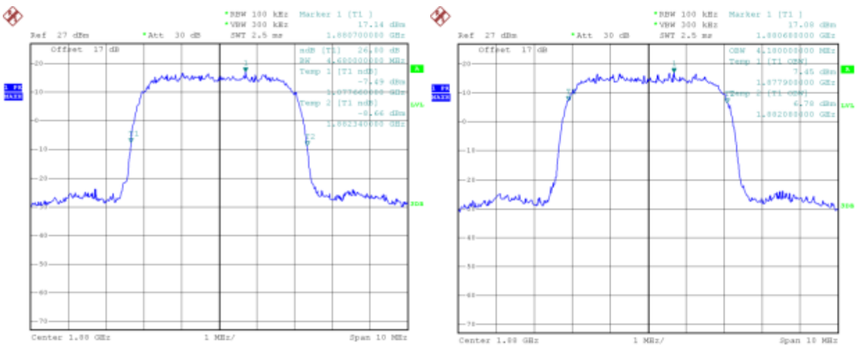
(Plot K: HSDPA 1900 MHz Channel = 9400)
