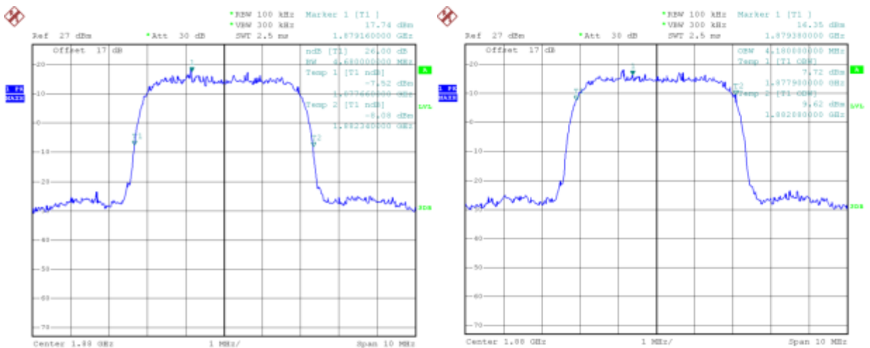
(Plot Q: HSUPA1900 MHz Channel = 9400)
