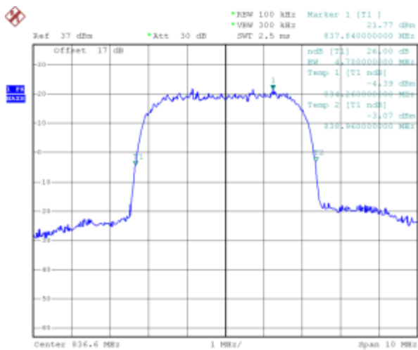
(Plot N: HSDPA 850 MHz Channel = 4183)
