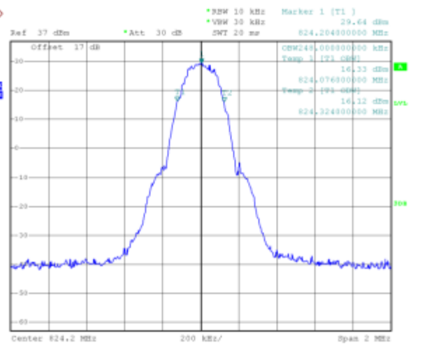
(Plot S: GSM 850MHz Channel = 128)
