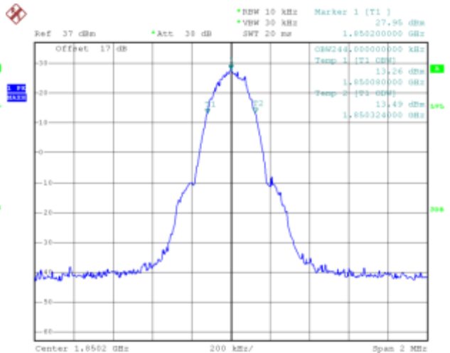
(Plot V: GSM 1900MHz Channel = 512)
