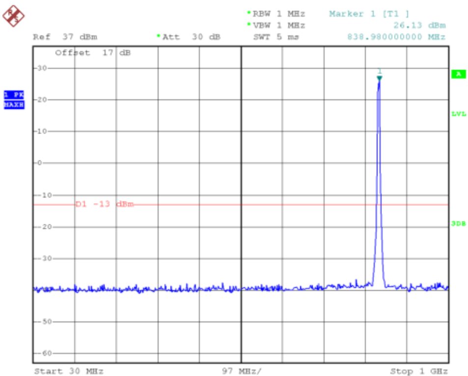
(Plot C2: WCDMA850MHz Channel = 4183, 30MHz to 1GHz)
