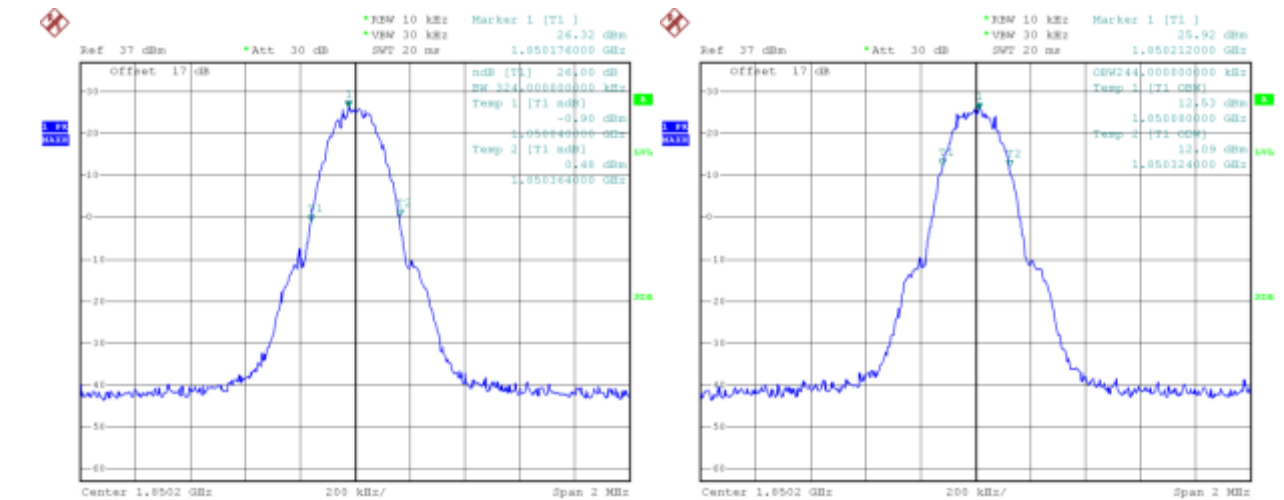
(Plot B1: GPRS 1900MHz Channel = 512)
