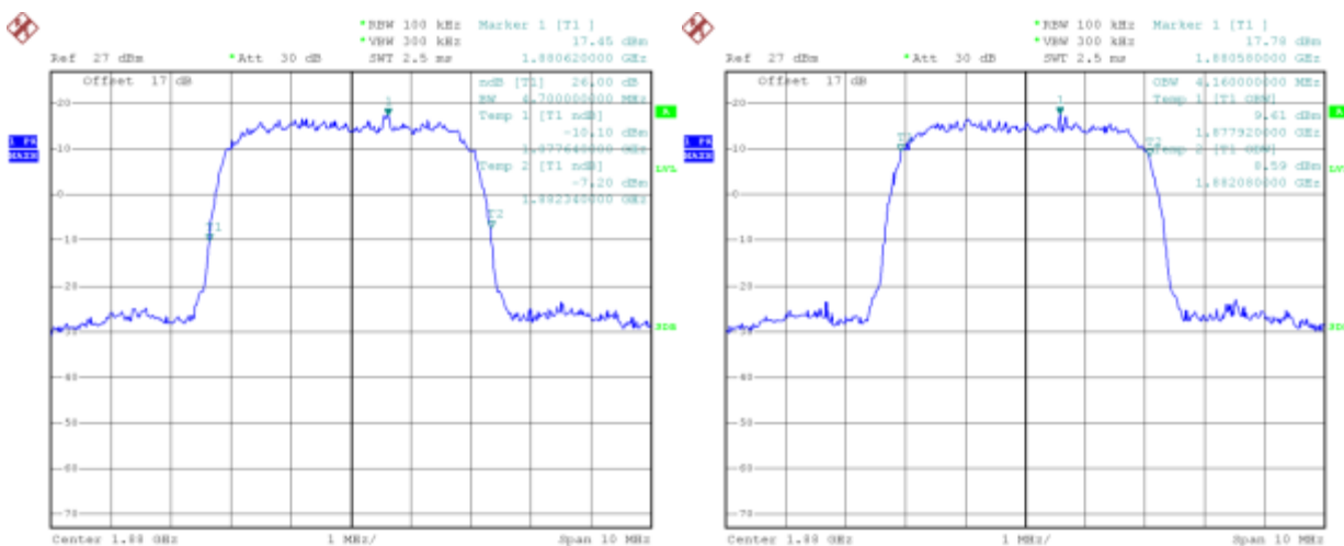
(Plot E: WCDMA 1900 MHz Channel = 9400)
