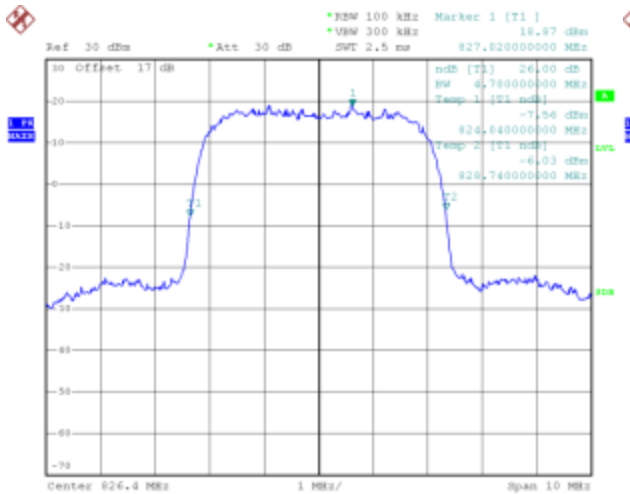
(Plot M: HSDPA 850 MHz Channel = 4132)
