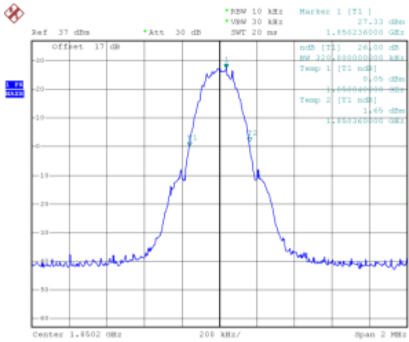
(Plot V: GSM 1900MHz Channel = 512)
