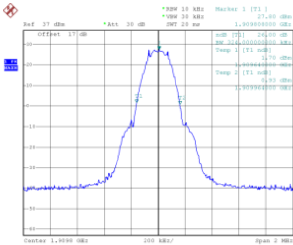
(Plot X: GSM 1900MHz Channel = 810)
