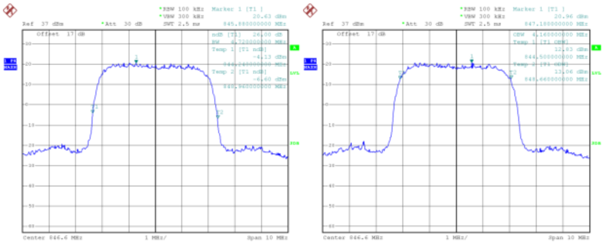
(Plot O: HSUPA850 MHz Channel = 4233)
