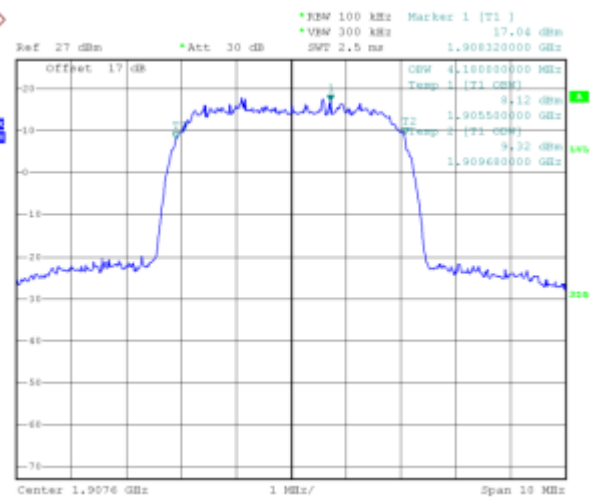
(Plot R: HSUPA1900 MHz Channel = 9538)
