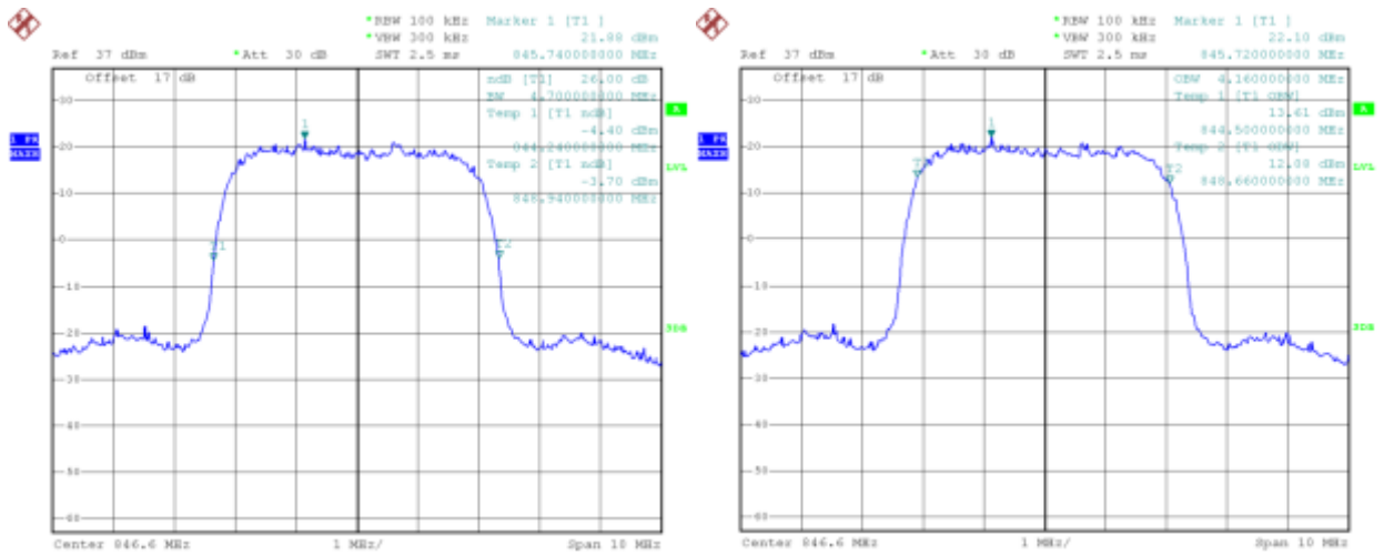
(Plot C: WCDMA 850MHz Channel = 4233)
