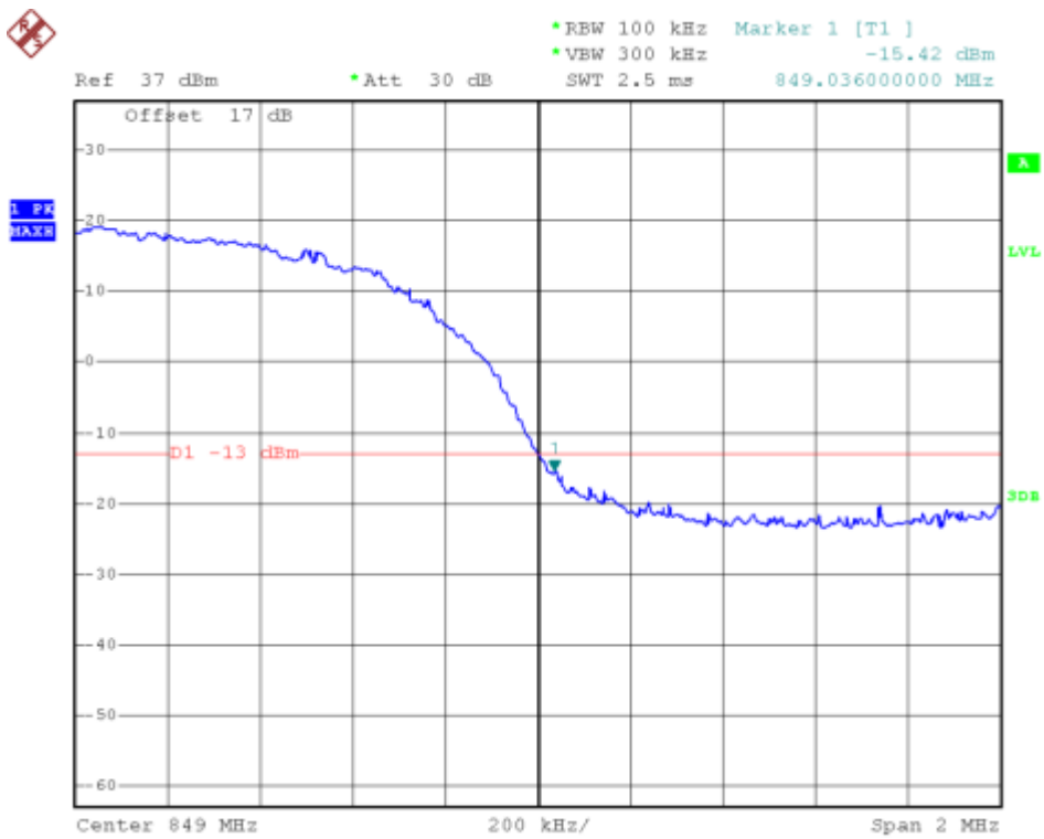
(Plot J: HSDPA850 Channel = 4233)
