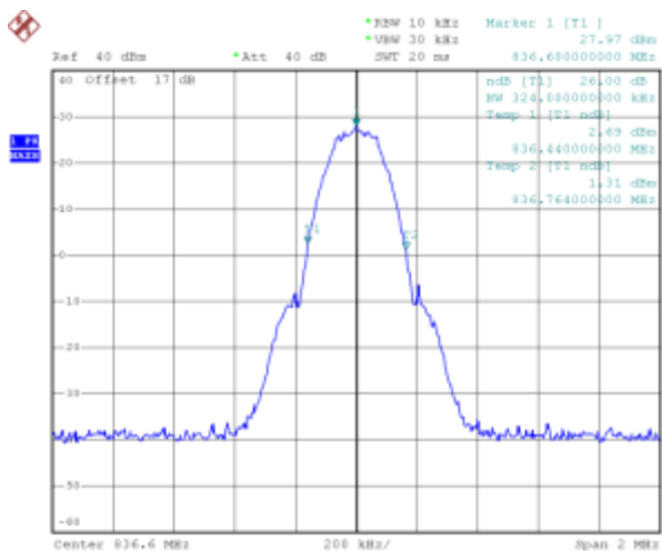
(Plot Z: GPRS 850MHz Channel = 190)
