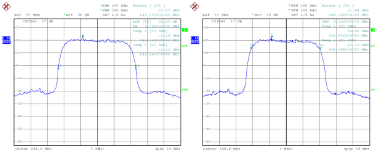
(Plot I: HSDPA 850 MHz Channel = 4233)
