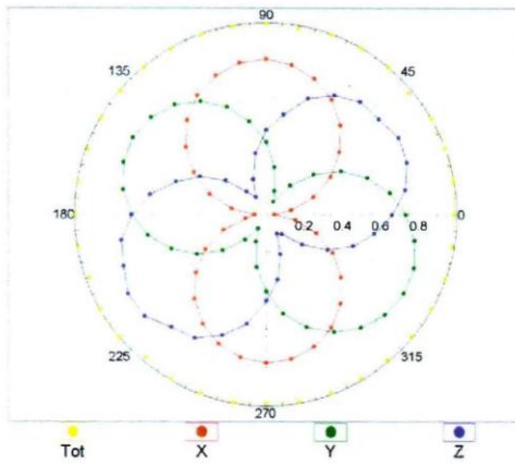
f=600 MHz,TEM
