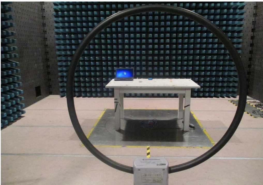
Radiated Emission Test setup photos
