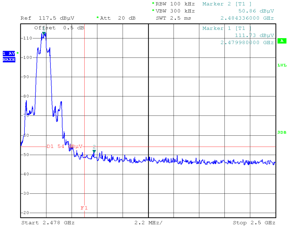
(Plot D2: Channel = 78 AVERAGE @π /4-DQPSK)
