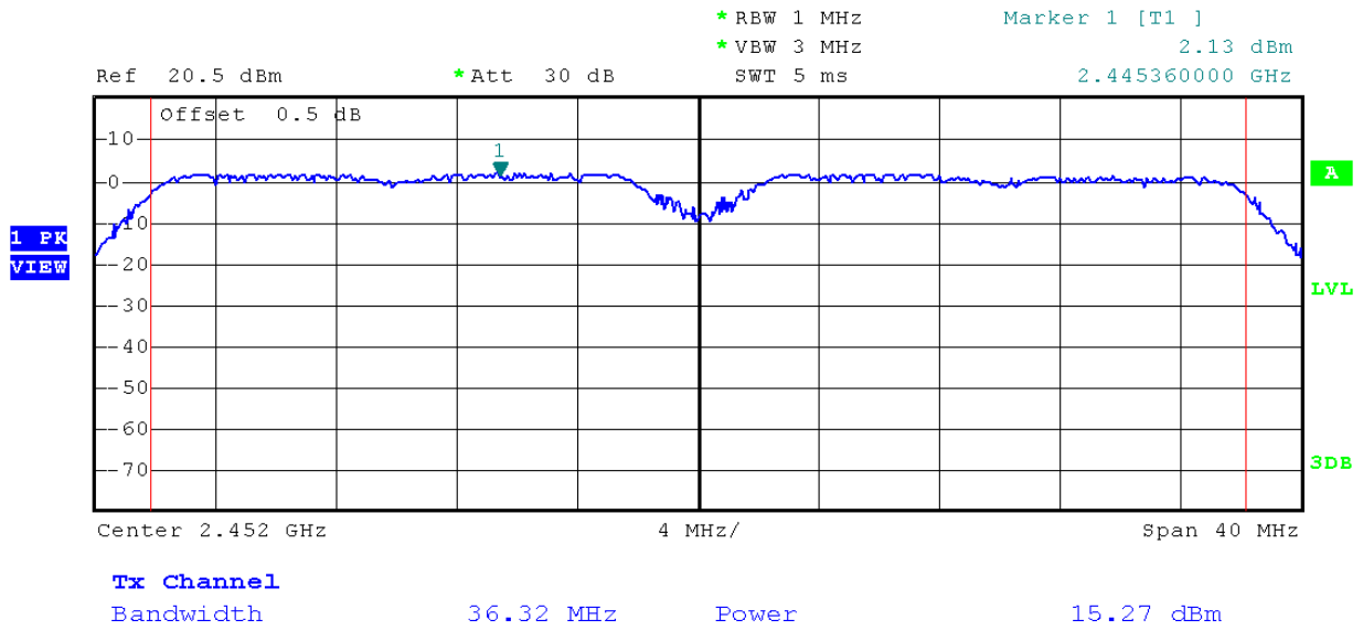
(Plot 2.2 L: Channel 9: 2452MHz @ 802.11n40)
