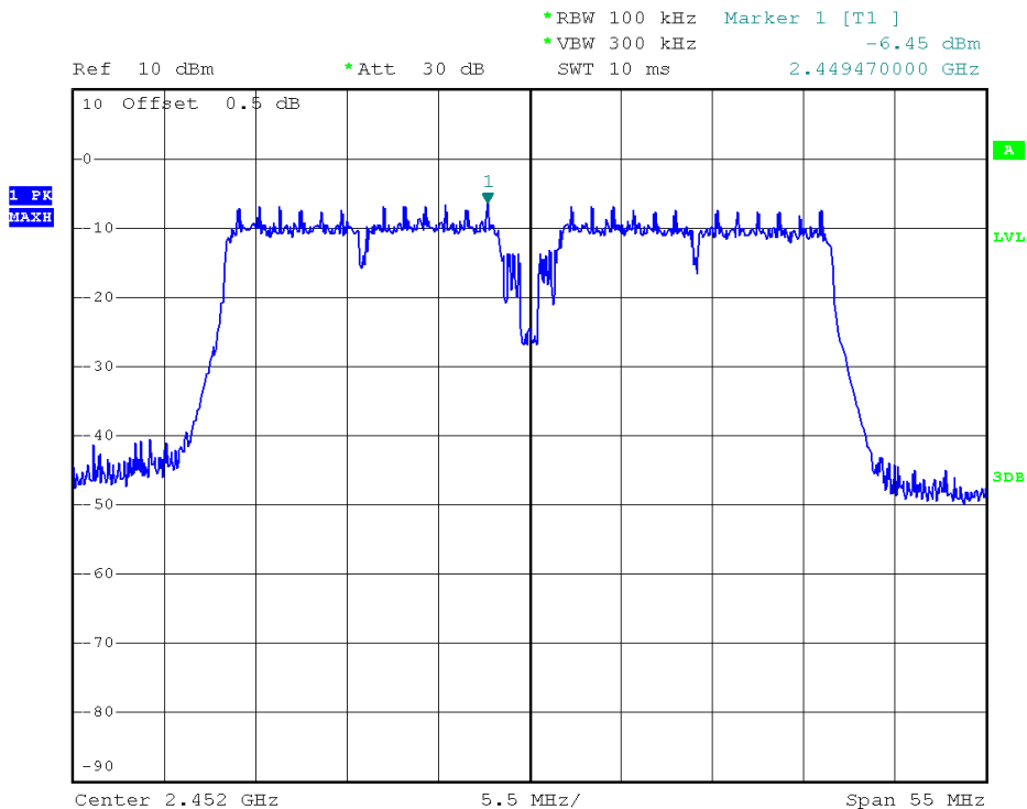
(Plot 2.5 L: Channel = 9 @ 802.11n-40)
