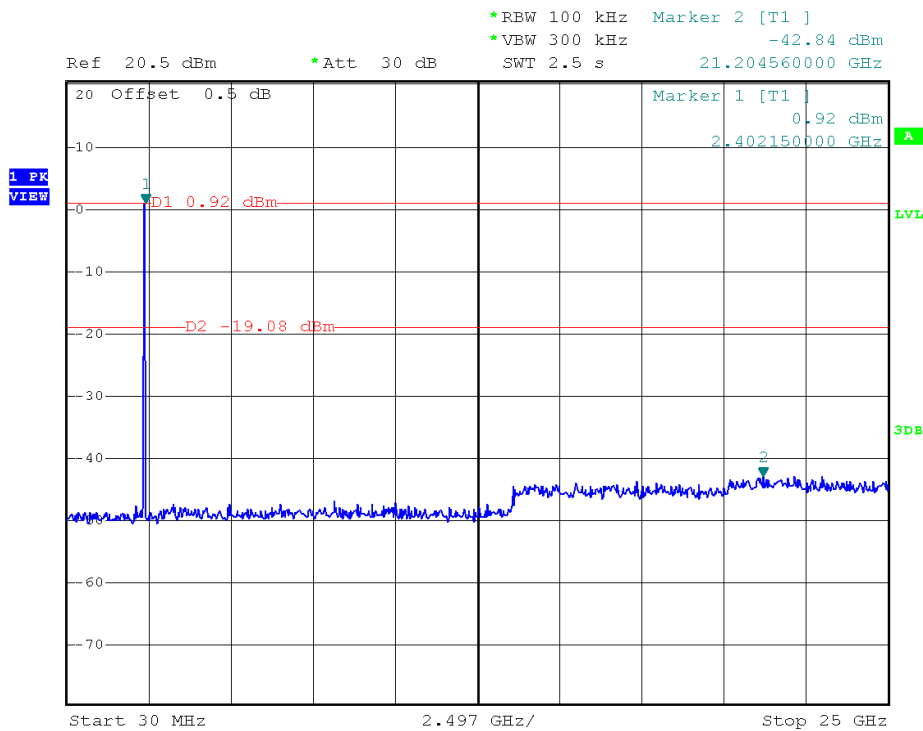
(Plot 2.4 A: Channel = 1, 30MHz to 25GHz@ 802.11b)
