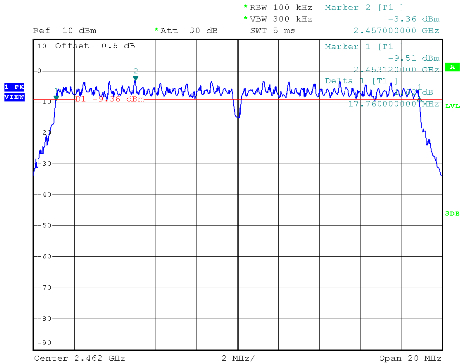
(Plot 2.3 I: Channel 11: 2462MHz @ 802.11n-20)
