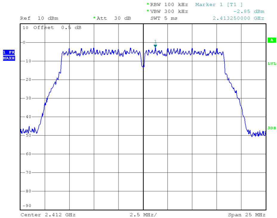
(Plot 2.5 D: Channel = 1 @ 802.11g)
