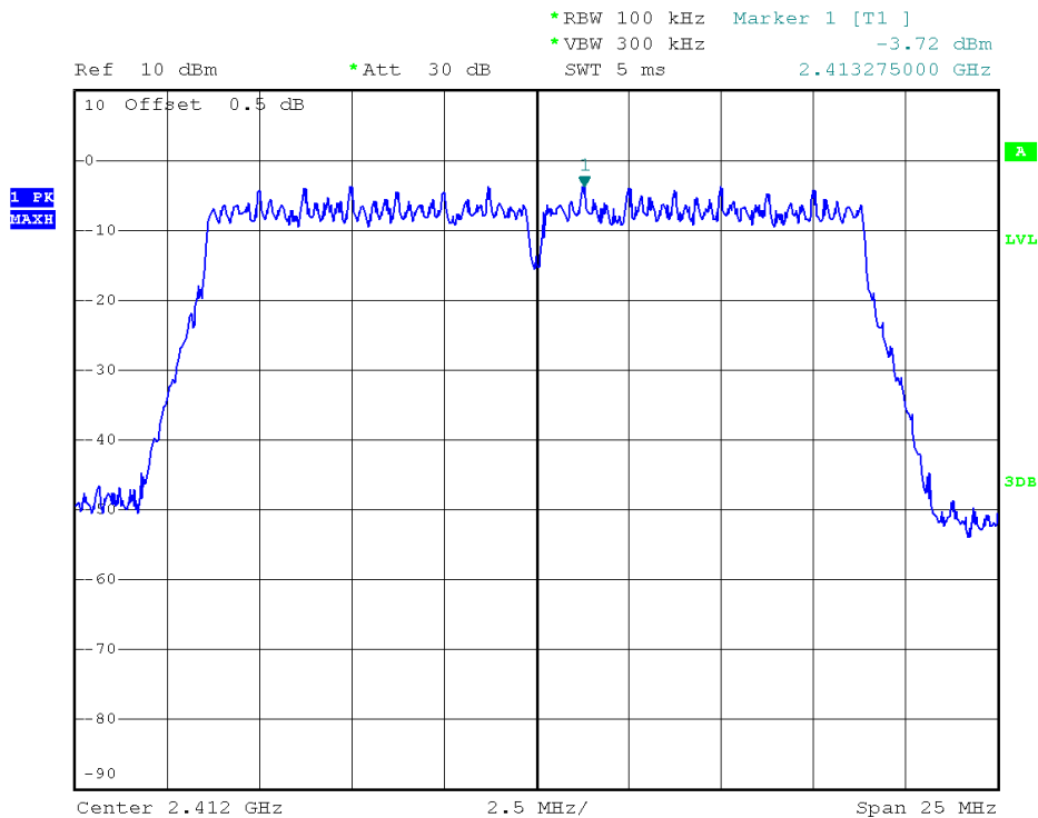
(Plot 2.5 G: Channel = 1 @ 802.11n-20)
