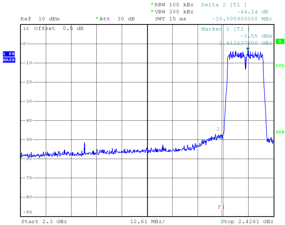
(Plot 2.6 G1: Channel =1 2412MHz @ 802.11n-20)
