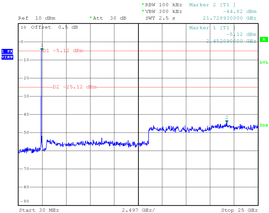
(Plot 2.4 F: Channel = 11, 30MHz to 25GHz @ 802.11g)
