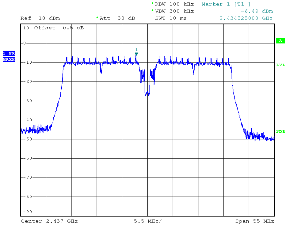
(Plot 2.5 K: Channel = 6 @ 802.11n-40)
