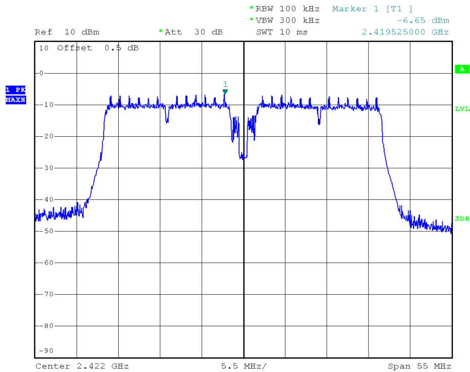
(Plot 2.5 J: Channel = 3 @ 802.11n-40)
