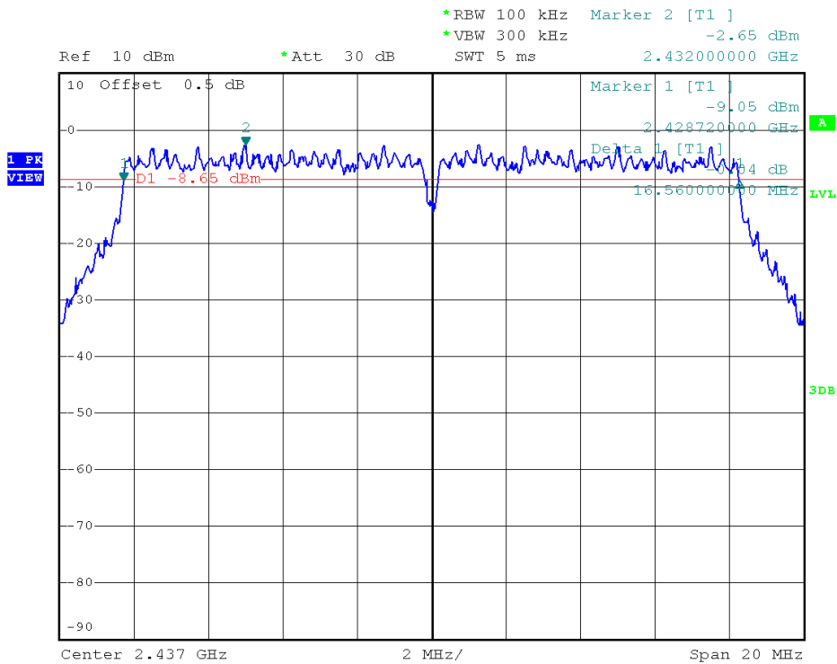
(Plot 2.3 E: Channel 6: 2437MHz @ 802.11g)
