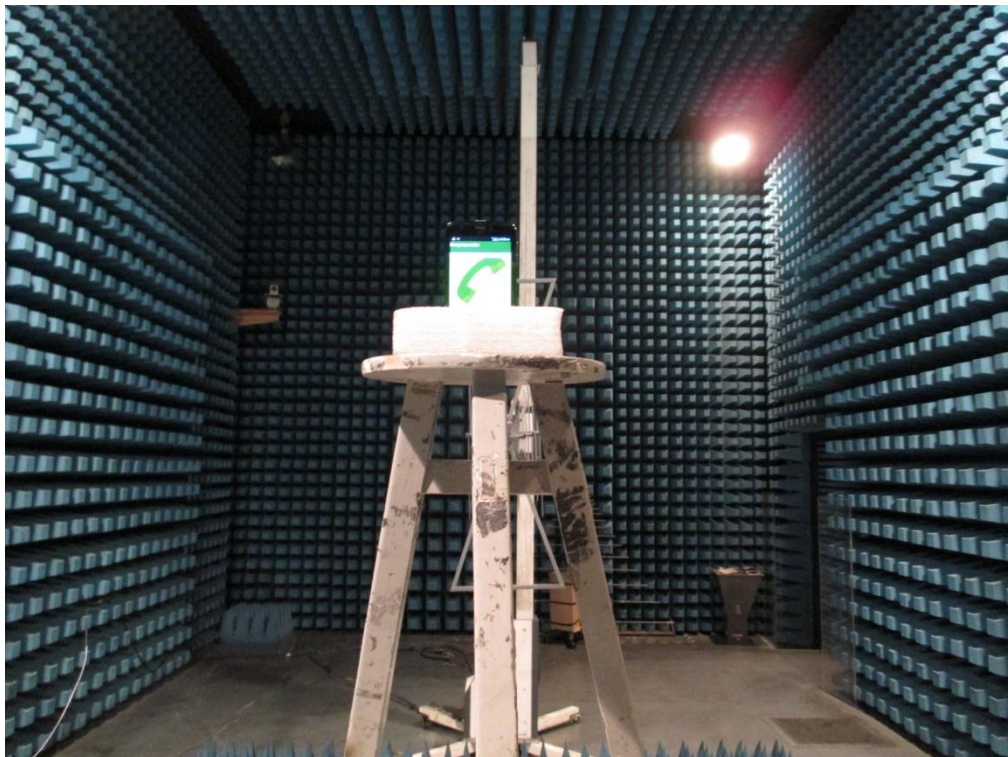
Radiated Test setup photos
