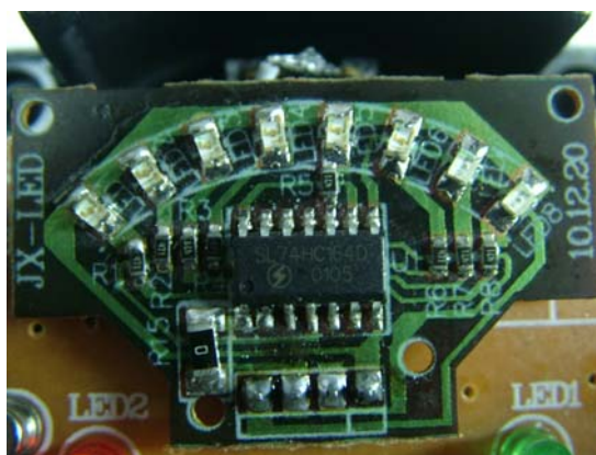
PCB Layout-5
