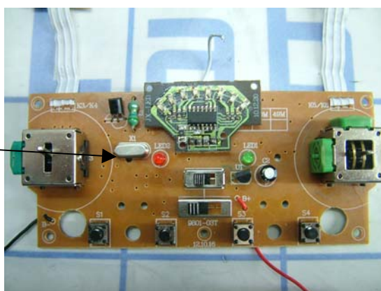
PCB Layout-1
