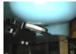
Figure 18. Head SAR Test Setup
