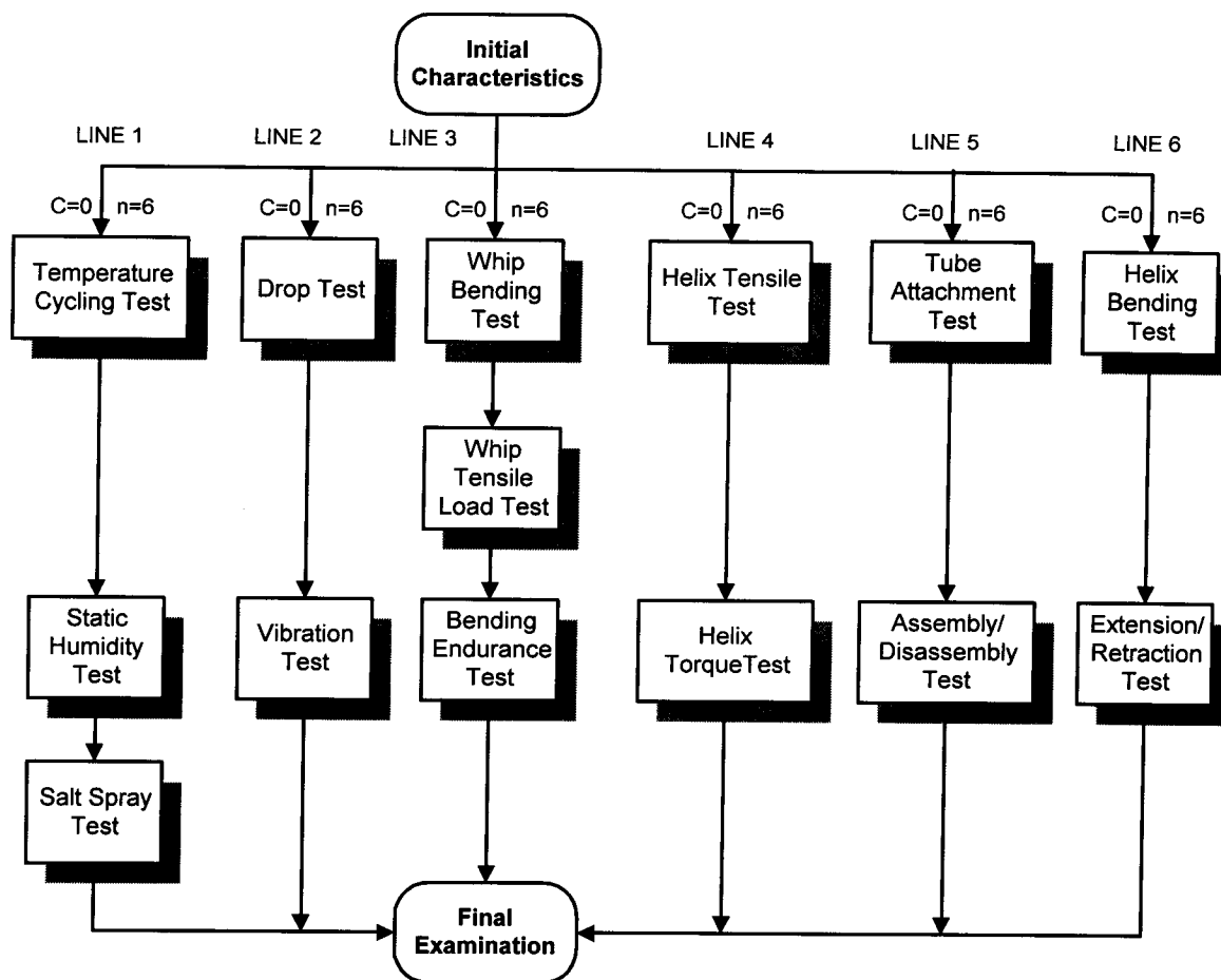
Figure 5. Qualification Flow Chart
