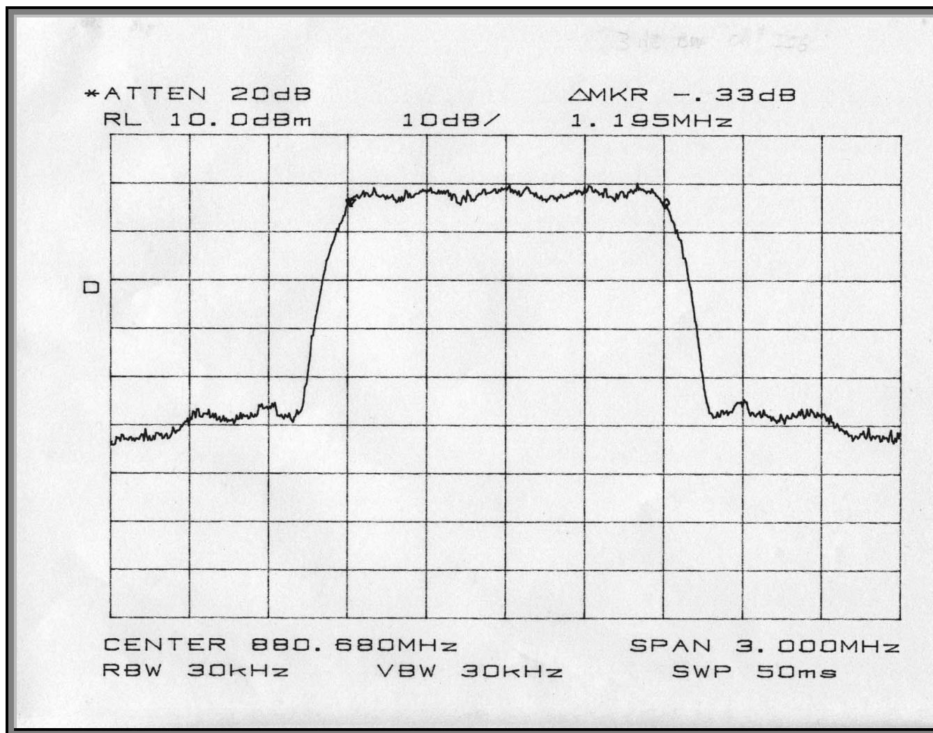
Channel 356 3 dB Bandwidth
