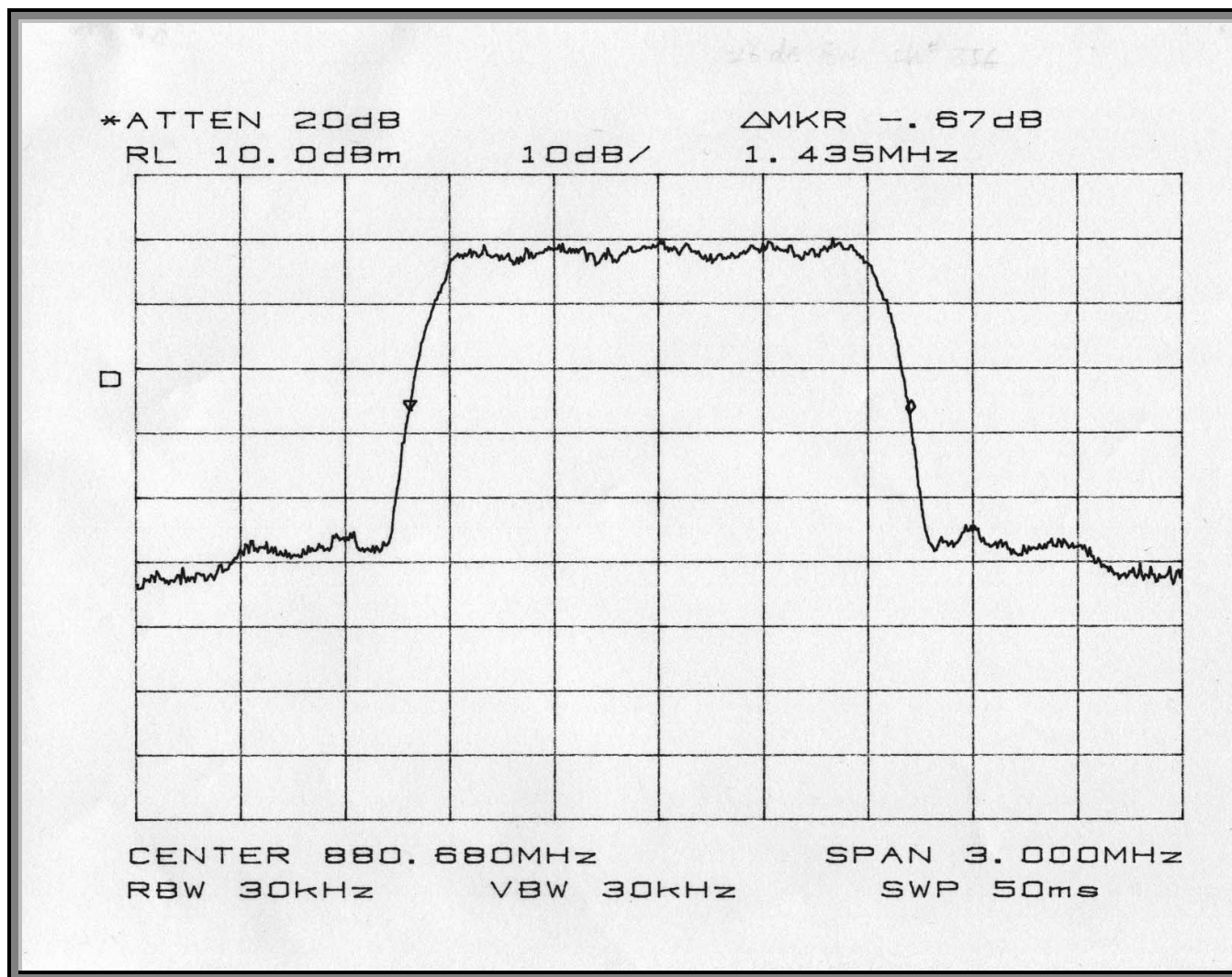
Channel 356 26 dB Bandwidth
