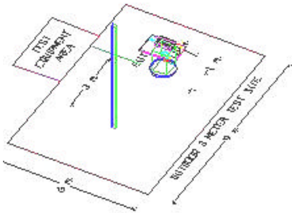
Figure 2. Outdoor 3-meter test site
