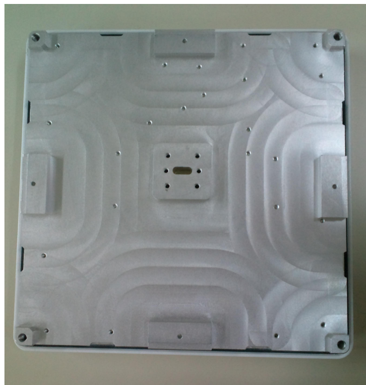
rear side (without antenna)
