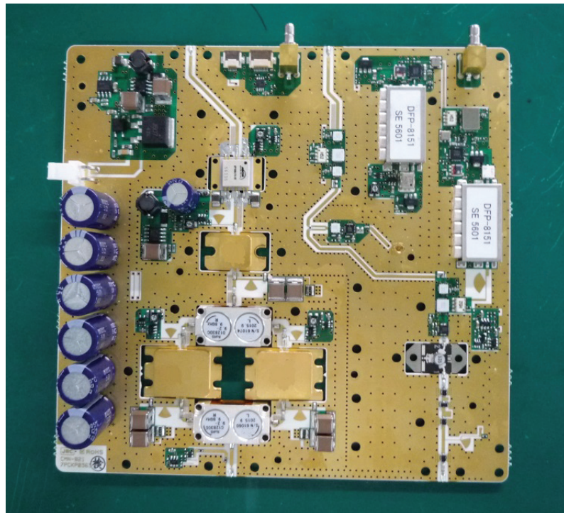
Inside View of TRX Module(Part Side)
