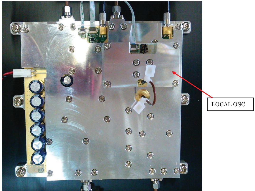
TRX MODULE Top view and LOCAL OSC Top view
