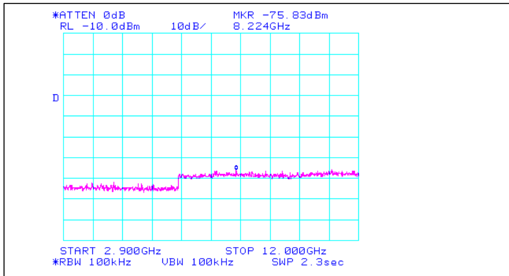
Plot 11. Radiated Spurious Emissions, Test Results (2.9GHz - 12.0GHz)
