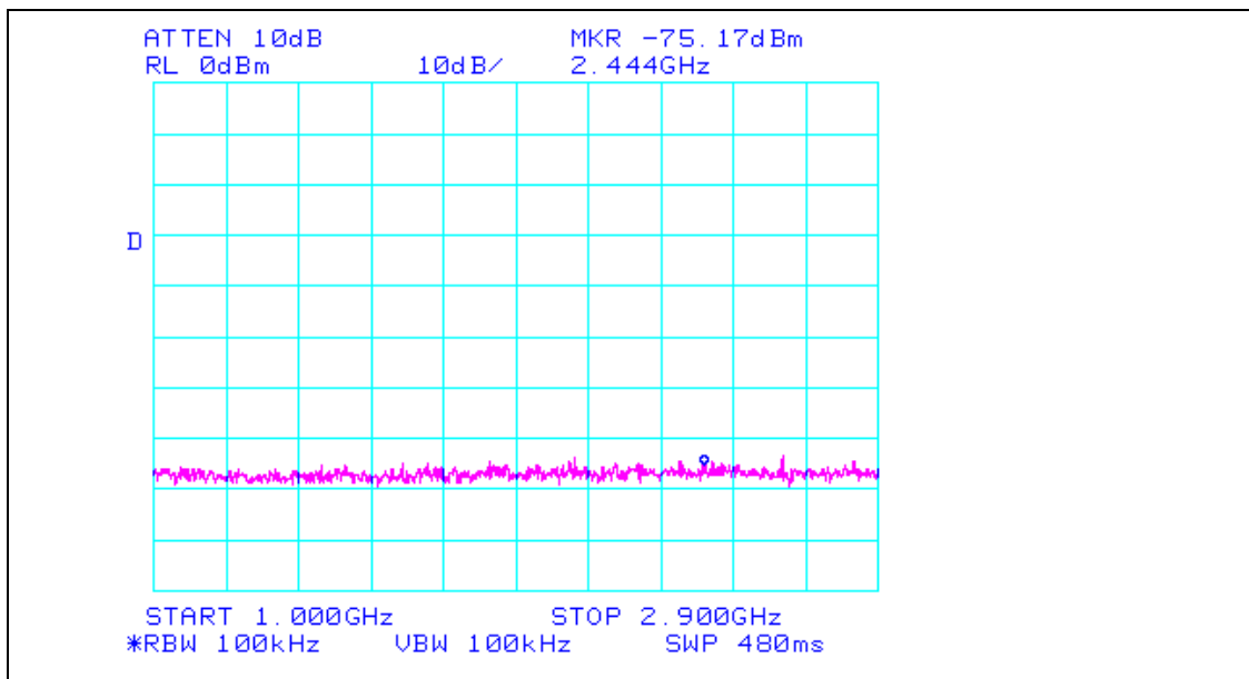
Plot 7. Conducted Spurious Emissions, Test Results (1GHz - 2.9GHz)
