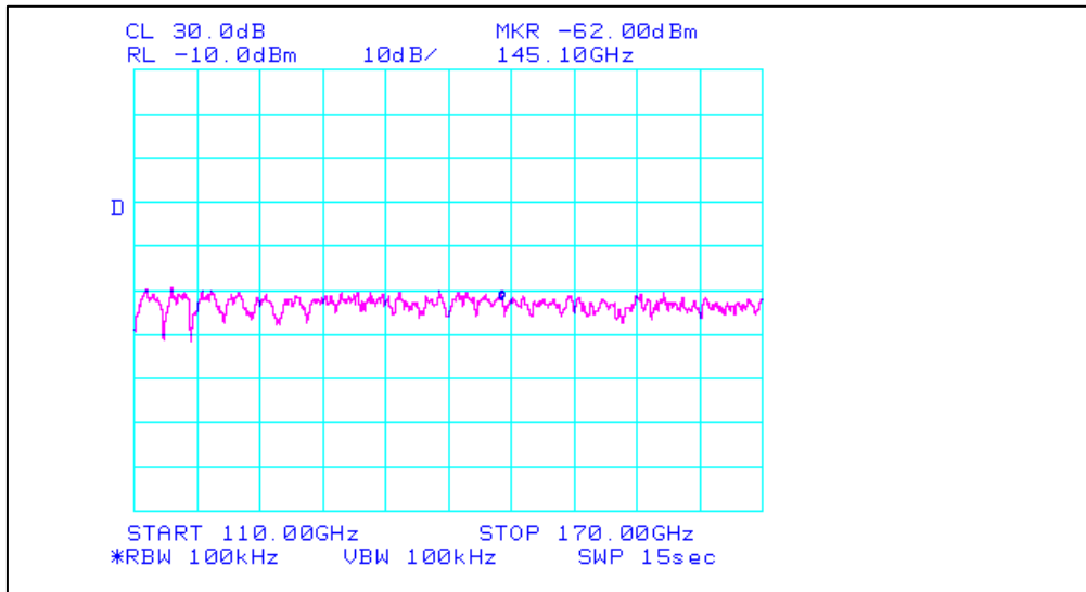
Plot 17. Radiated Spurious Emissions, Test Results (110.0GHz - 170.0GHz)
