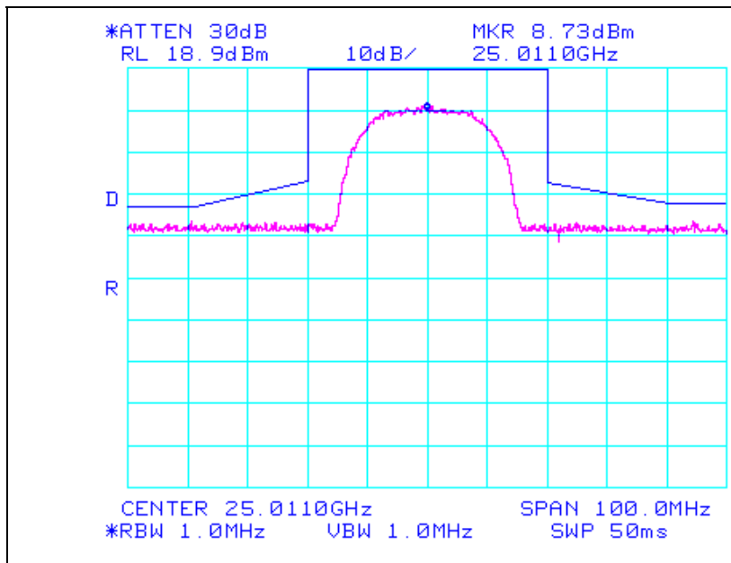
Plot 3. Emission Limitation Test Results (QPSK)
