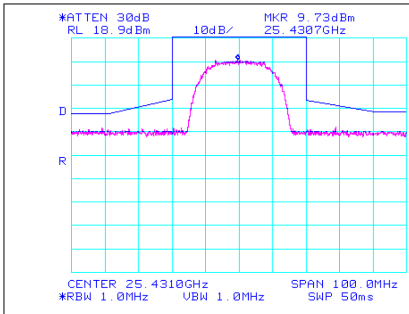
Plot 5. Emission Limitation Test Results (QPSK)
