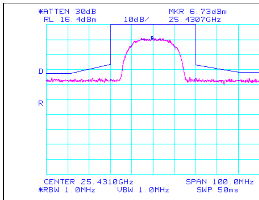
Plot 6. Emission Limitation Test Results (16QAM)
