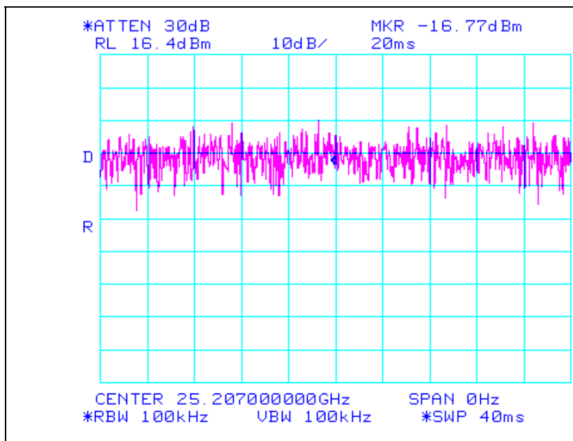
Plot 24. Modulation Test Results (16QAM)
