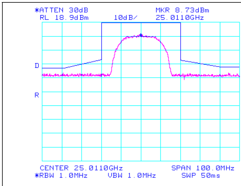
Plot 21. Emission Limitation Test Results (QPSK)
