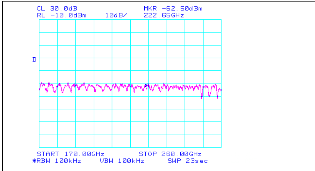
Plot 18. Radiated Spurious Emissions, Test Results (170.0GHz - 260.0GHz)
