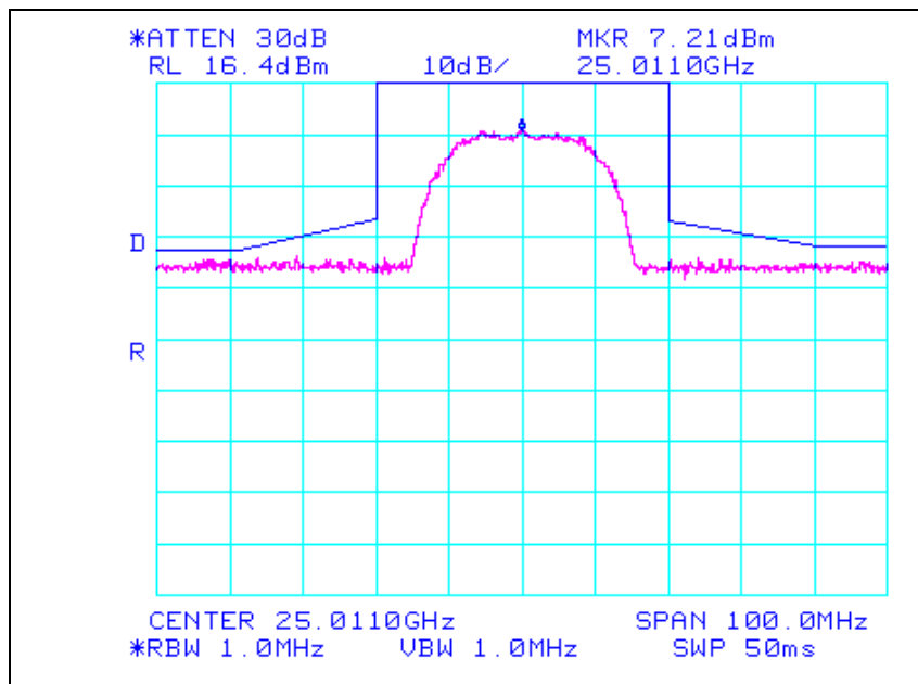
Plot 4. Emission Limitation Test Results (16QAM)
