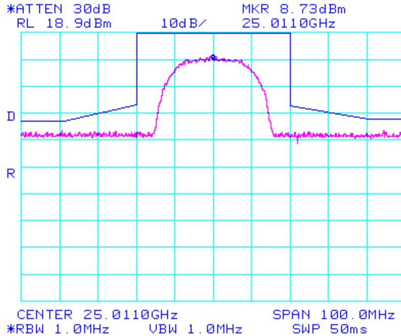
Graph 1. Emissions Limitation Test Result, QPSK
