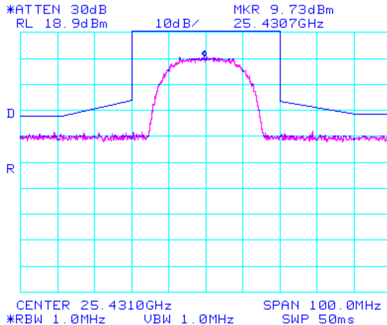
Graph 2. Emissions Limitation Test Result, QPSK
