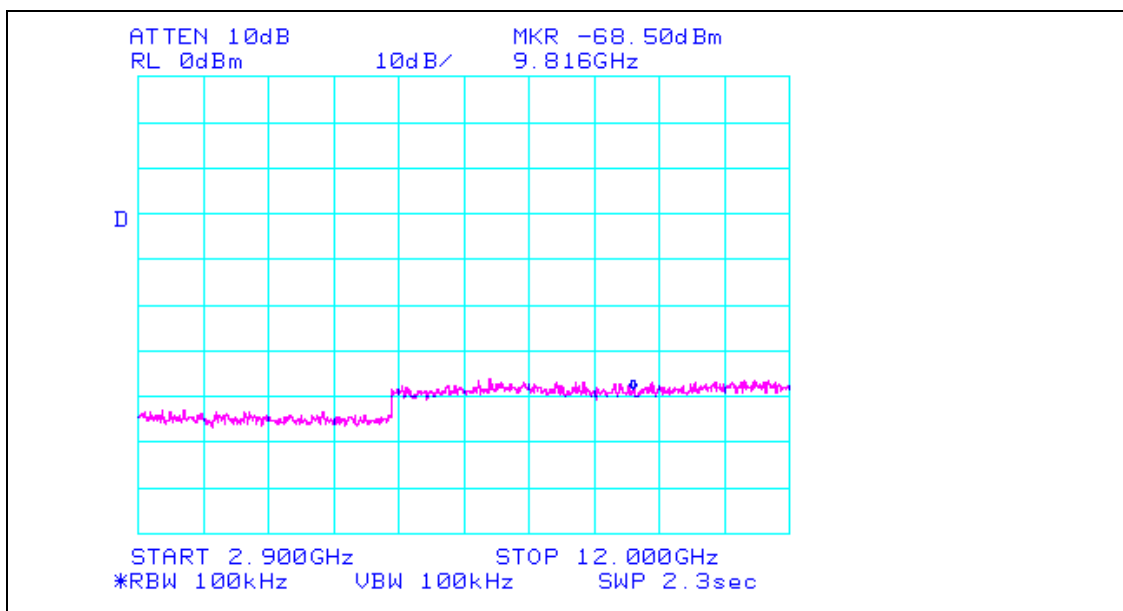
Plot 8. Conducted Spurious Emissions, Test Results (2.9GHz – 12GHz)
