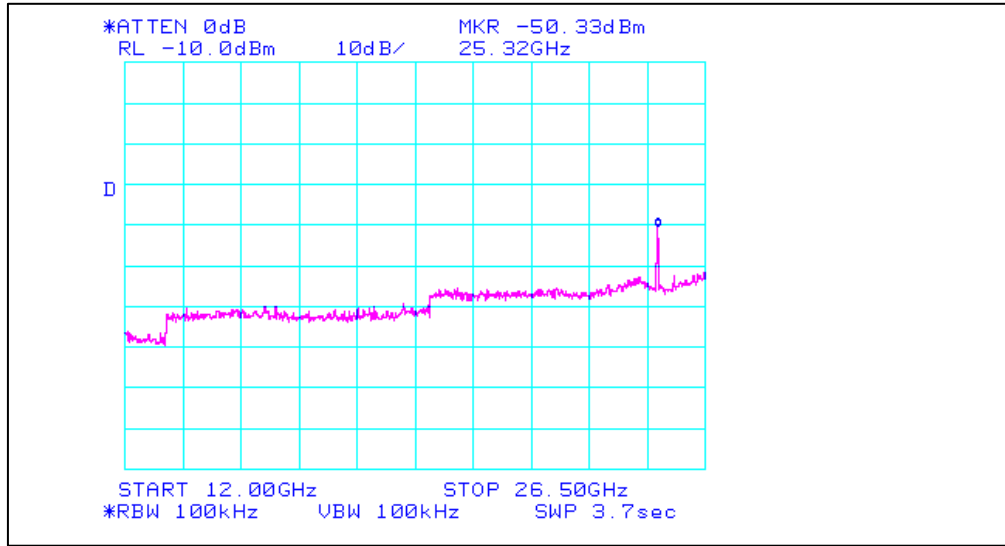
Plot 12. Radiated Spurious Emissions, Test Results (12.0 GHz - 26.5GHz)
