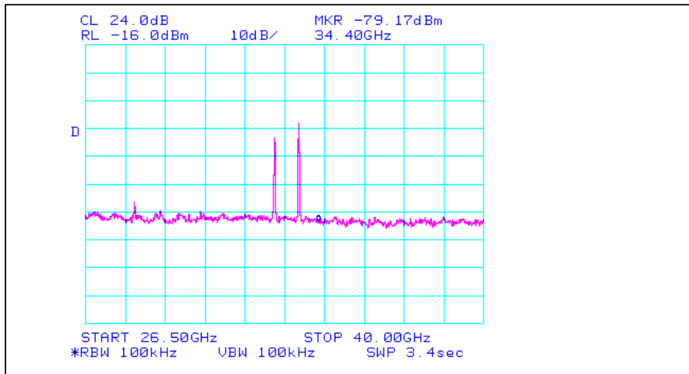
Plot 13. Radiated Spurious Emissions, Test Results (26.5GHz - 40GHz)
