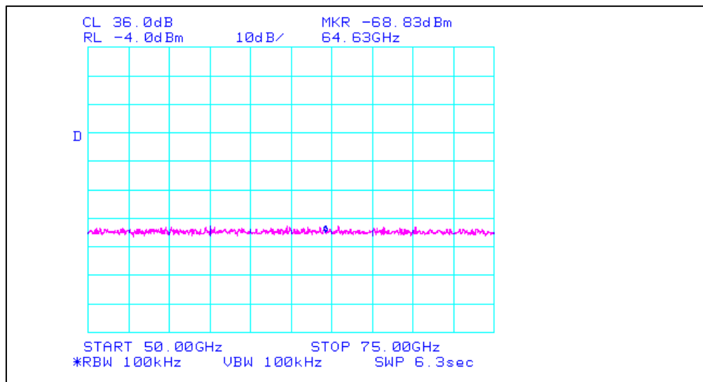
Plot 15. Radiated Spurious Emissions, Test Results (50.0GHz - 75.0GHz)
