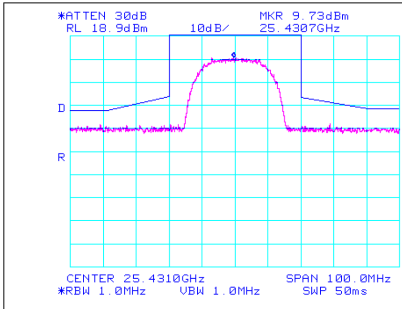
Plot 19. Emission Limitation Test Results (QPSK)
