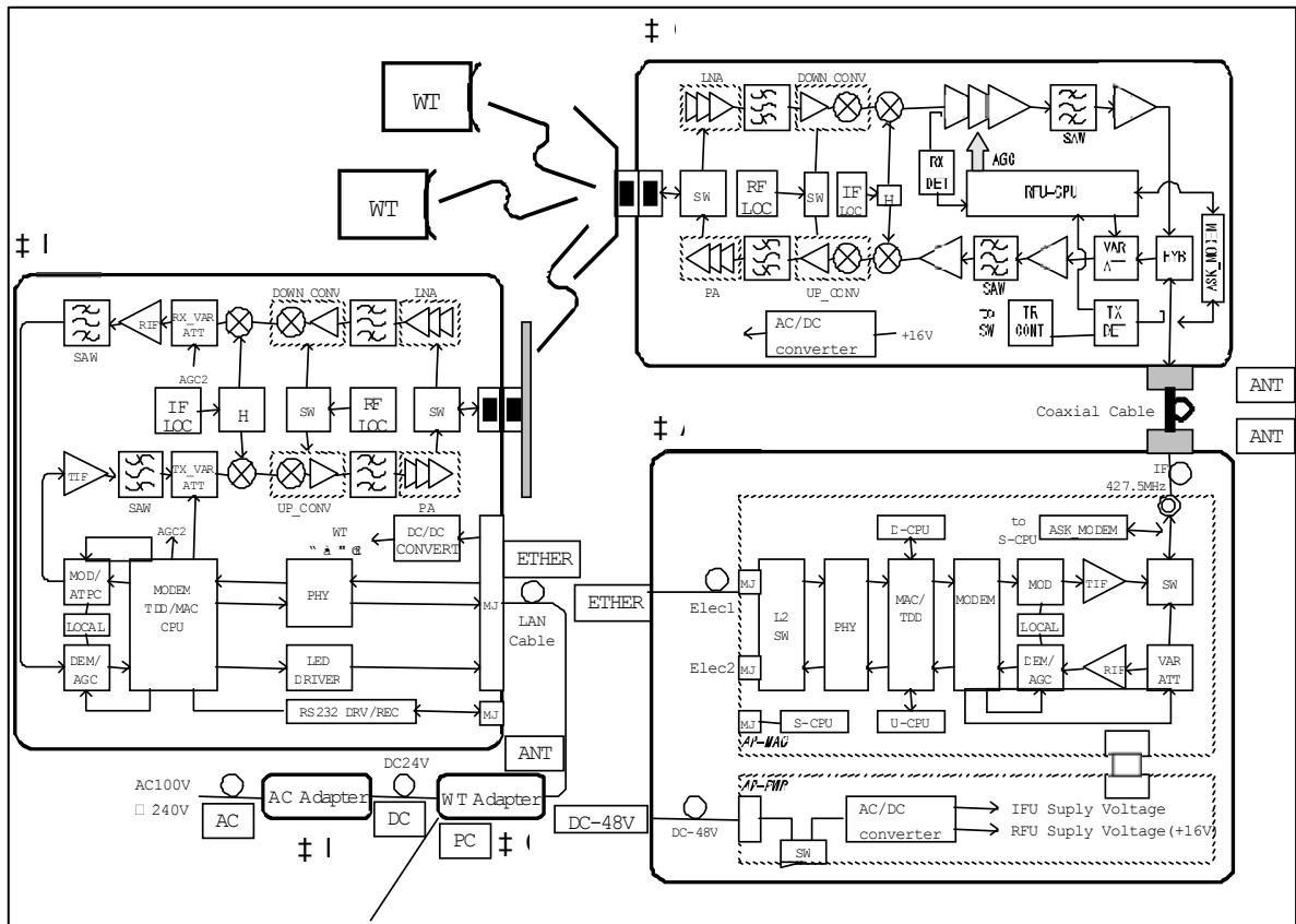
Figure 1. Block Diagram of Test Configuration
