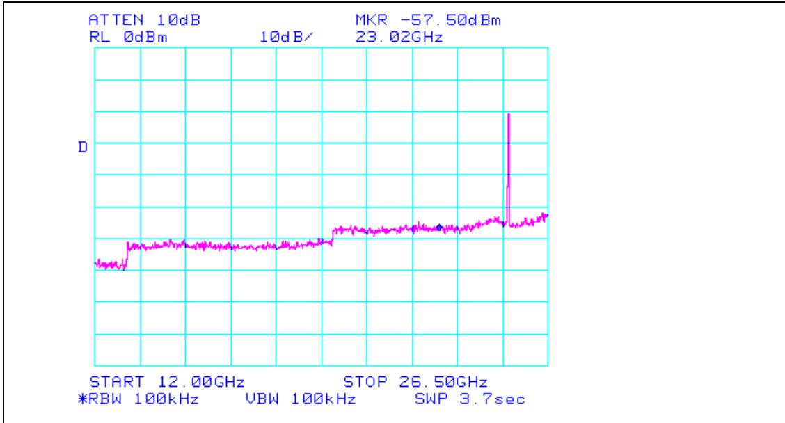
Plot 9. Conducted Spurious Emissions, Test Results (12GHz – 26.5 GHz)
