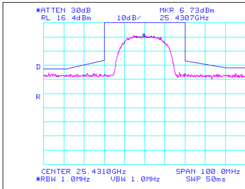
Plot 20. Emission Limitation Test Results (16QAM)
