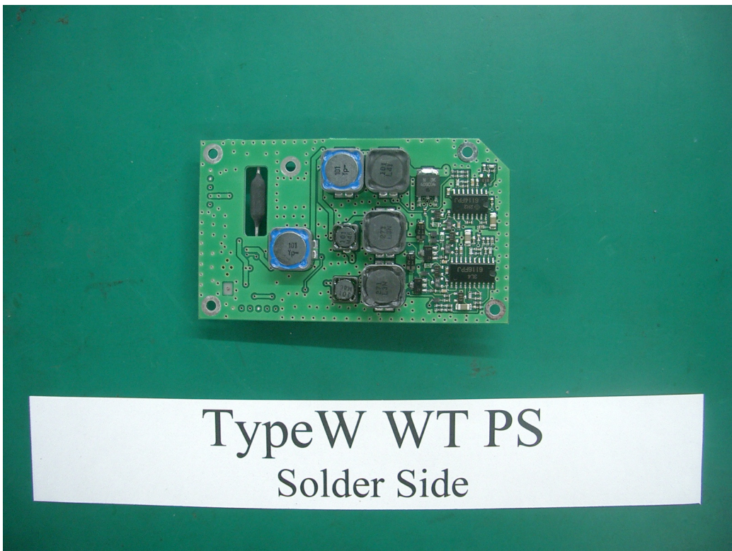
TypeW WT PS Solder Side Internal View
