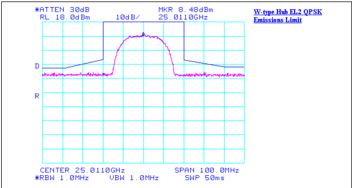
Plot 16. Emission Limitation Test Results (QPSK)
