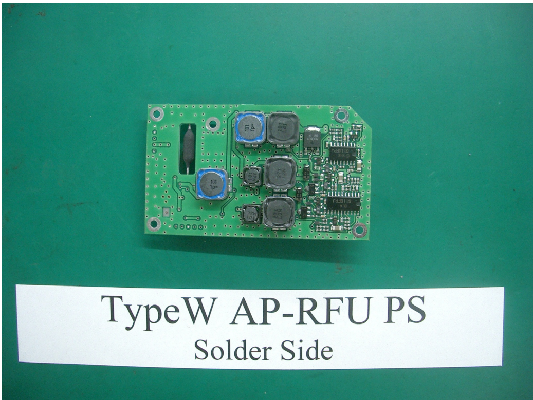
Type W AP-RFU PS Solder Side Internal View
