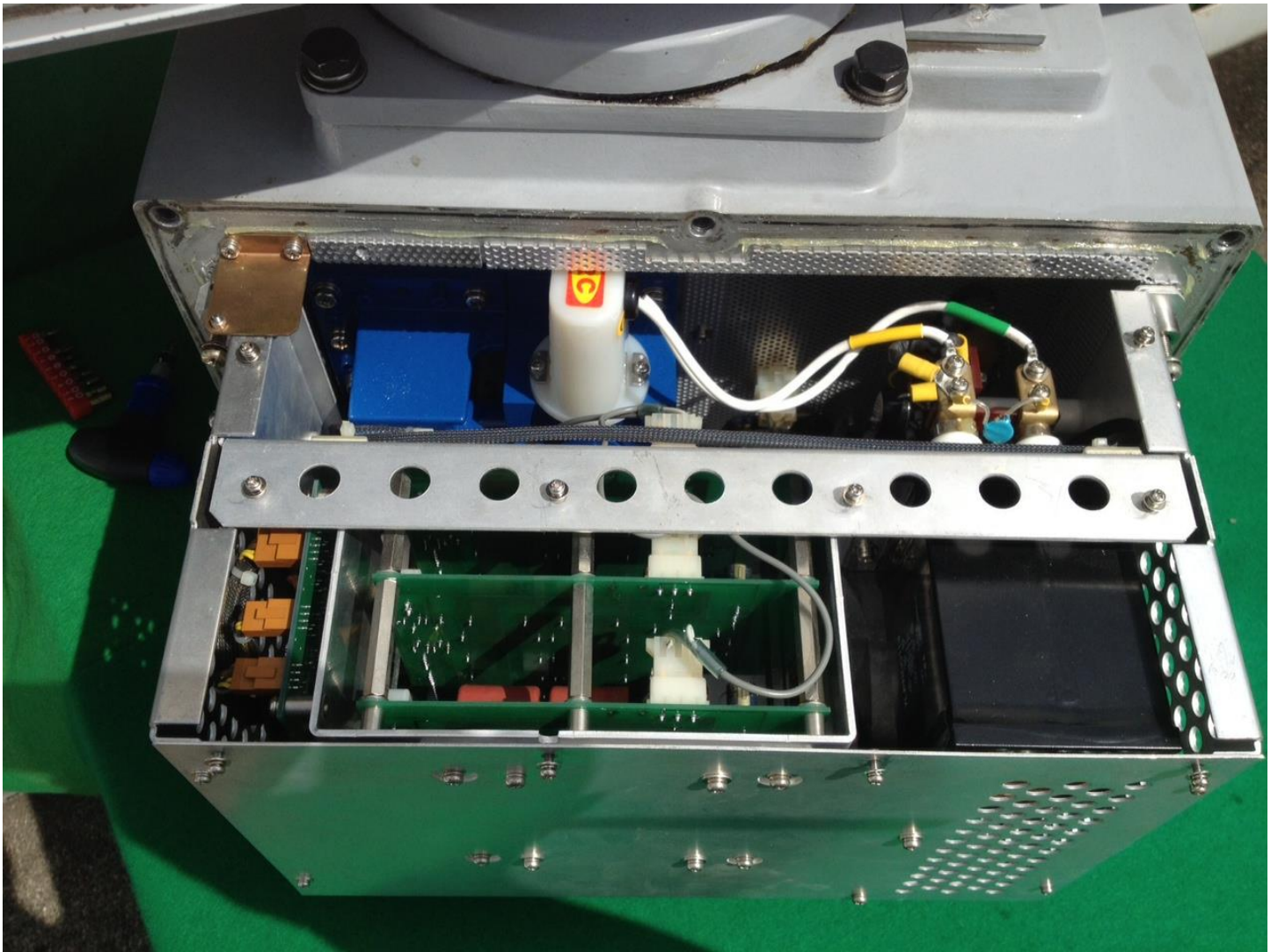
NKE-3710-8 Port Side without Cover_04
