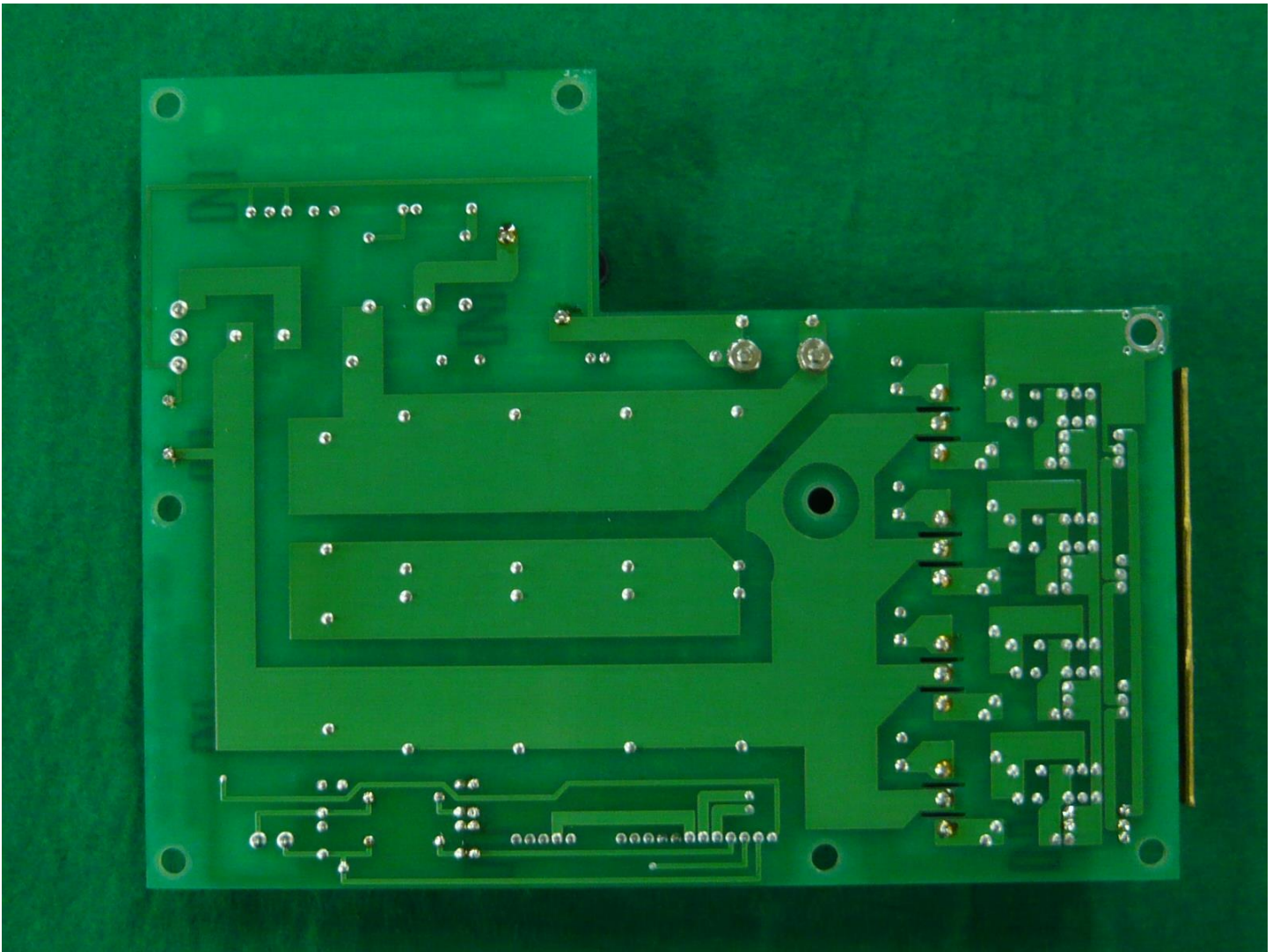
NKE-3710-CPA-209A_Solder Side
