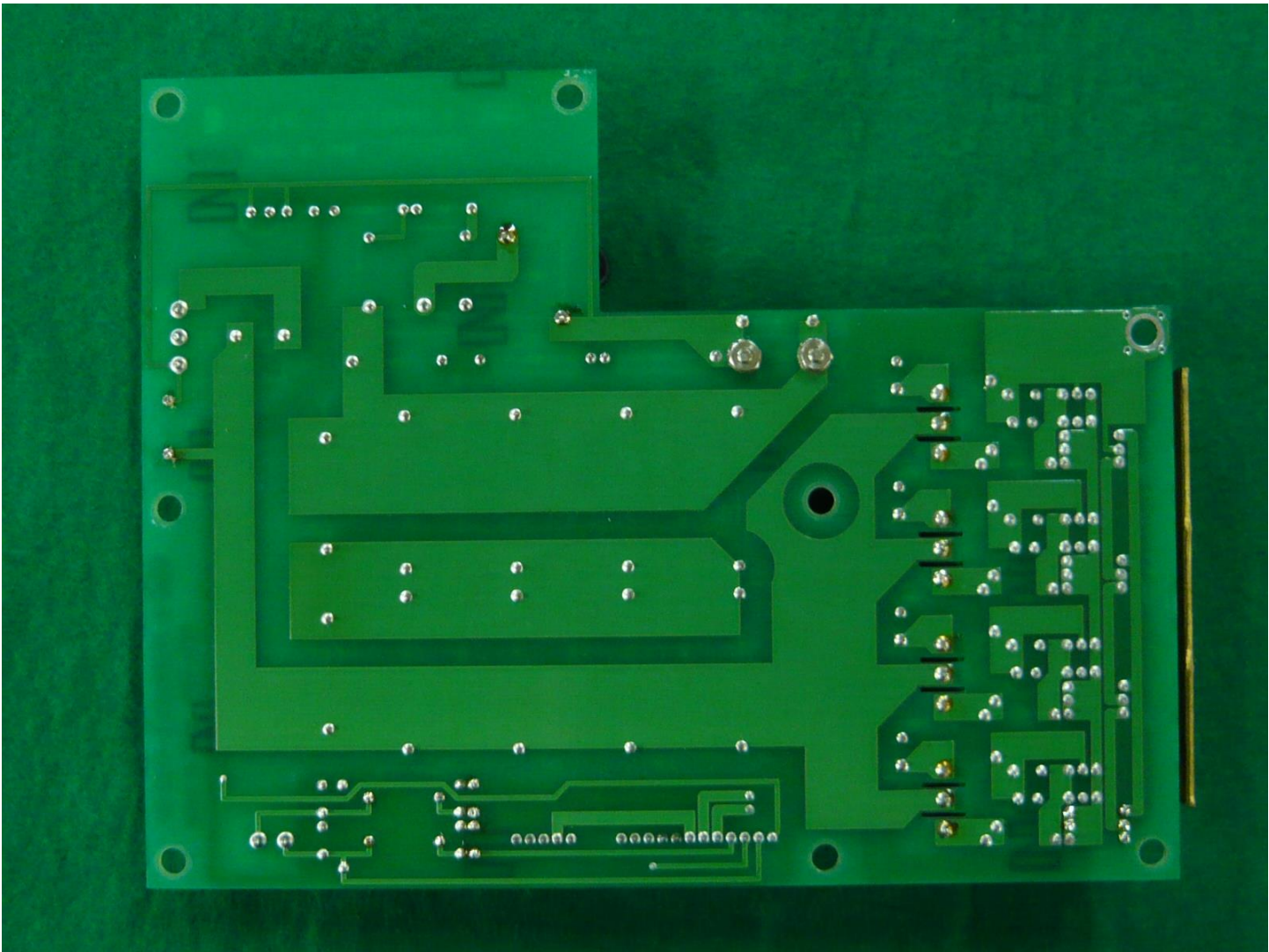
NKE-3710-CPA-209A_Component Side
