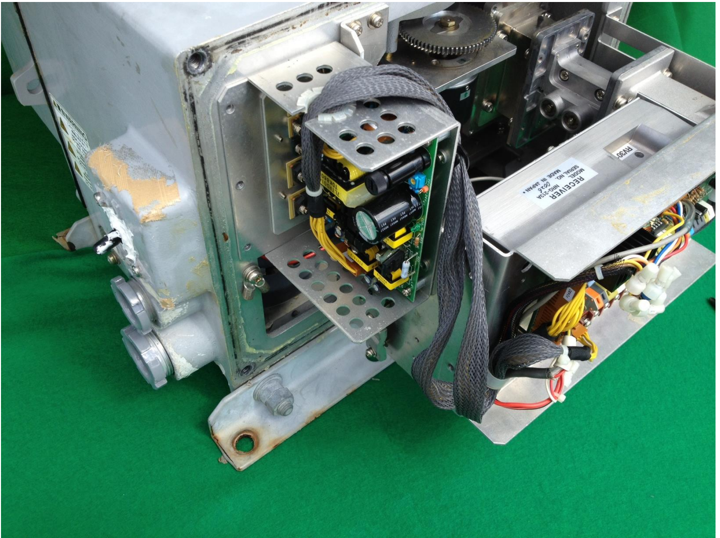
NKE-3710-8 Starboard Side without Cover_02
