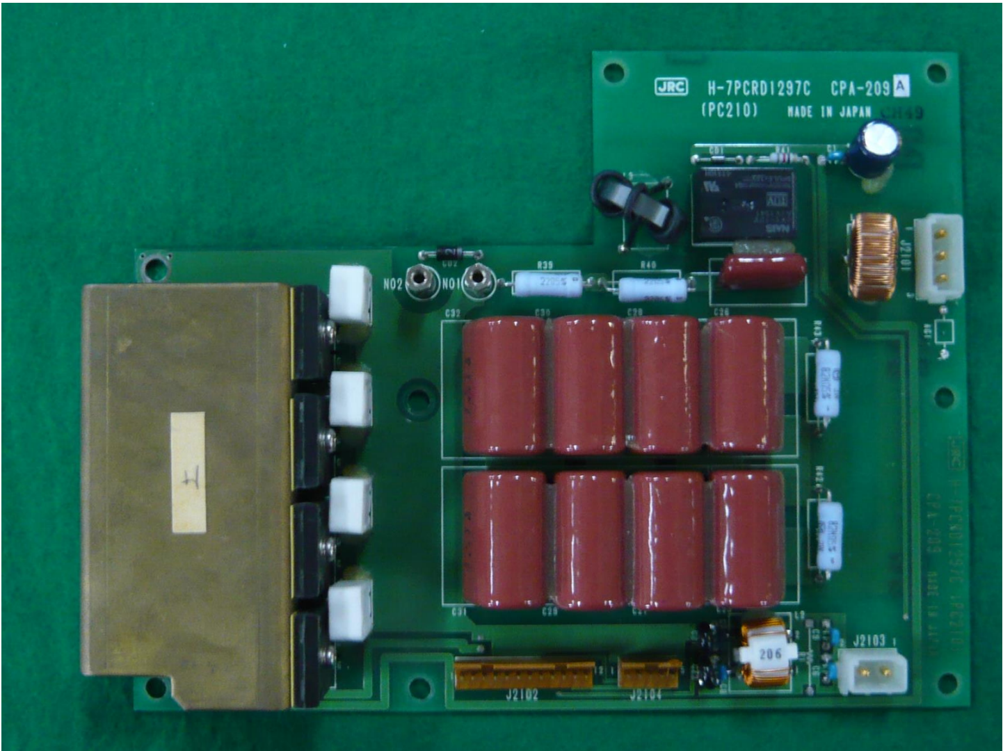
NKE-3710-CPA-209A_Component Side
