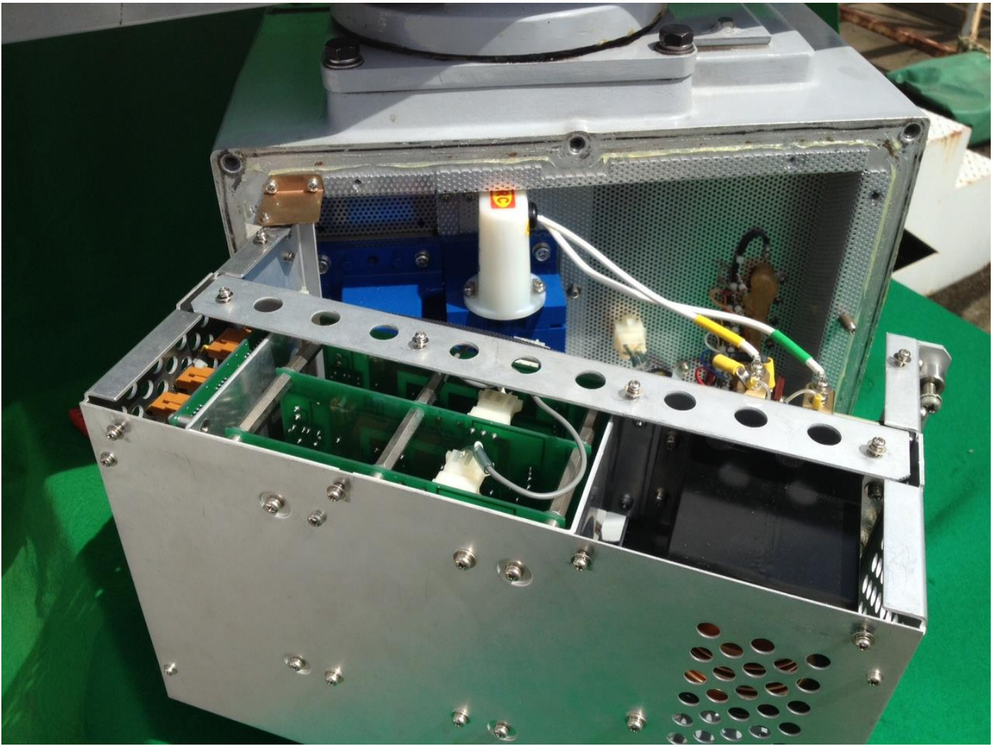
NKE-3710-8 Port Side without Cover_03
