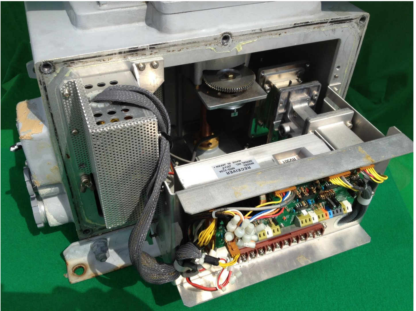
NKE-3710-8 Starboard Side without Cover_01
