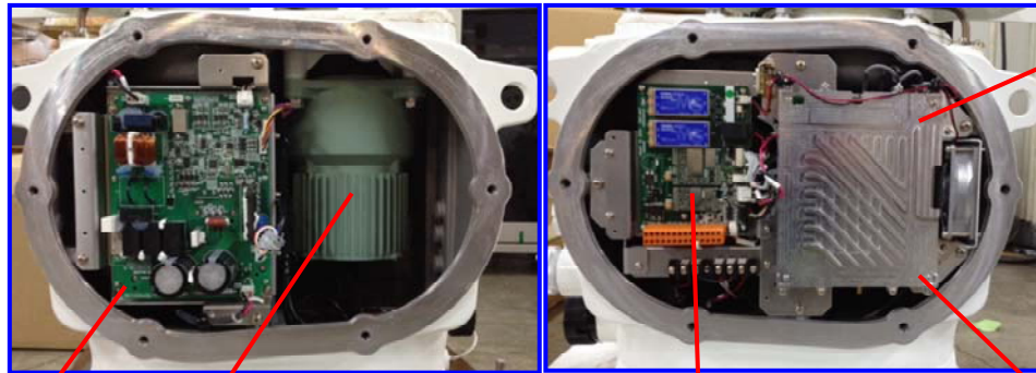
Right side
