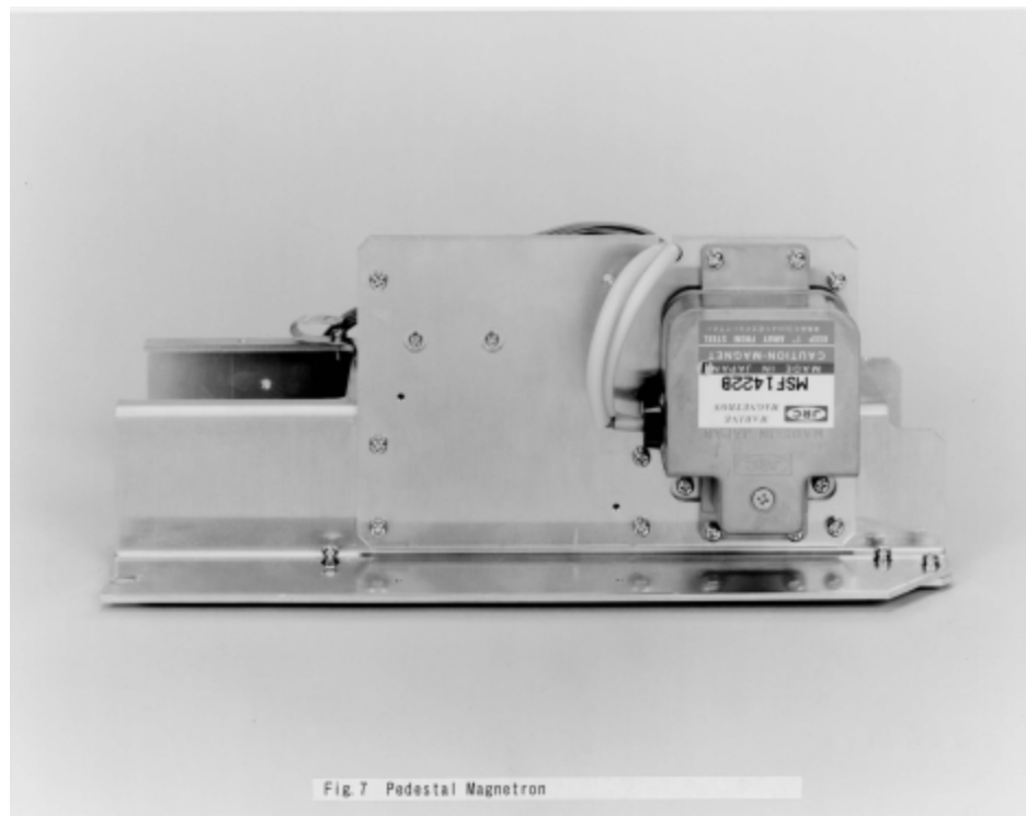
Internal Photo of Magnetron Board.
