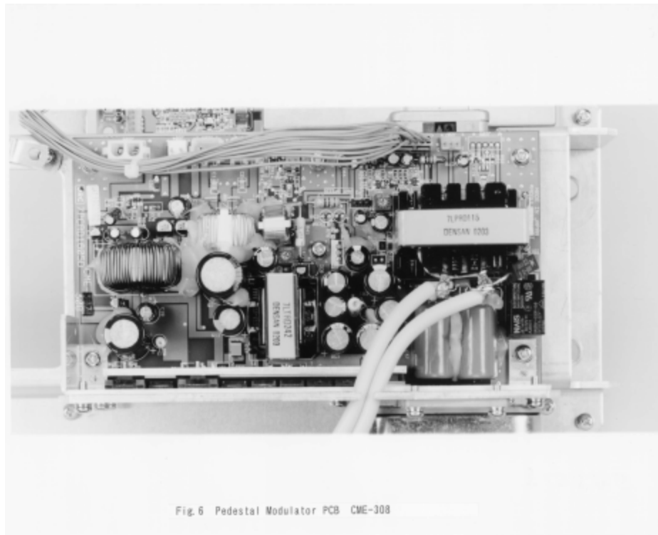
Internal photo of Modulator board.
