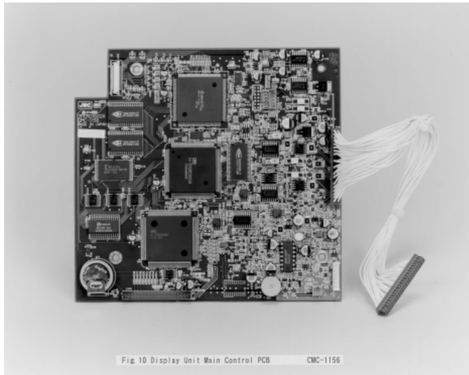
Internal Photo Main control unit in display
