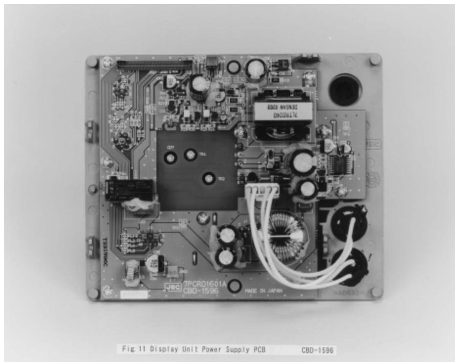
Internal photo of Power supply board in display.
