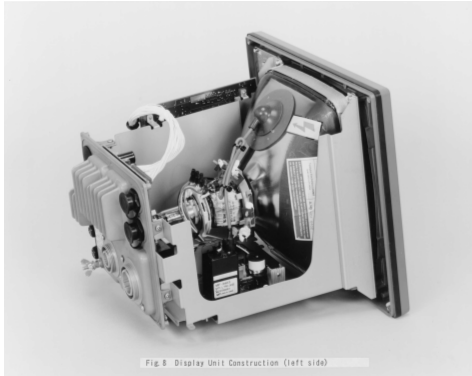
Display Internal Photo from left
