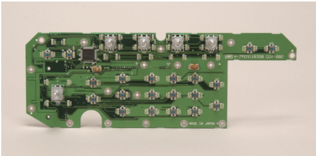
Key board front
