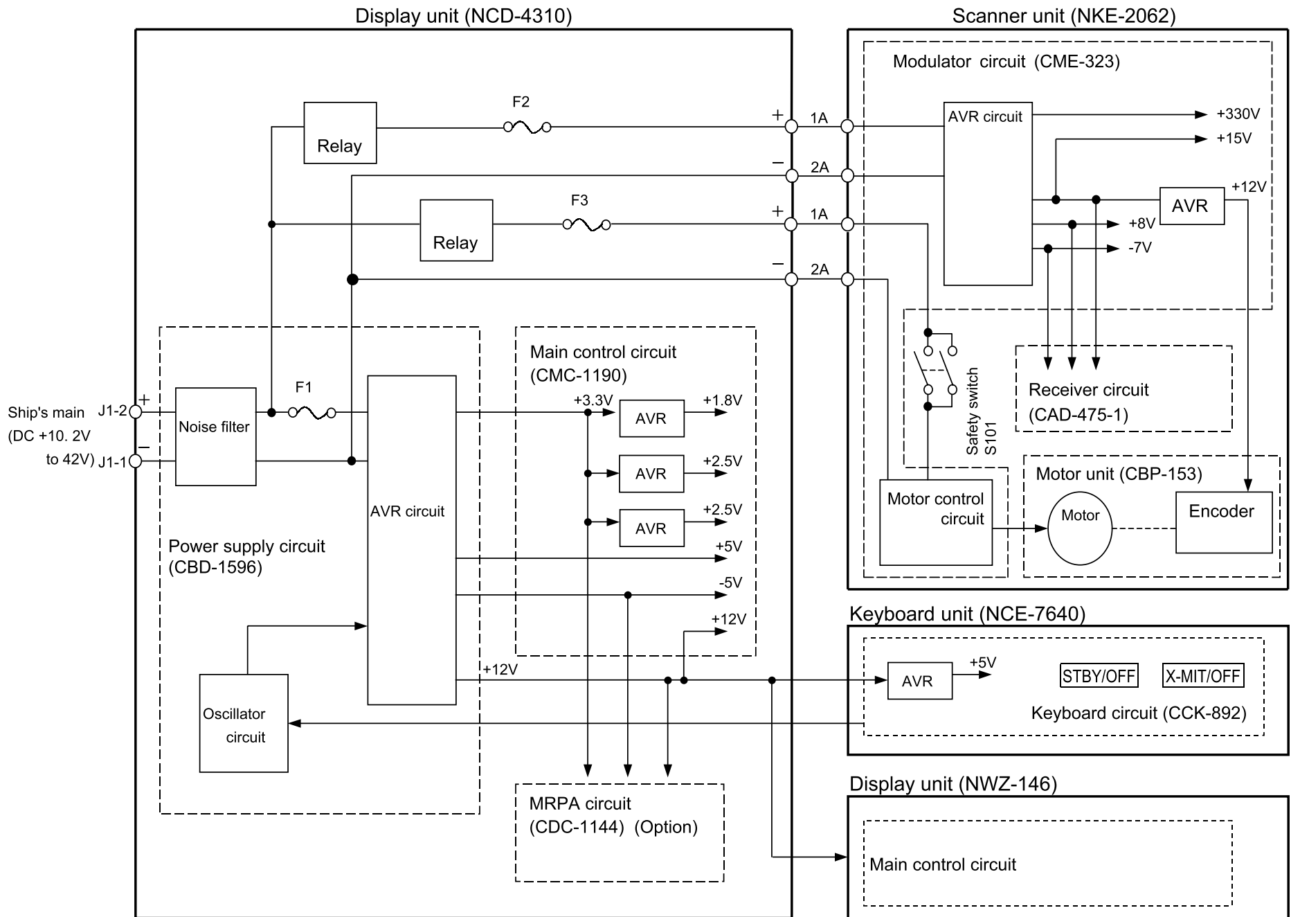
[Fig. 105 PRIMARY POWER SYSTEM DIAGRAM OF JMA-5106]
