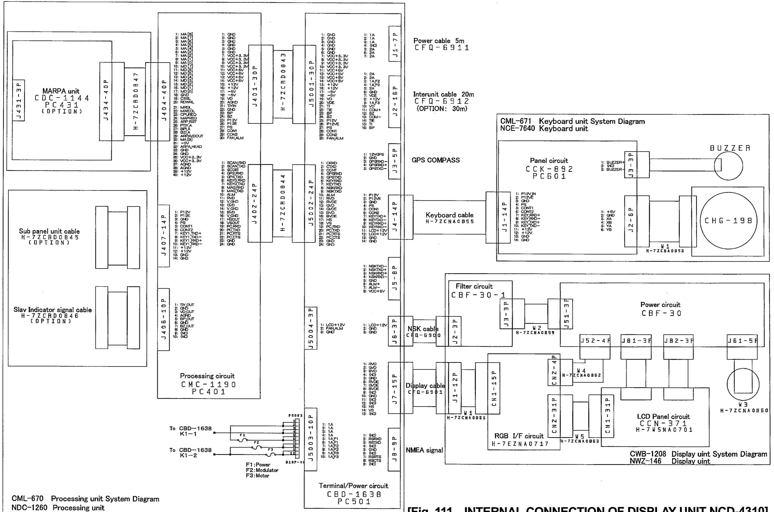
[Fig. 111 INTERNAL CONNECTION OF DISPLAY UNIT NCD-4310]
