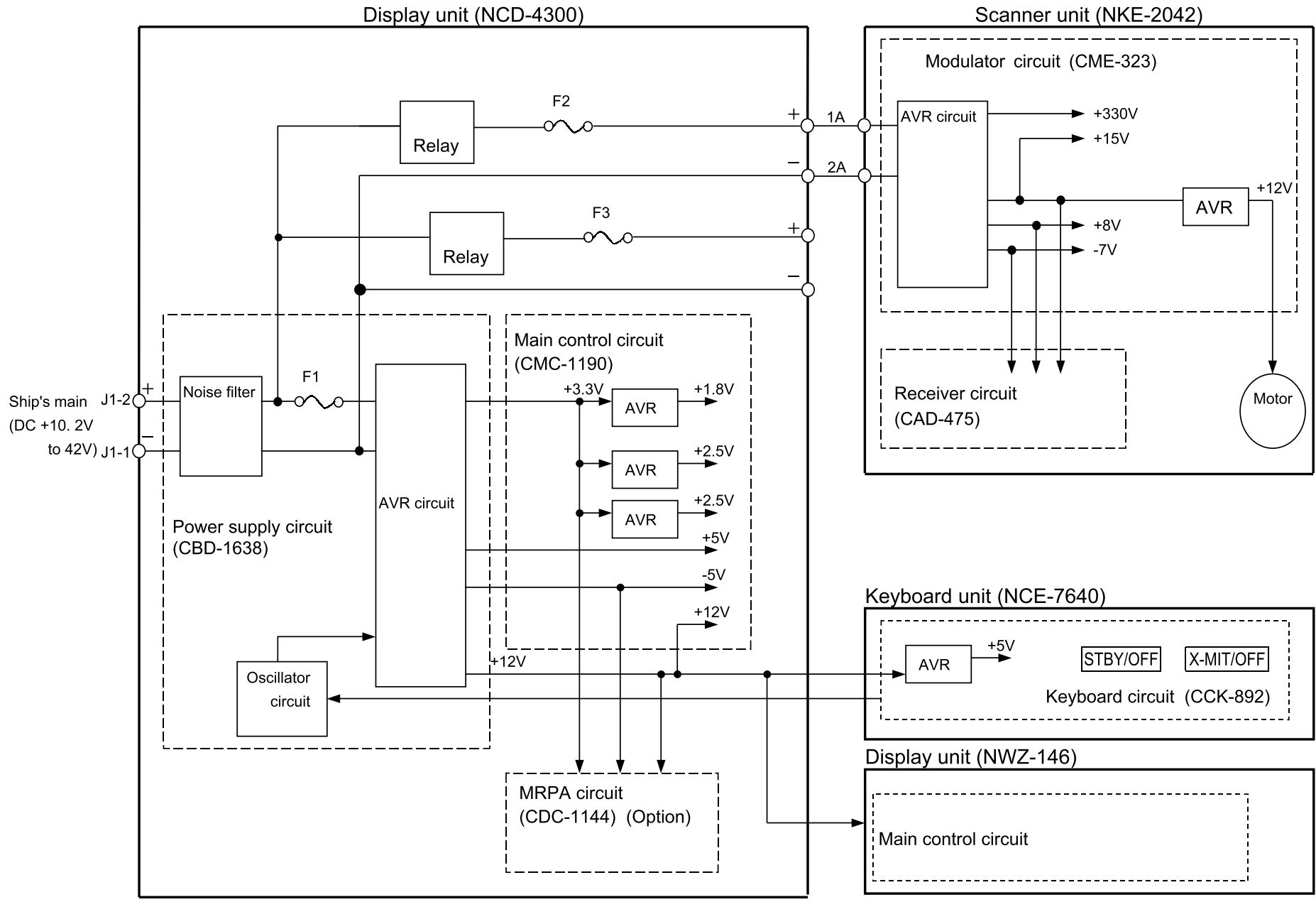
[Fig. 104. PRIMARY POWER SYSTEM DIAGRAM OF JMA-5104]
