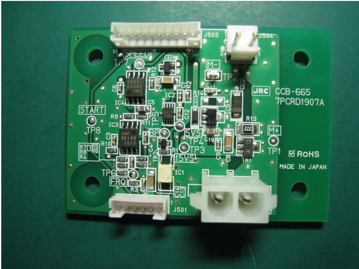
NKE2063 CCB-665 Parts Side
