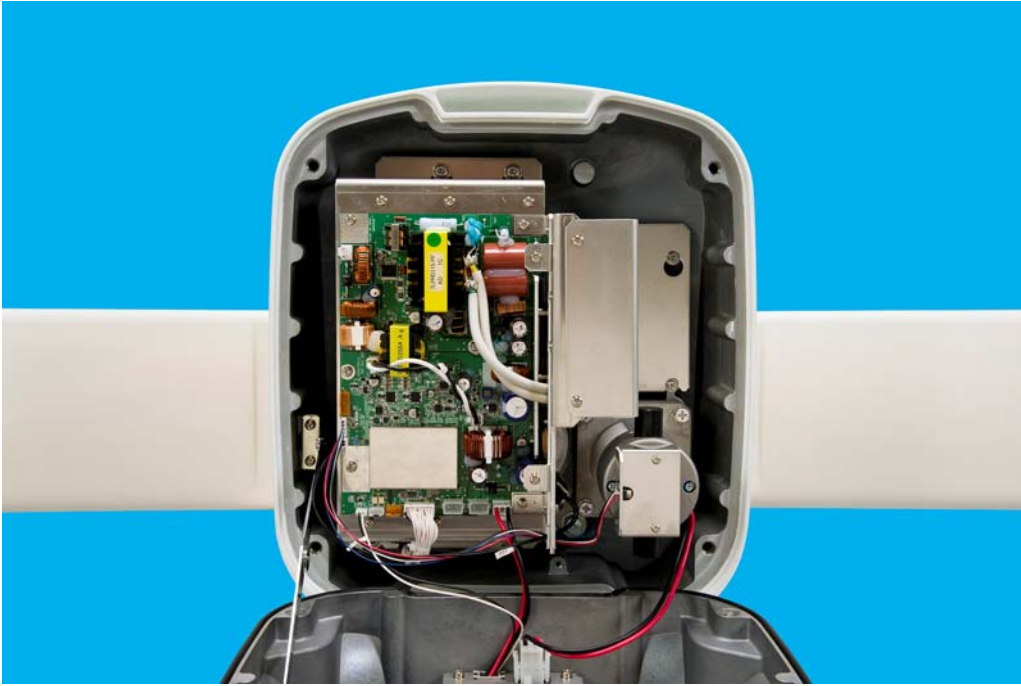
NKE2063 without cover
