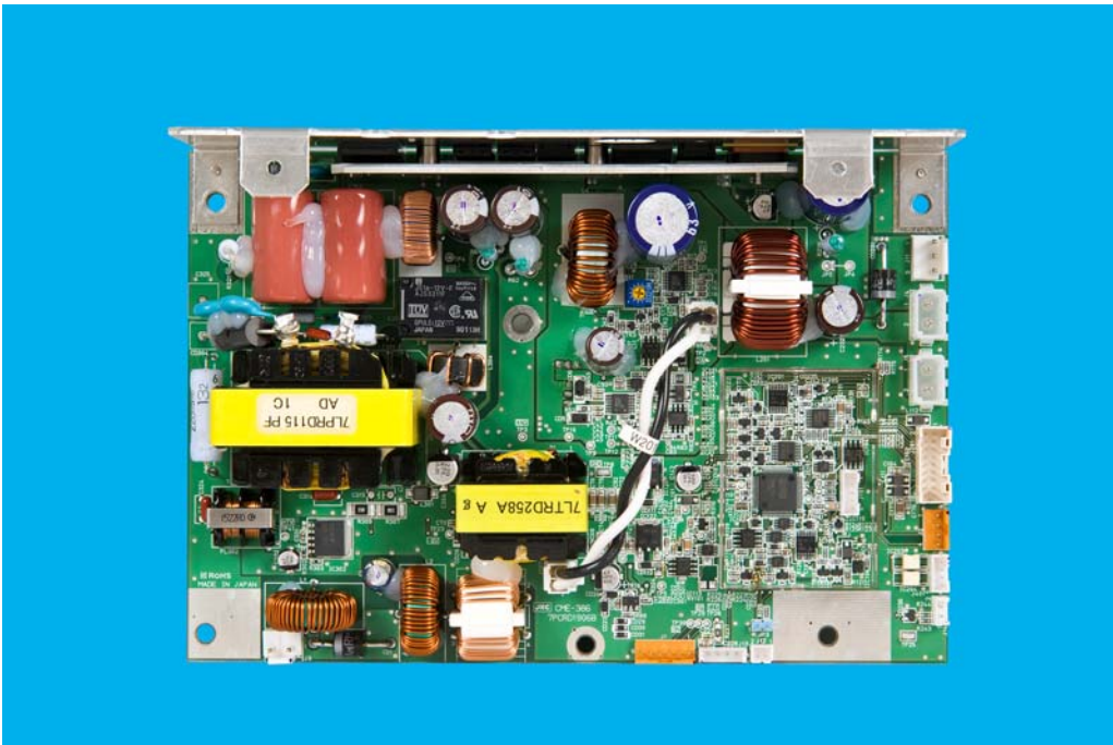
NKE2063 CME-386 Parts Side without Shield
