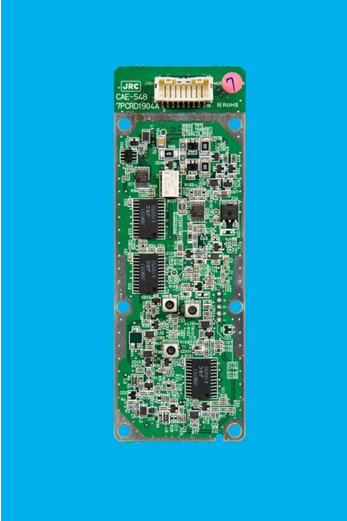
NKE2063 CAE-548 Parts Side without Shield
