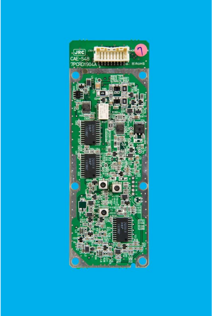
CAE-548 Parts Side without Shield
