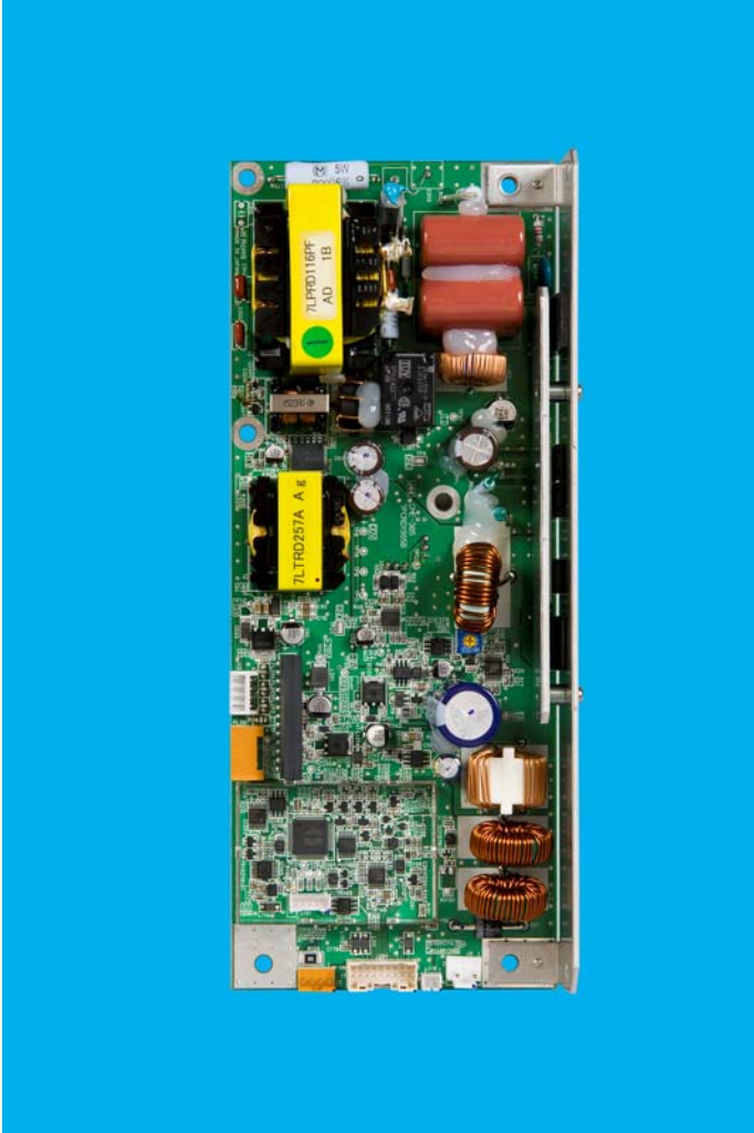
CME-385 Parts Side without Shield
