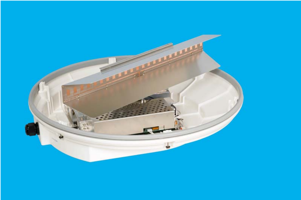
NKE2043 without Radome Starboard Side
