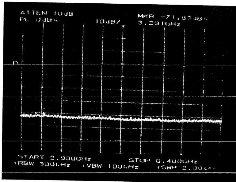
0.4 μS Pulse
