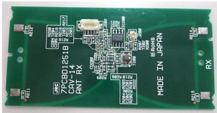
Parts side
