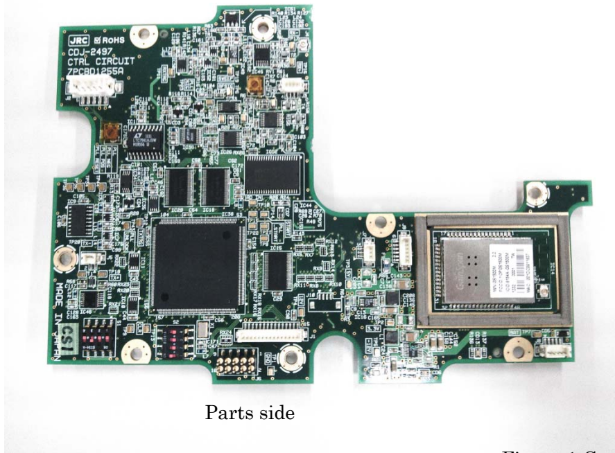
Figure 1 Control Circuit
