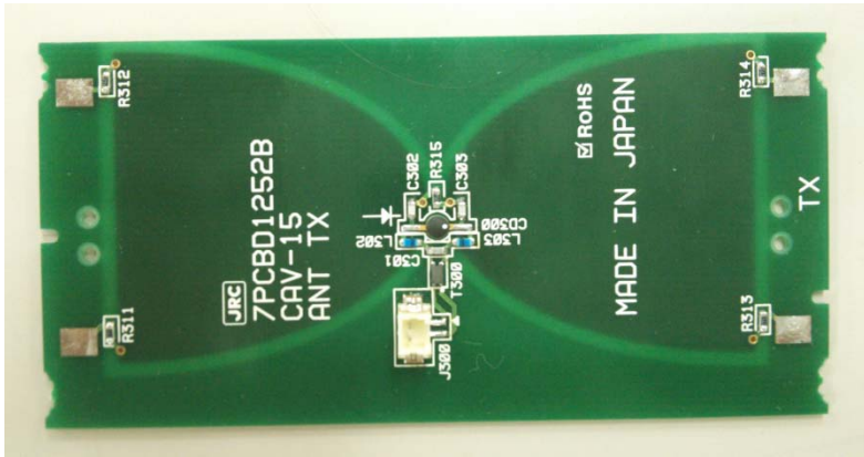
Parts side
