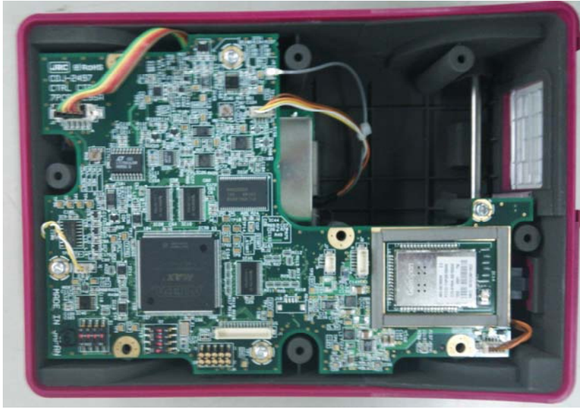
Figure 5 Control Circuit
