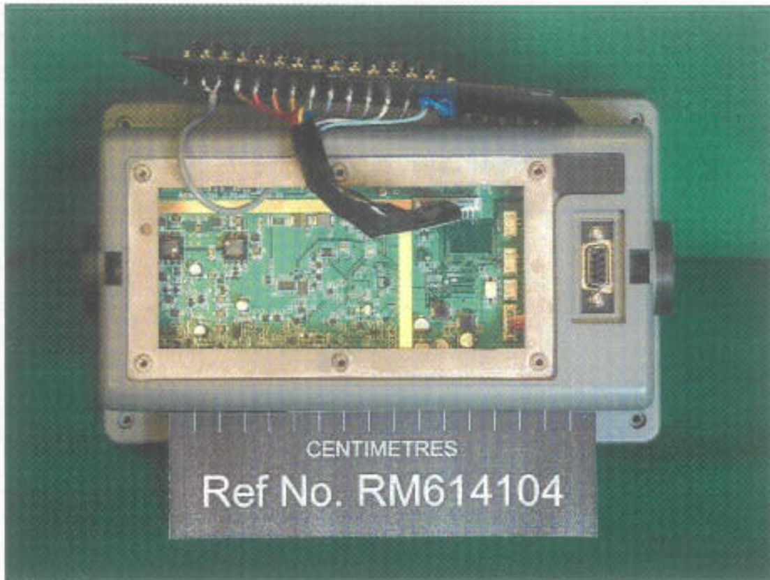
Figure 3: NCR-333 internal view
