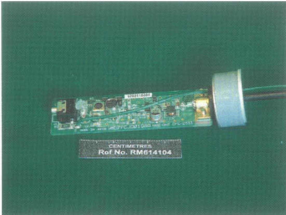
Figure 6: NAW-333 internal view
