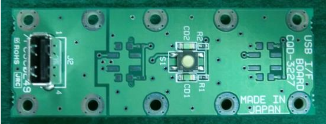
CQD-3227 USB I/F BOARD
