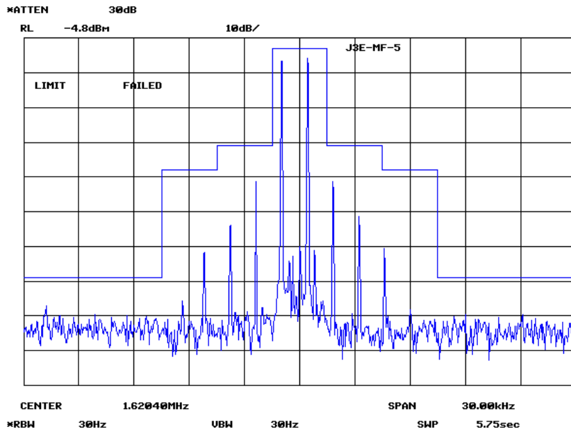
Fig. 2.3.2-1 Occupied bandwidth Frequency : 1.619 MHz Mode : J3E Line Voltage : AC220V
