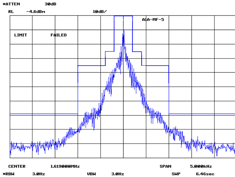
Fig. 2.3.2-2 Occupied bandwidth Frequency : 1.619 MHz Mode : A1A Line Voltage : AC220V
