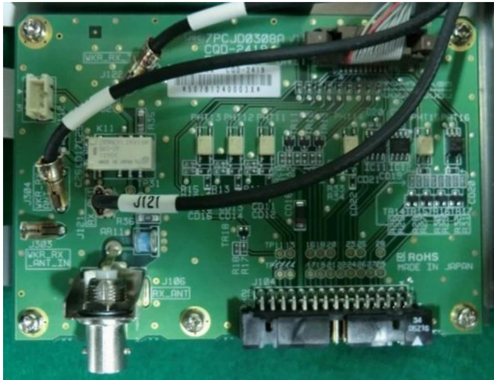
(5) CQD-2419 EXTERNAL UNIT [NTD-2250 TRANSCEIVER]
